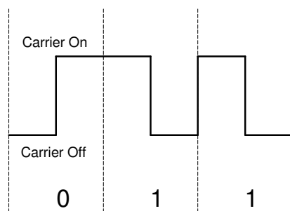
Manchester ASK Coding
