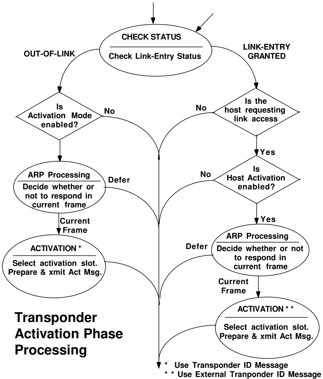
Figure 5-3b: Transponder Activation Phase Processing
