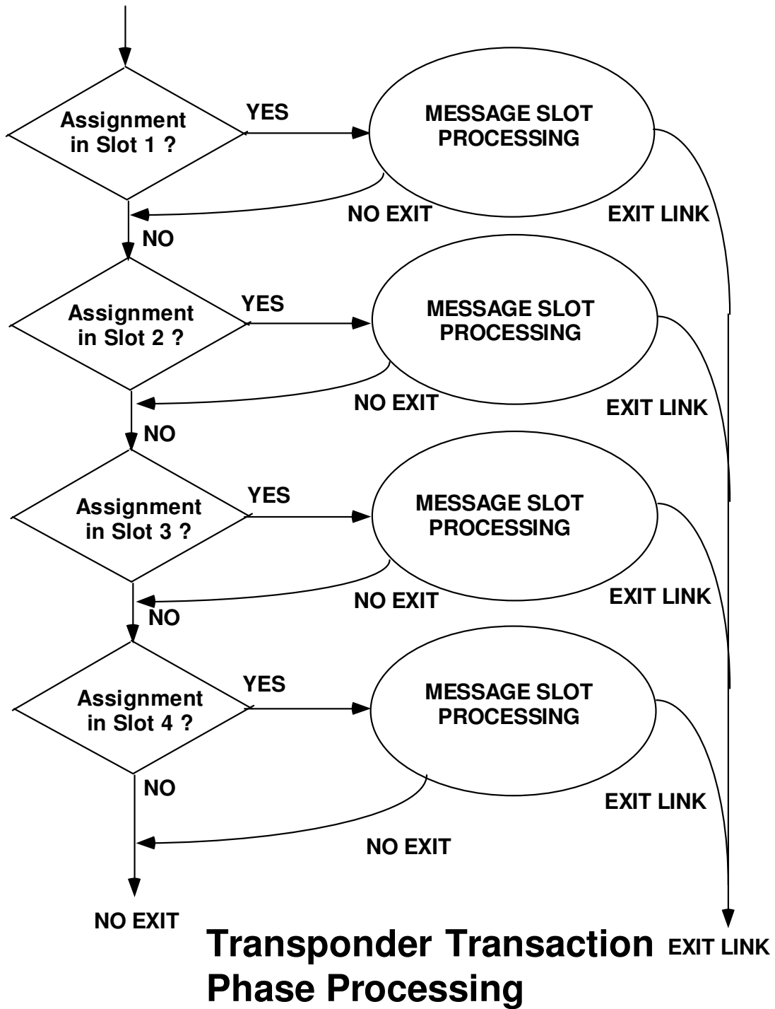
Figure 5-3c: Transaction Phase Processing
