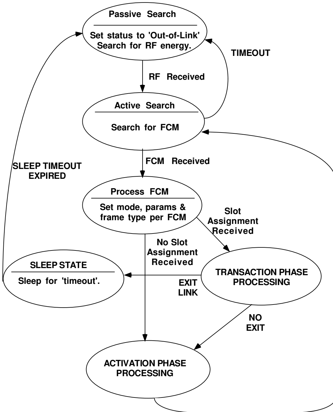
Transponder VRC Link Protocol Flow
