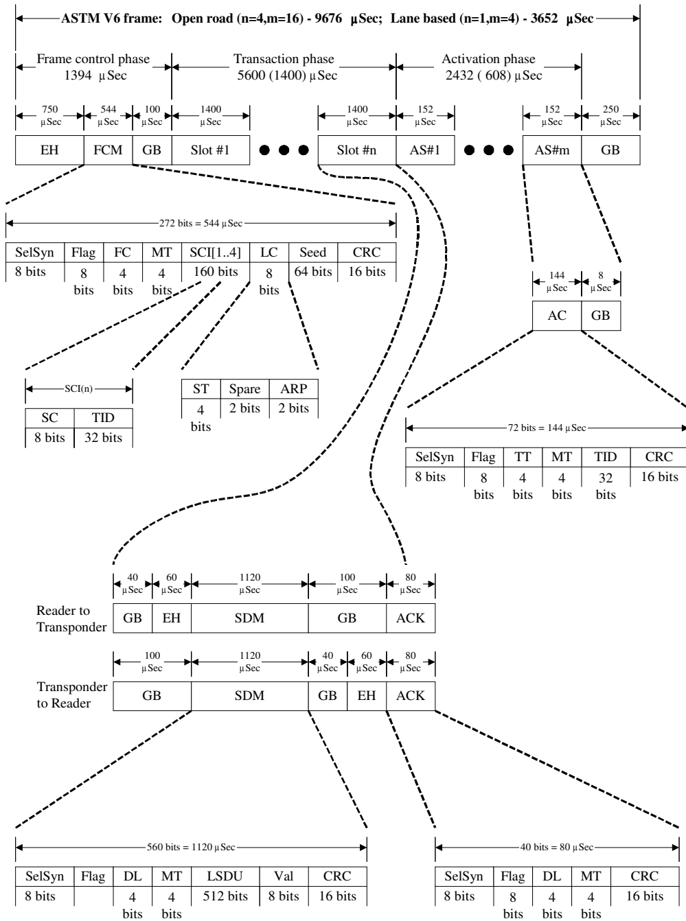
Figure 5-1: Frame Structure and Timing
