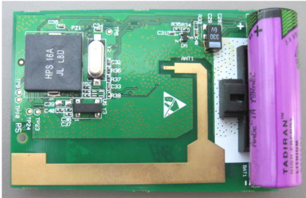
Photograph No.5 Mobile transponder PCB second side view
