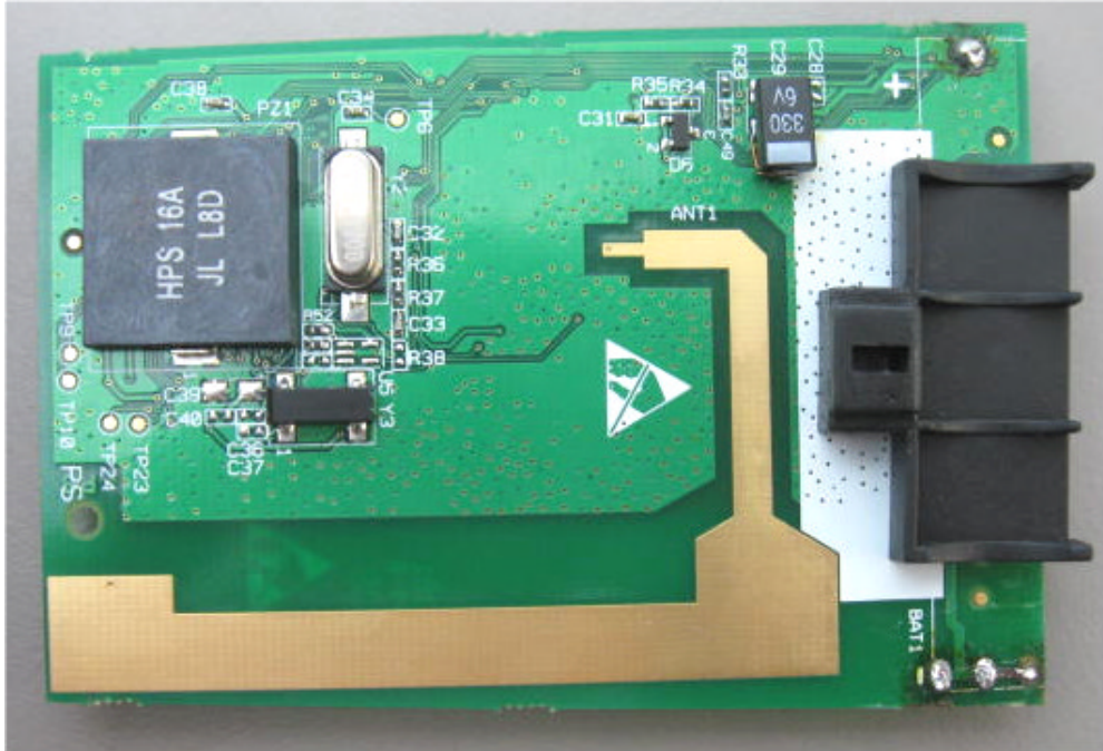
Photograph No.6 Mobile transponder PCB second side view without battery
