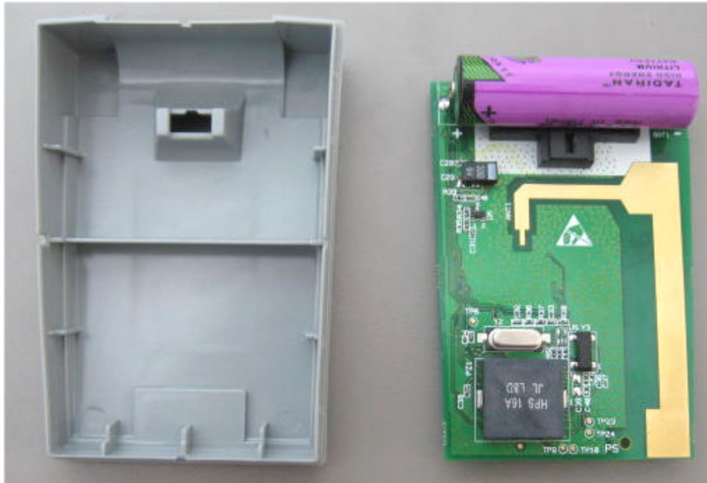
Photograph No.3 Mobile transponder FP101TB internal view, second side
