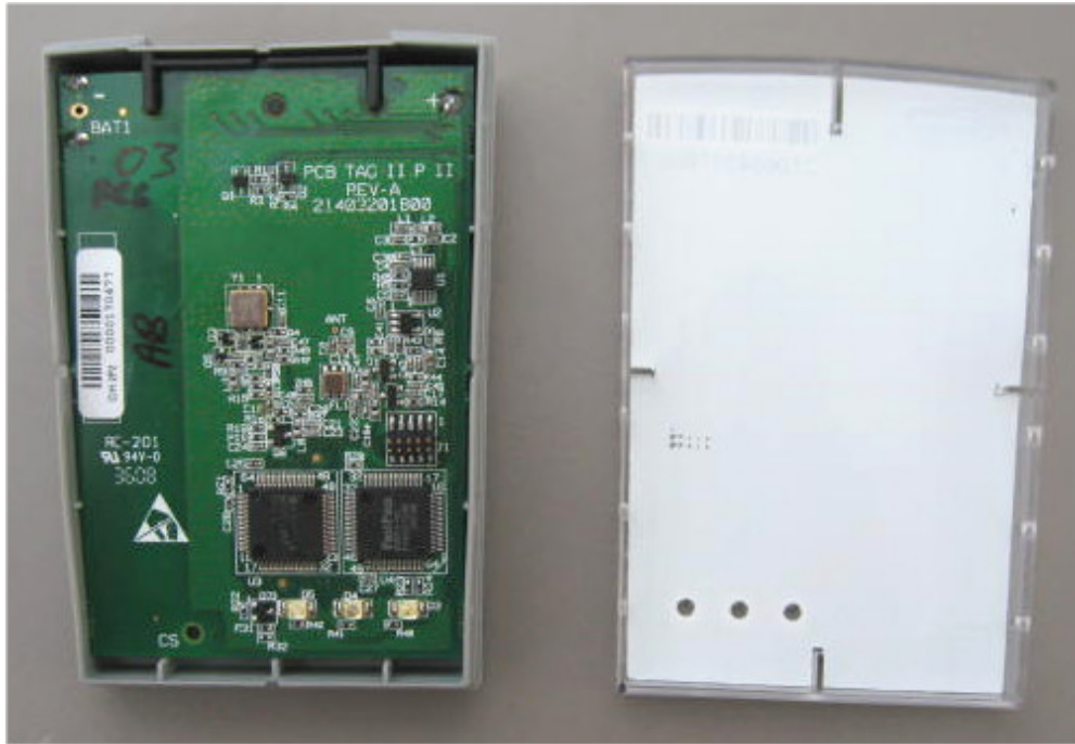
Photograph No.1 Mobile transponder FP101TB internal view
