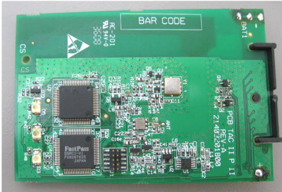
Photograph No.4 Mobile transponder PCB front view
