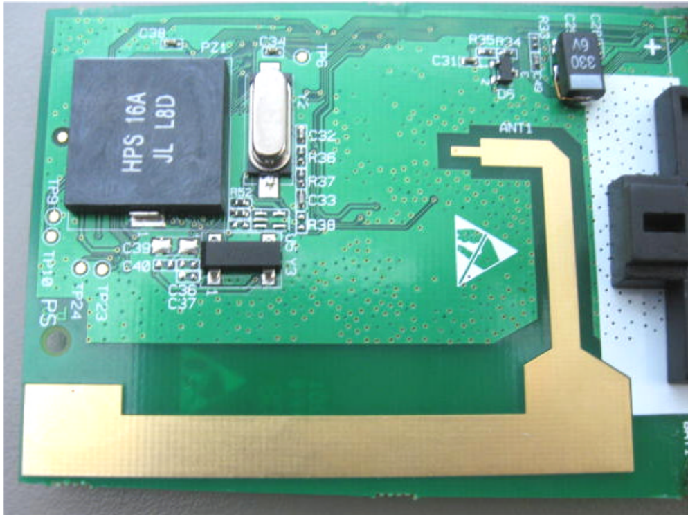
Photograph No.7 Mobile transponder antenna close view
