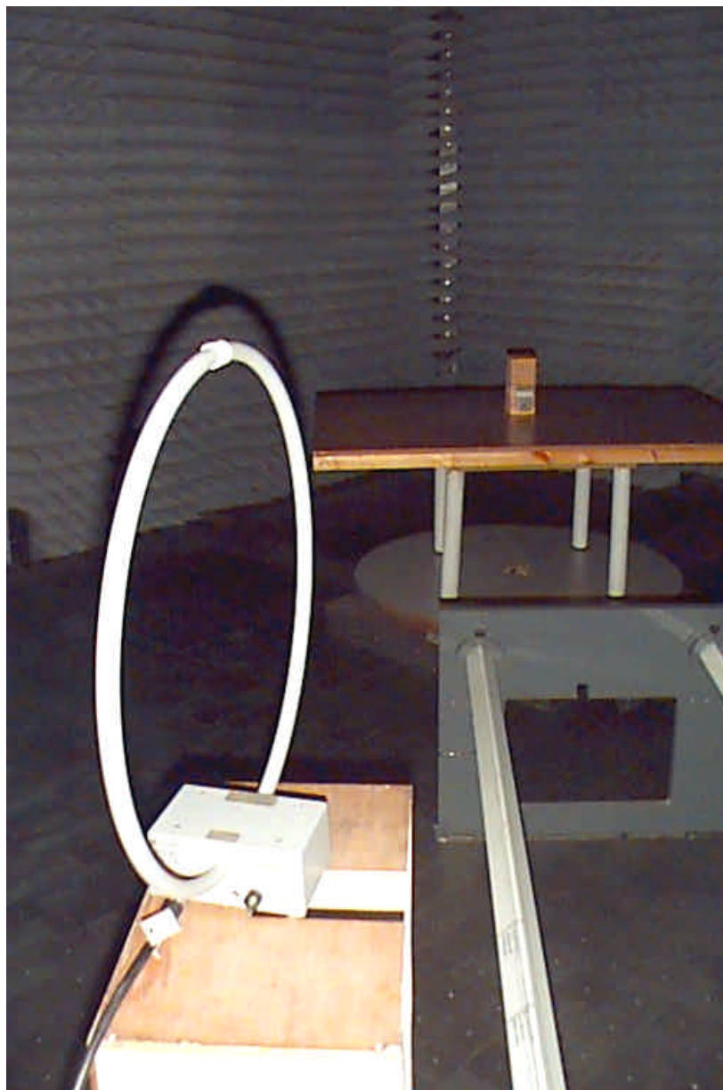
Photograph No.3 Radiated emissions measurement setup in the anechoic chamber with loop antenna
