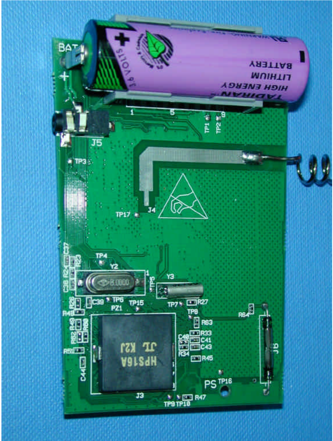
Photograph No.3 FP100SA 915 electronic seal PCB second side view
