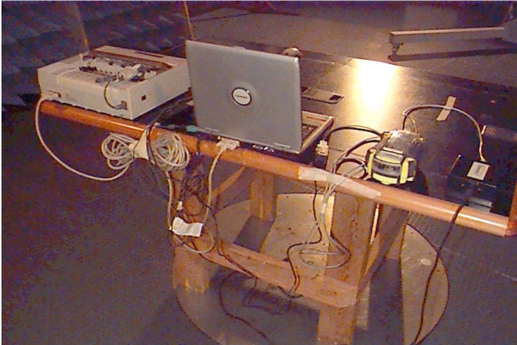
Photograph No.5 EUT configuration
