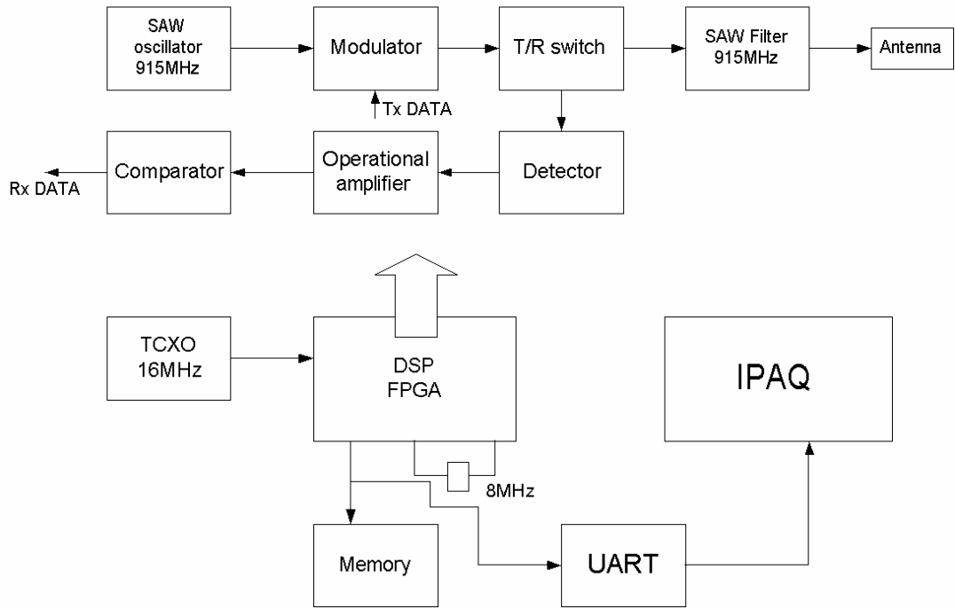
Block diagram of FP100HH
