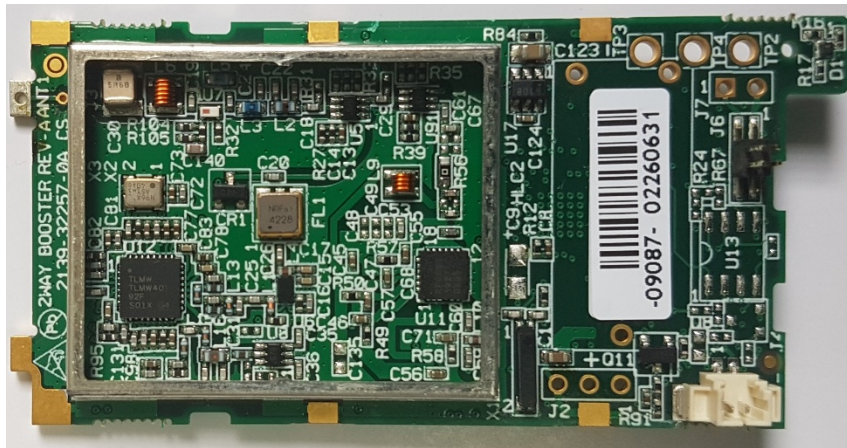
RF card - top view without shield
