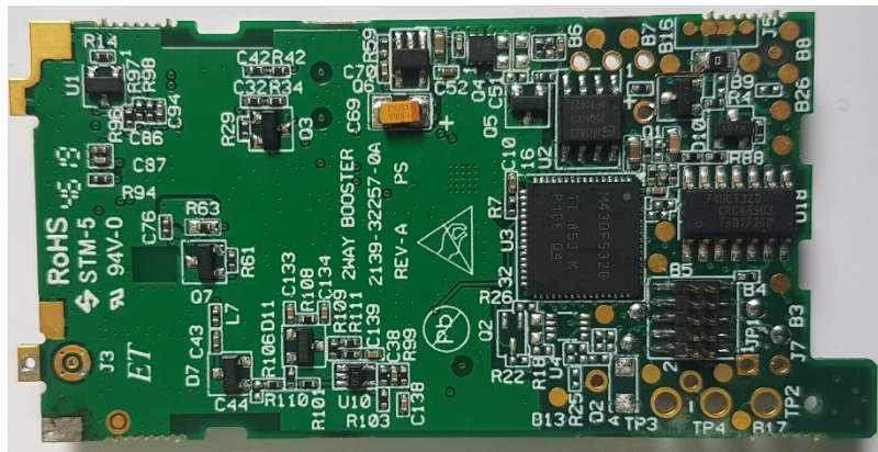
RF card - bottom view
