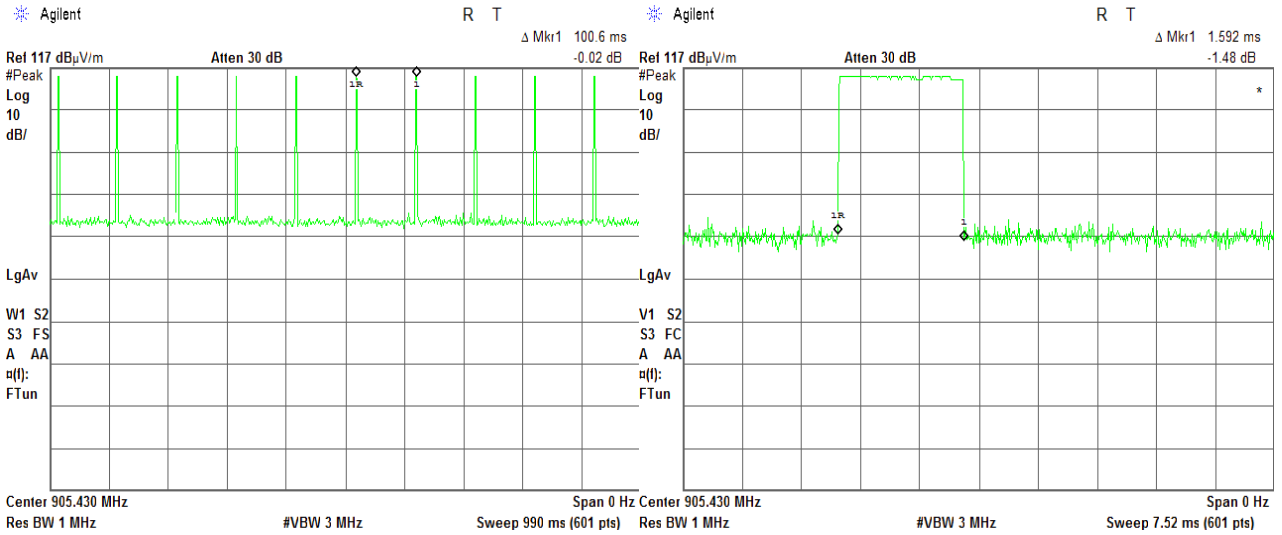
Plot 7.2.5 Pulse duration and period measurements for duty cycle calculation, BPSK modulation
