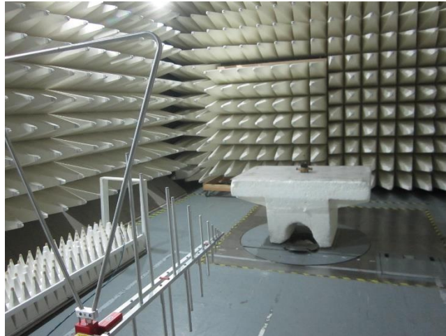
Photograph No.3 Setup for spurious emission measurements in the anechoic chamber above 30 MHz
