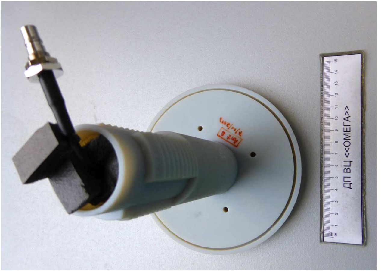
Figure 4 – Antenna.
