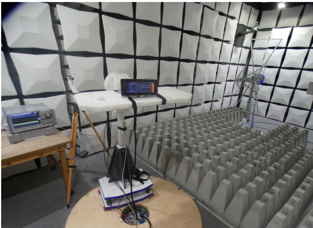
Photo 4: Test setup for radiated measurements (26 GHz - 40 GHz)
