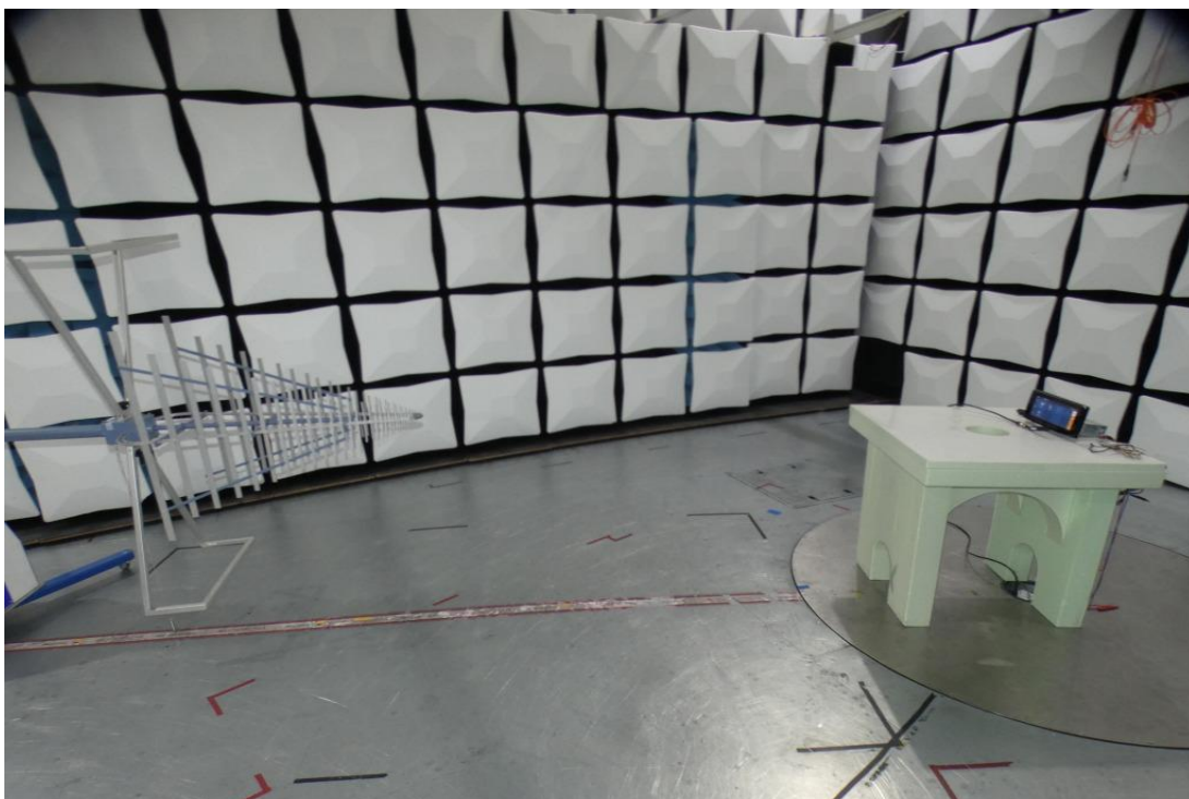
Photo 2: Test setup for radiated measurements (30 MHz - 1 GHz)
