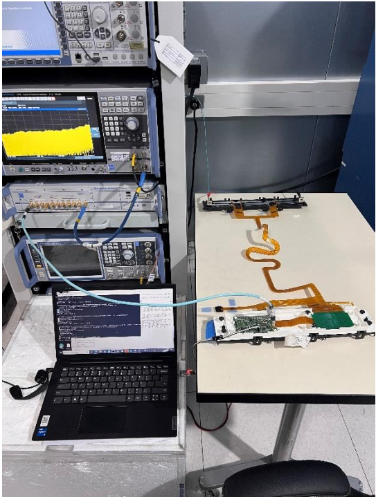
Figure B4. Conducted setup
