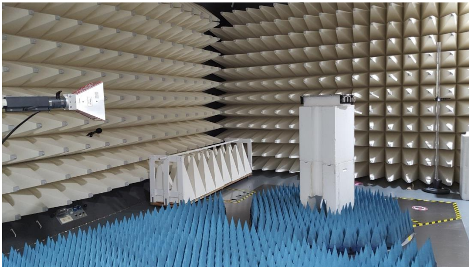
Figure B6. Radiated emission Setup – High Range 1 to 18 GHz (DUT orientation X)
