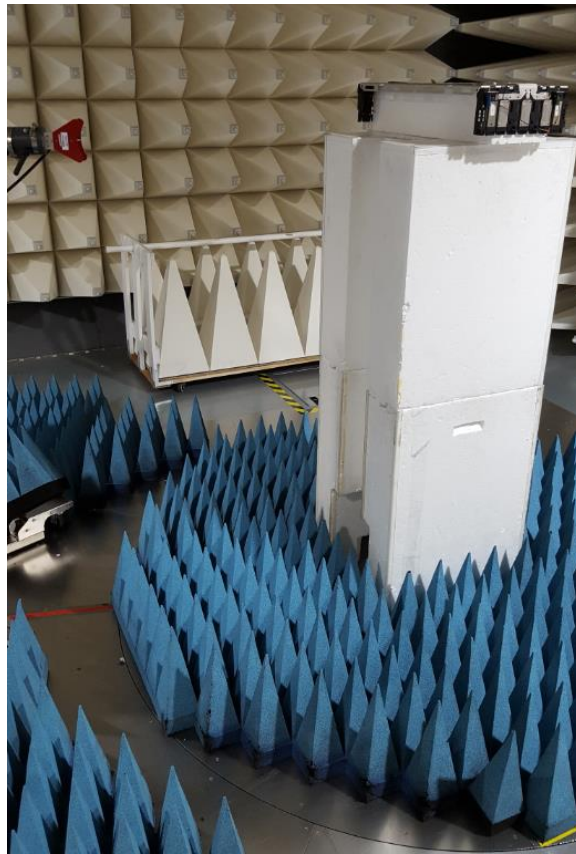
Figure B7. Radiated emission Setup – High Range 18 to 26 GHz (DUT orientation X)
