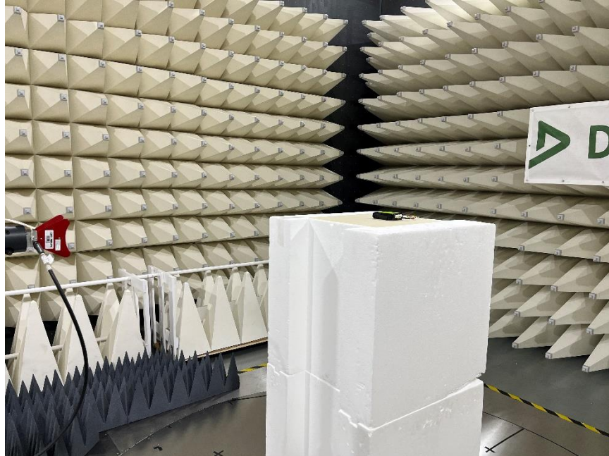
9. Radiated emission Setup 3
