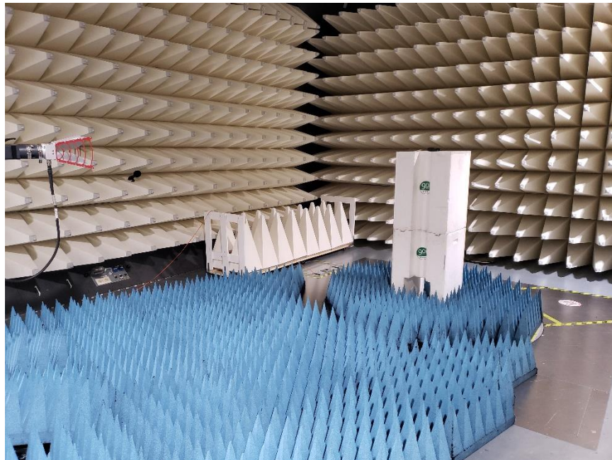
8. Radiated emission Setup 2
