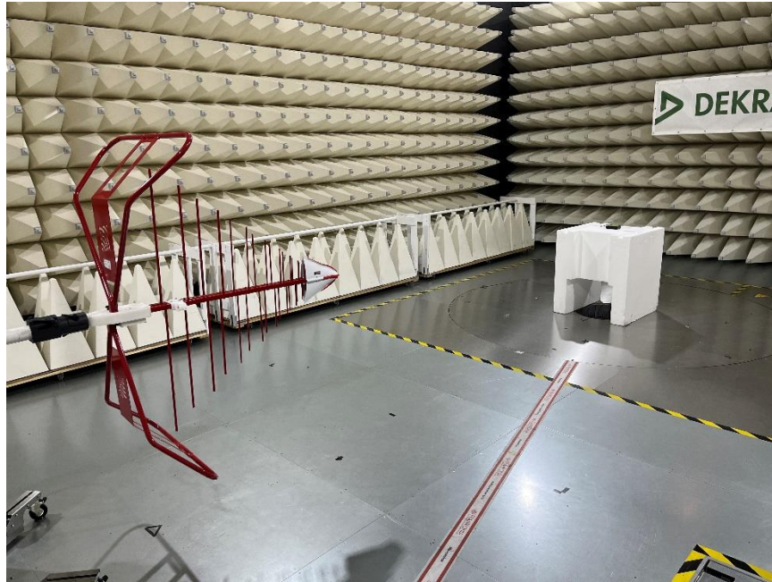
7. Radiated emission Setup 1
