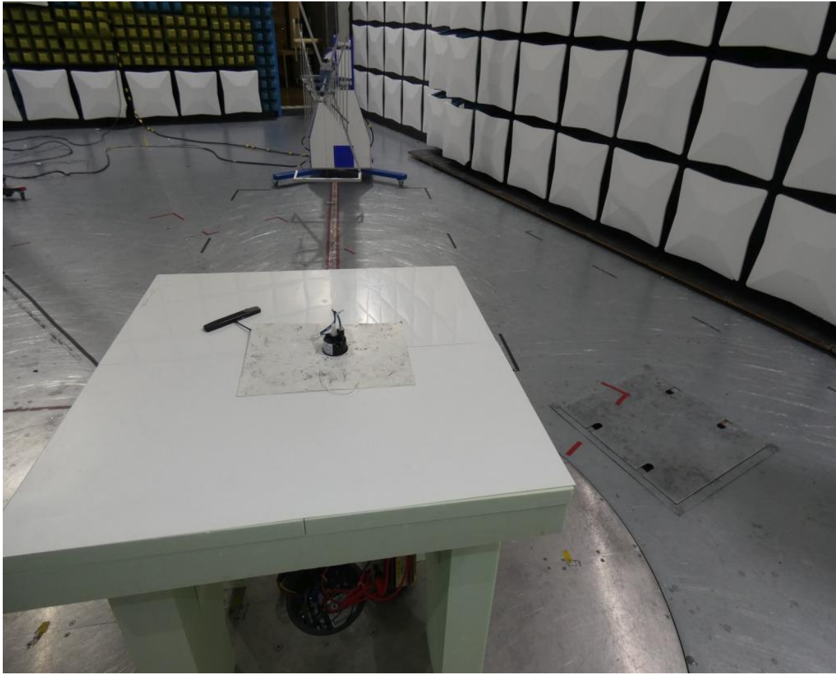
Photo 2: Test setup for radiated measurements (30 MHz - 1 GHz)
