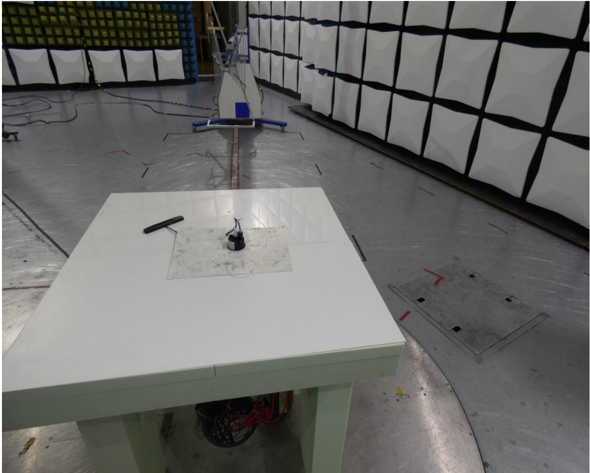
Photo 1: Test setup for radiated measurements (30 MHz - 1 GHz)
