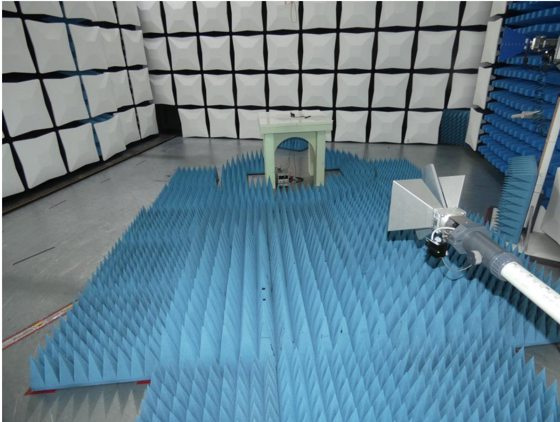
Photo 2: Test setup for radiated measurements (1 GHz – 18 GHz)
