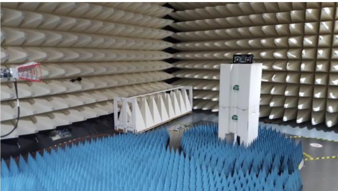
6. Radiated Emission test setup 2
