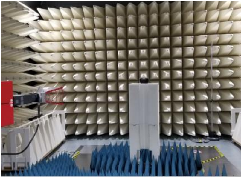
Figure B5. Radiated emission Setup – High Range 1 to 18 GHz
