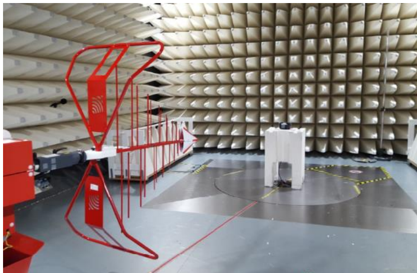
Figure B4. Radiated emission Setup – Low Range 30 to 1000 MHz
