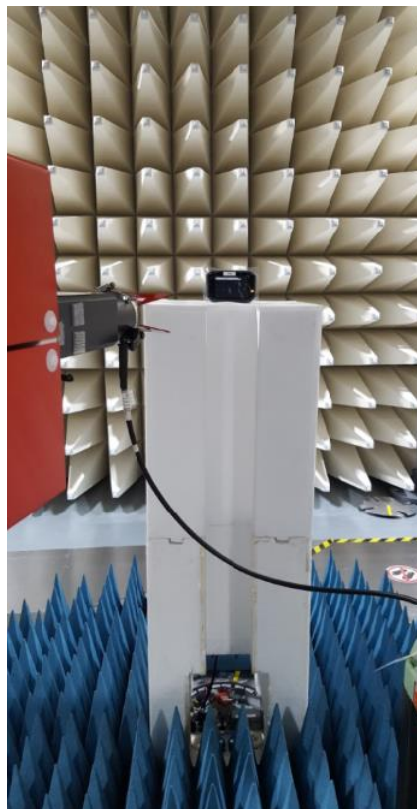
Figure B6. Radiated emission Setup – High Range 18 to 26 GHz
