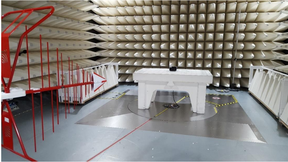
Figure B4. Radiated emission Setup – Low Range 30 to 1000 MHz
