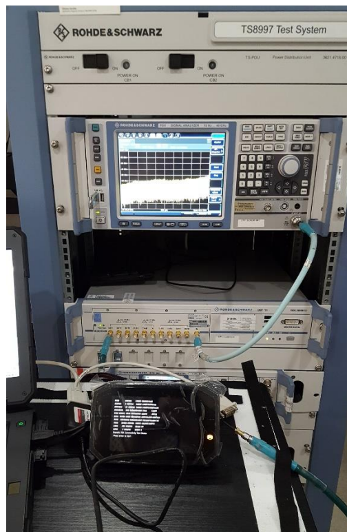
Figure B4. Conducted test setup
