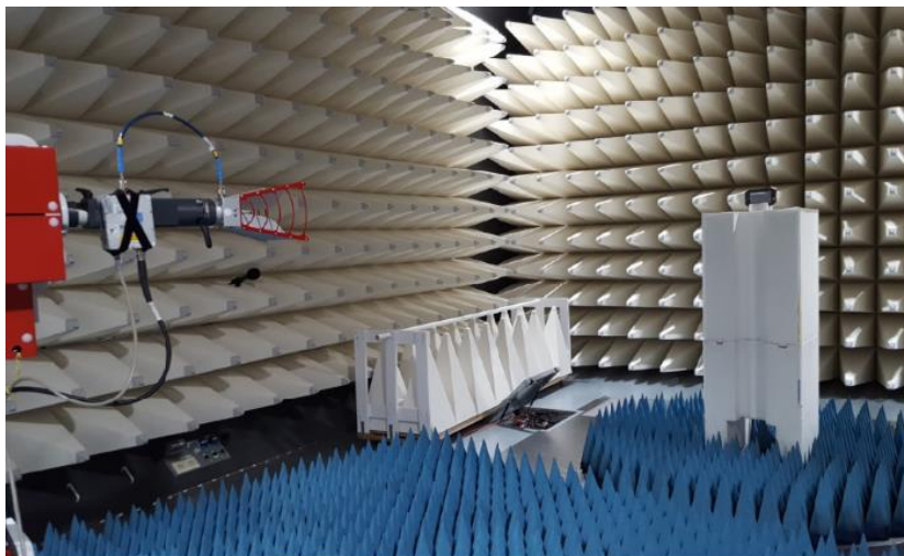
Figure B6. Radiated emission Setup 2
