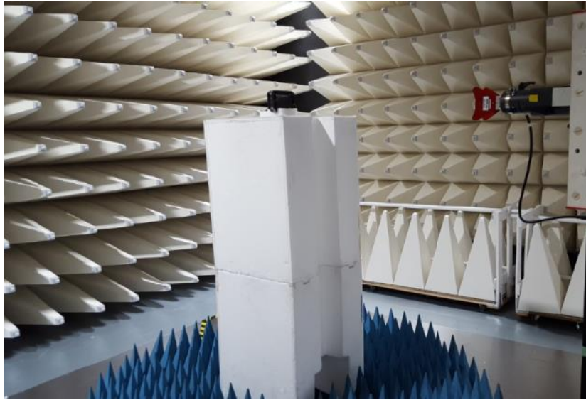
Figure B7. Radiated emission Setup 3
