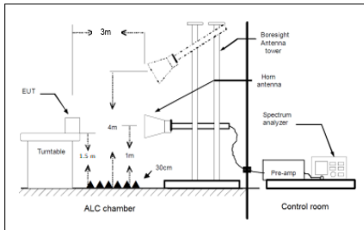
Radiated measurements setup f > 1-18 GHz
