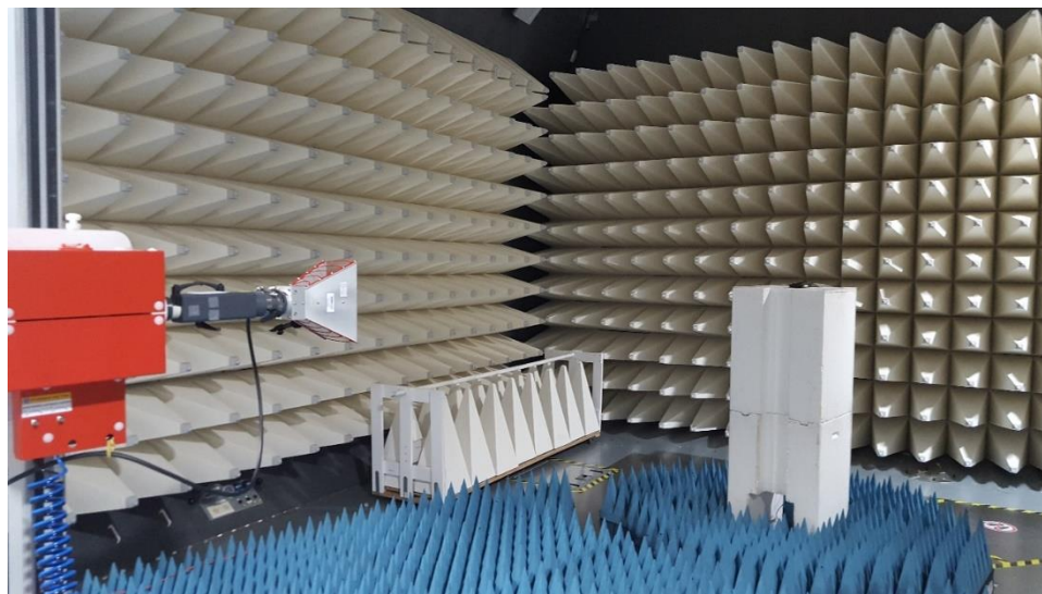
Figure B4. Radiated High Range Setup
