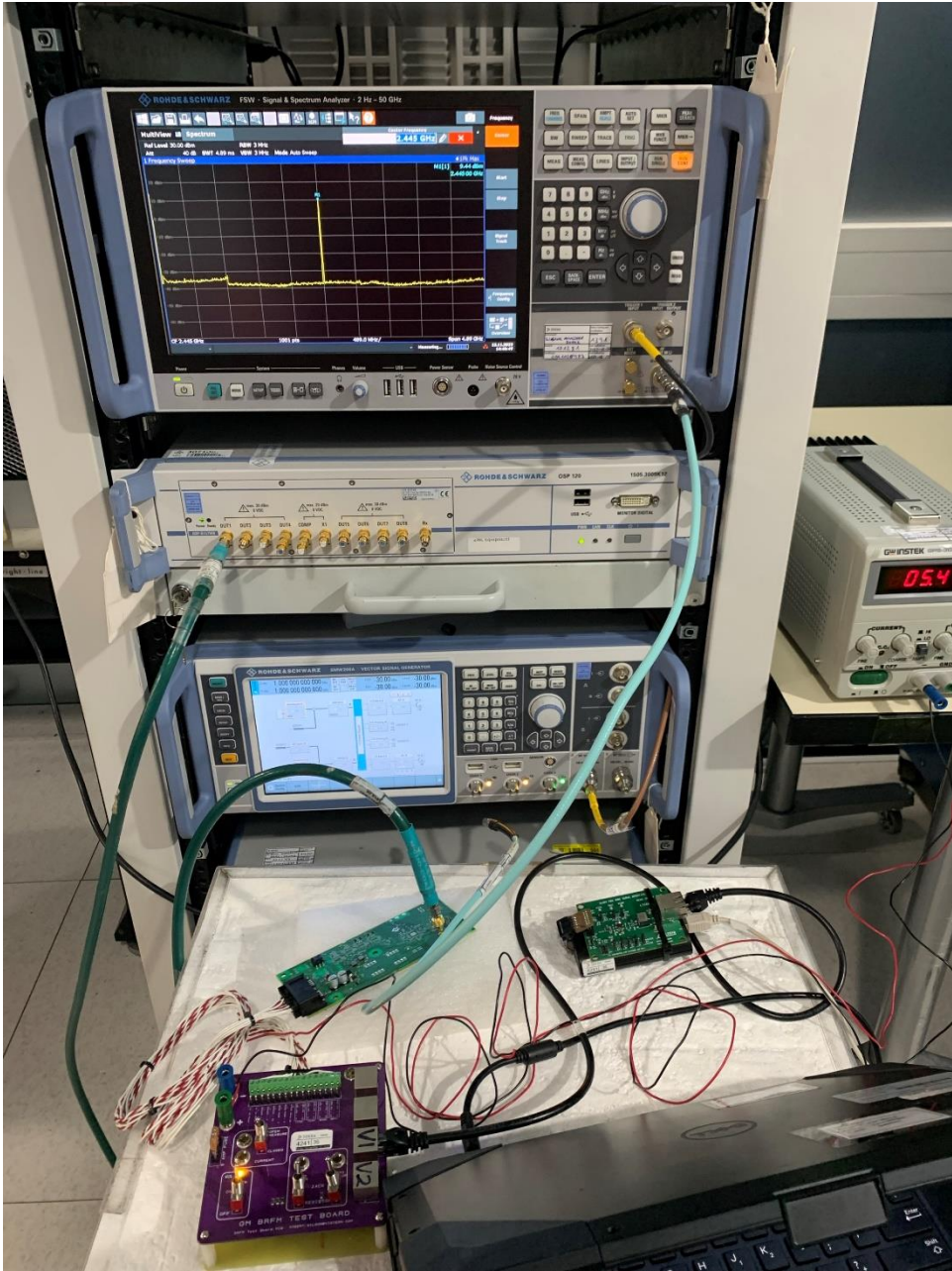
10. Conducted test setup
