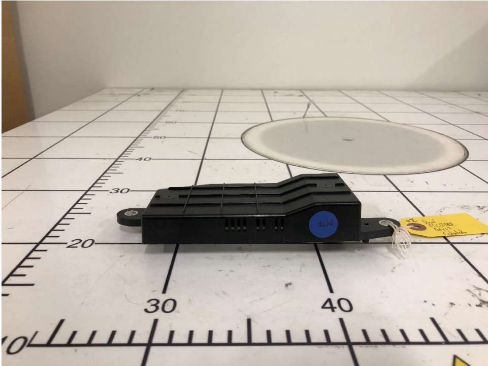
2. Side view of the Radiated DUT
