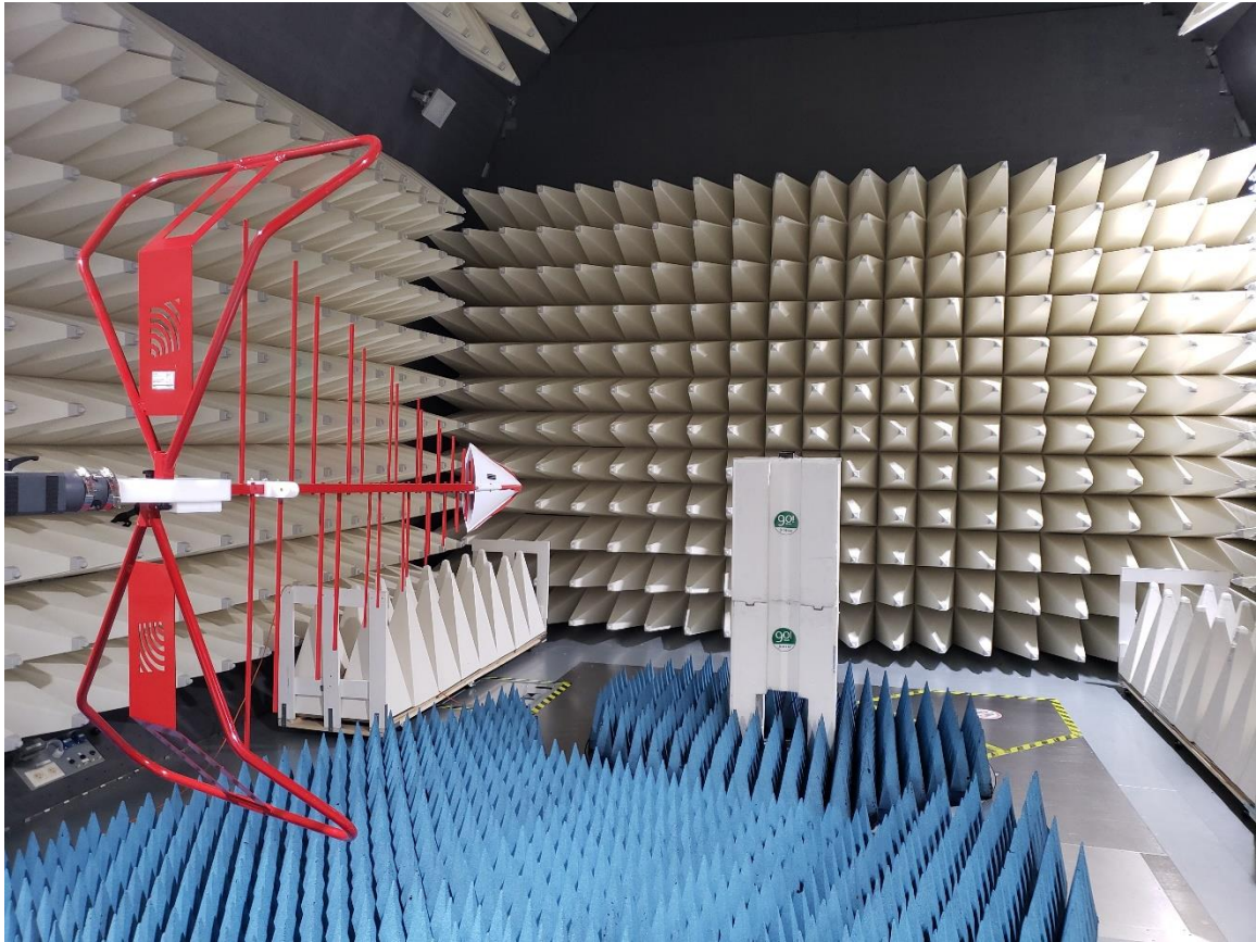
11. Radiated Emission test setup Low Range
