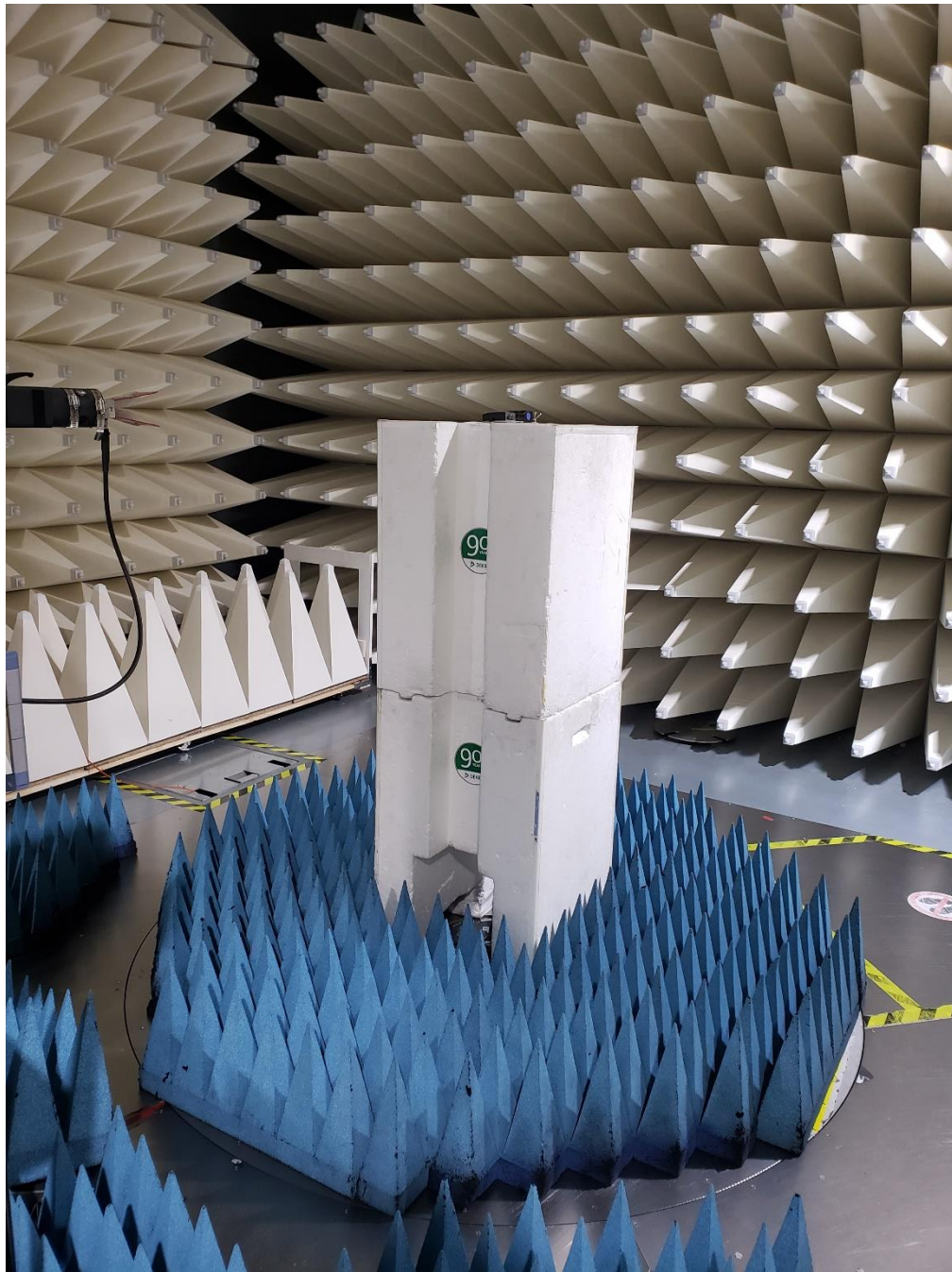
12. Radiated Emission test setup High Range
