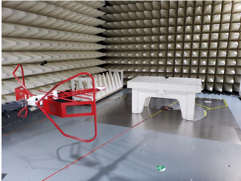
8. Radiated Emission test setup Low Range
