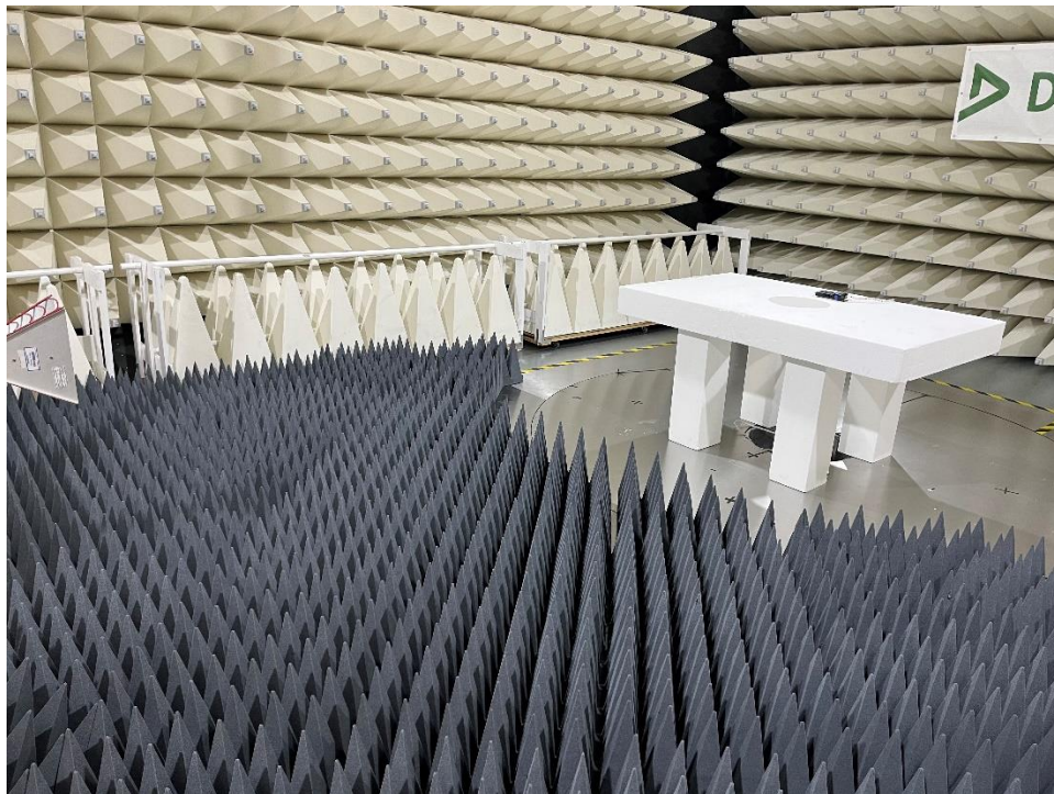
9. Radiated Emission test setup High Range
