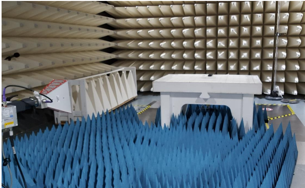
Figure B6. Radiated emission Setup 2 – High Range 1 to 18 GHz
