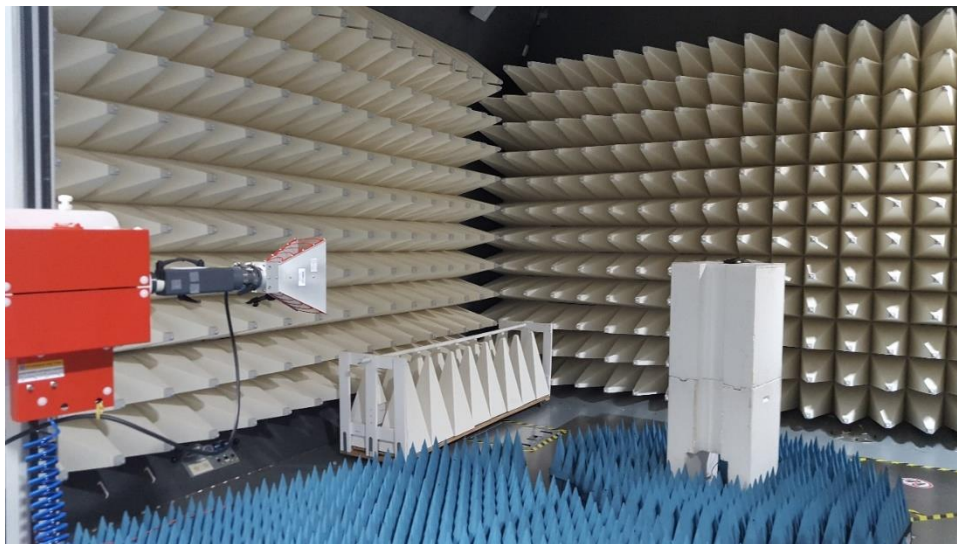
Figure B4. Radiated High Range Setup for DUT
