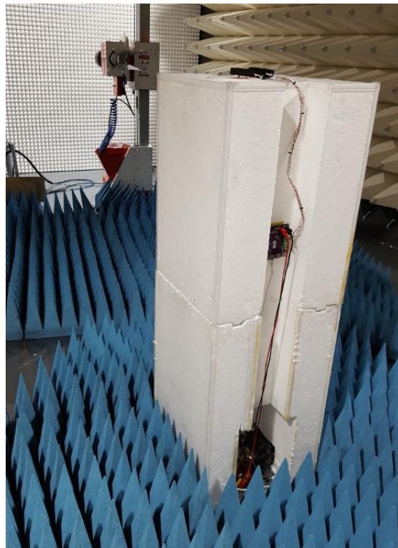
Figure B8. Radiated emission Test Setup 3
