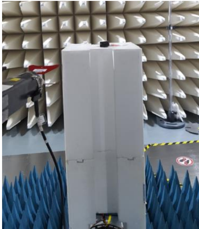
Figure B9. Radiated emission Test Setup 4
