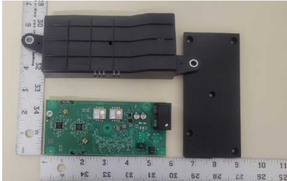
Figure B3. Conducted DUT
