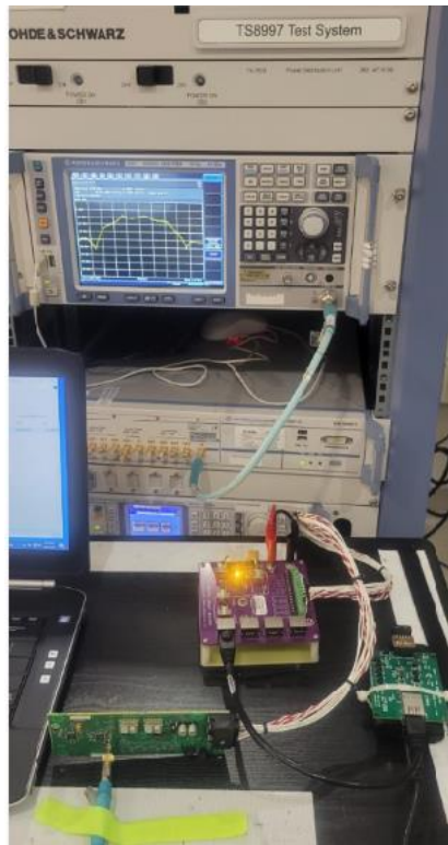
Figure B5. Conducted test setup
