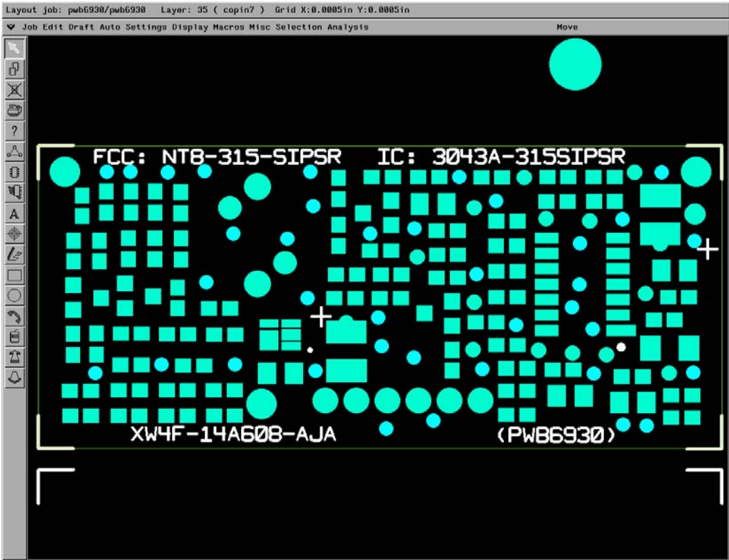
ID label silkscreen for receiver
