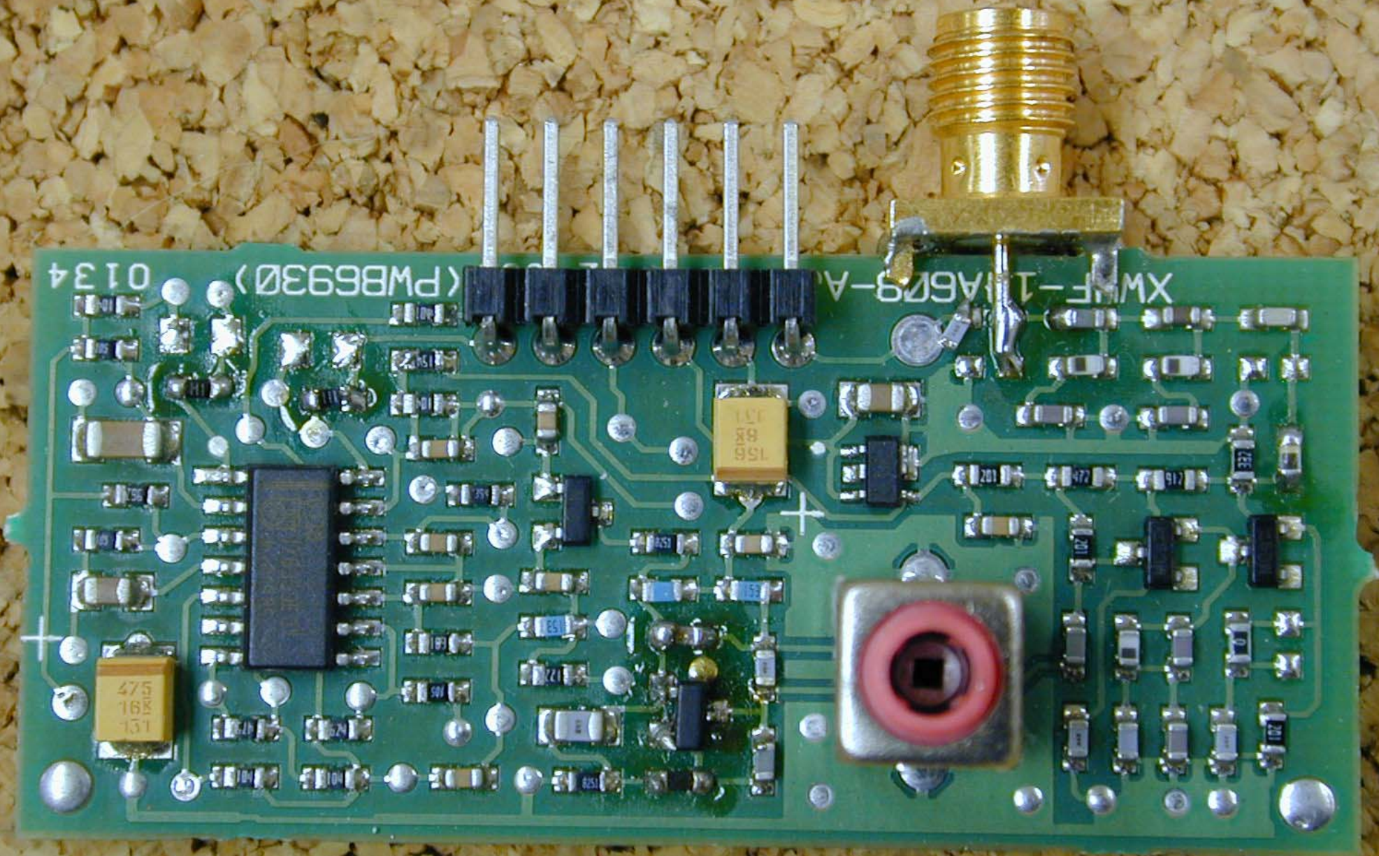
RX Top with connector
