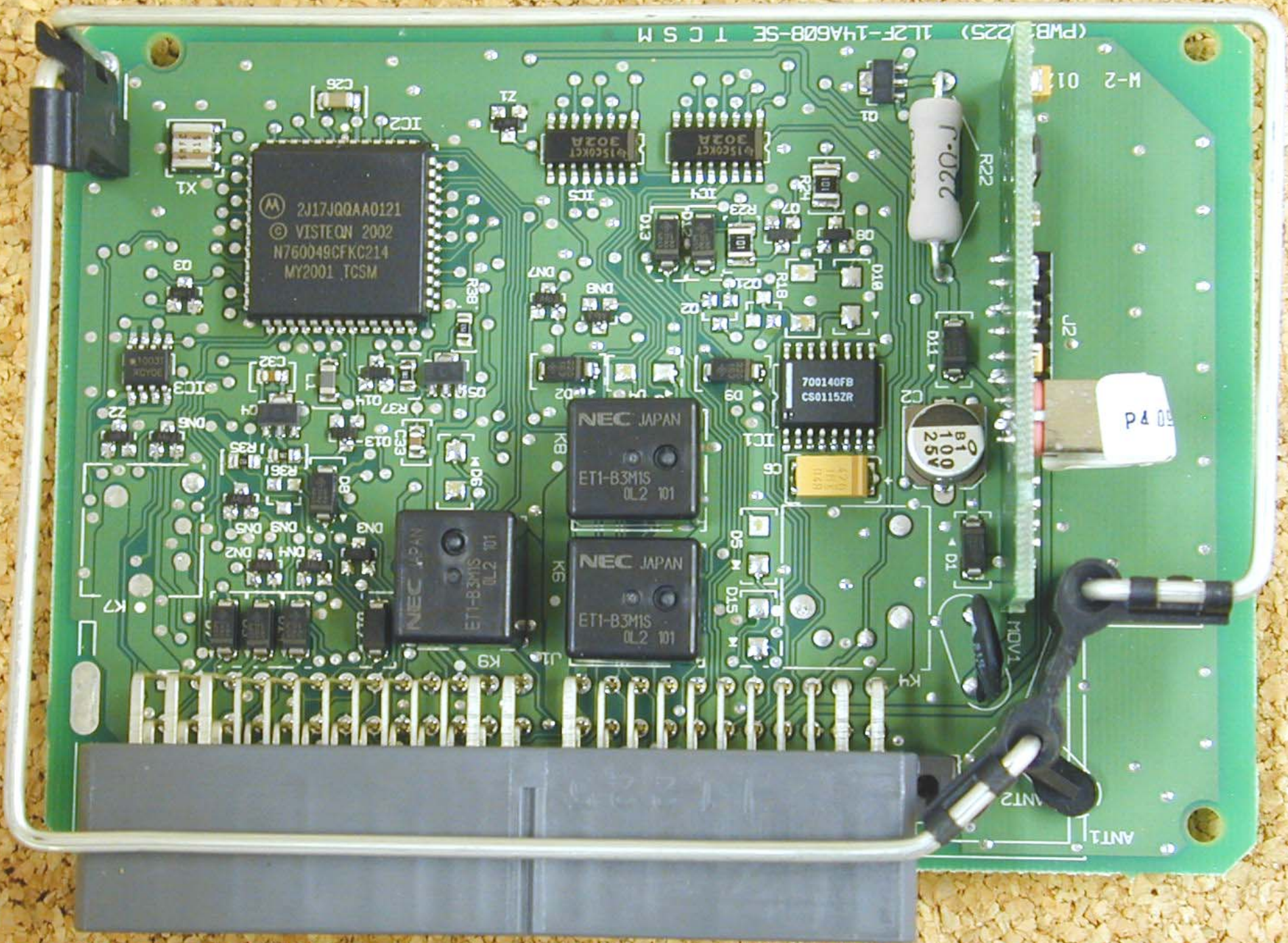
RKE TCSM, PCB, Top
