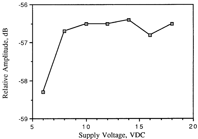
Figure 6.2. Relative emission at "fundamental" vs. supply voltage.
