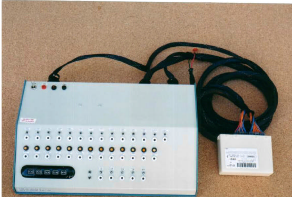
DUT as Tested with the Harness and Control Box
