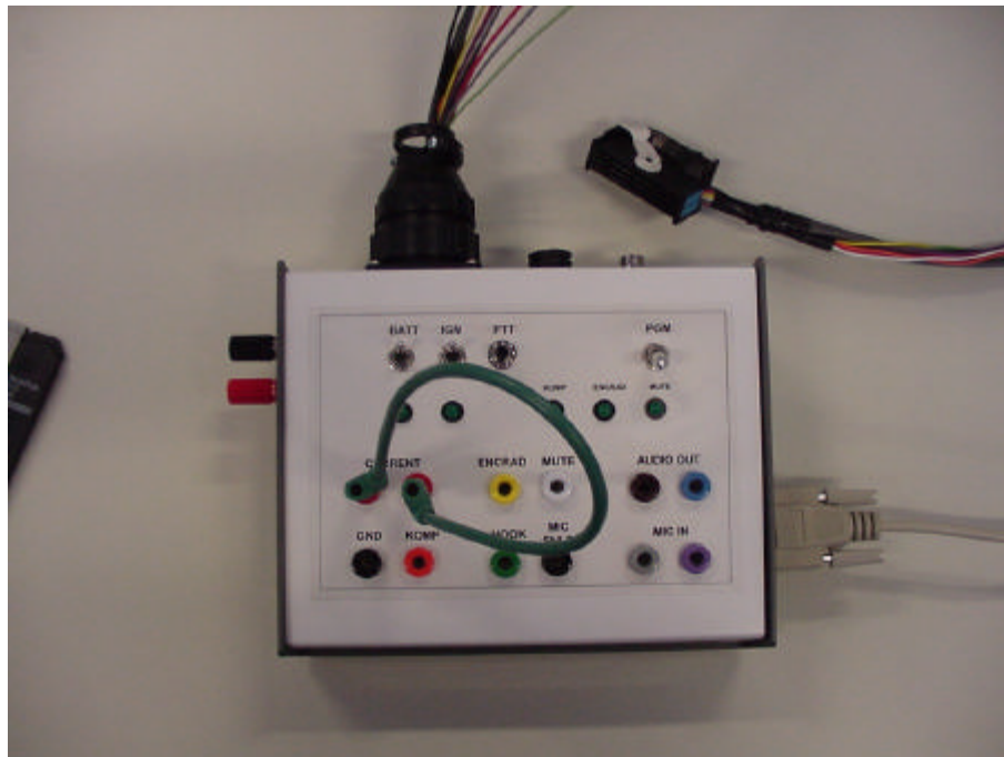
Picture 3 : Visteon Control board (top side)
