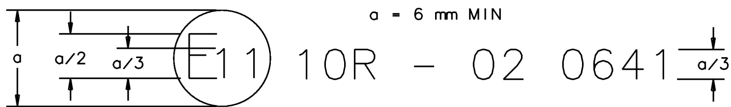
DETAIL A SCALE 4:1
