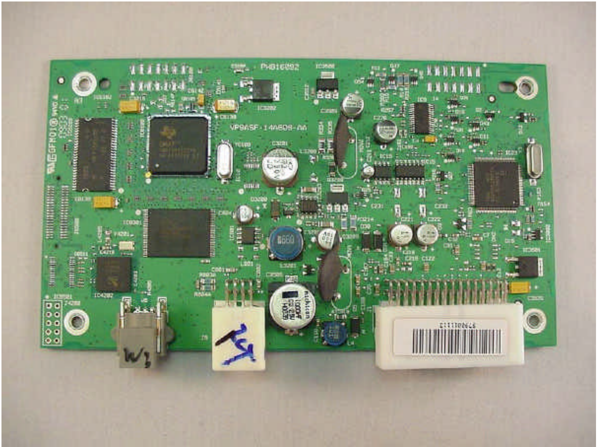
Photo 6: PCB of EUT (top side) The photo does not show one of the tested samples.
