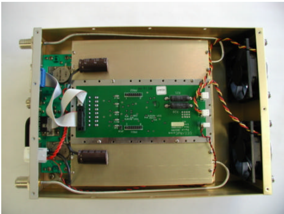
DAC Internal Top View
