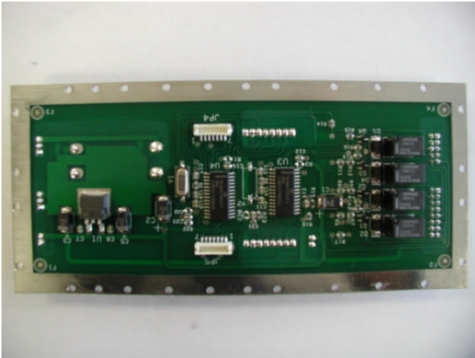
Logic Board Front View
