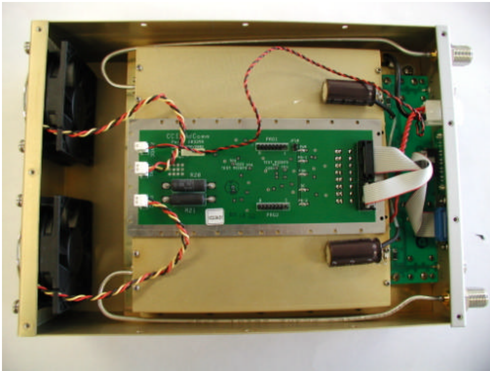
DAB Internal Top View
