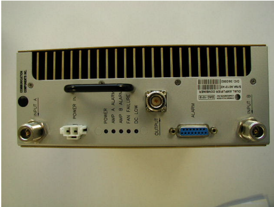
DAC1819 - Front View
