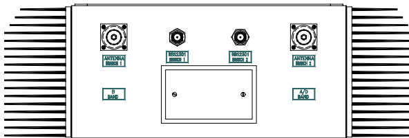
VIEW WITHOUT POWER SUPPLY
