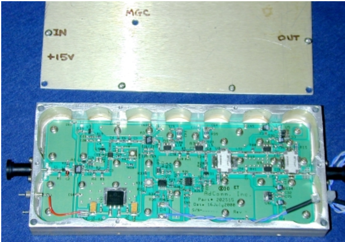
Photo 2 - Manual Gain Controlled Amplifier (Existing Amplifier Version)
