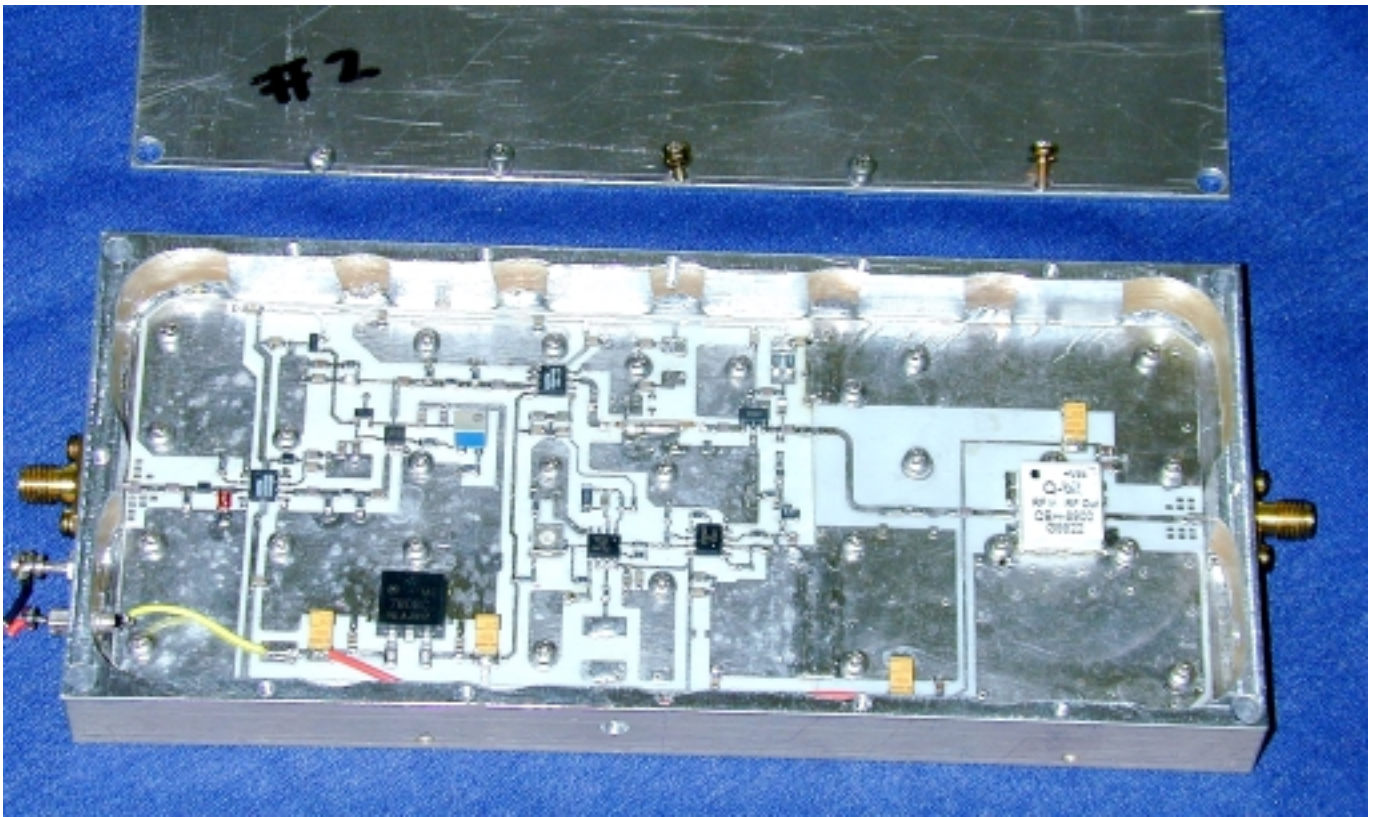
Photo 1 - Auto Gain Controlled Amplifier (New Amplifier Version)
