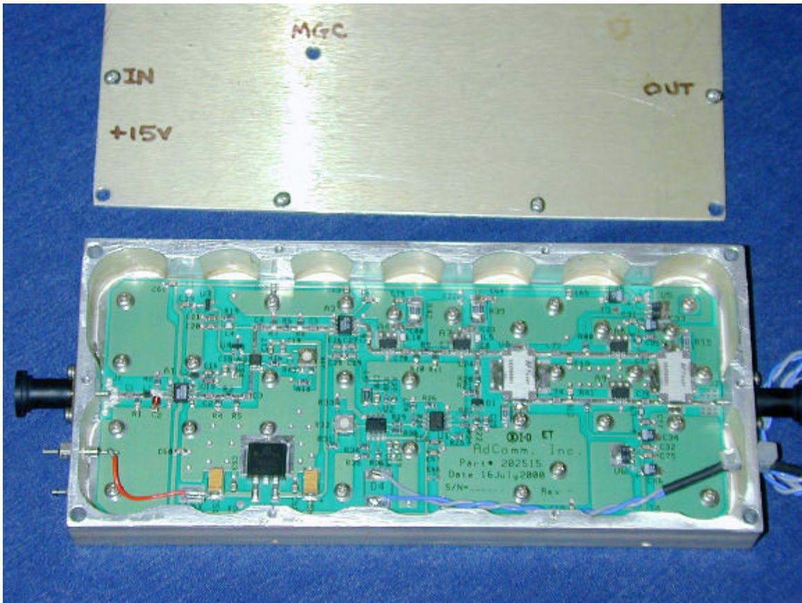
Photo 6 - MGC Amplifier
