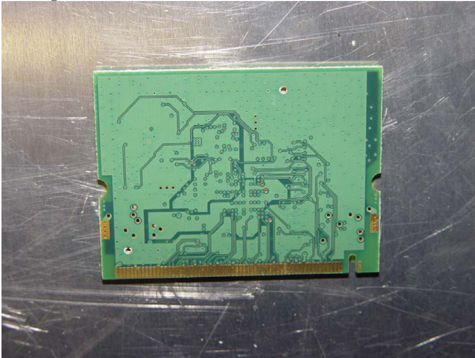
802.11b/g RF Card Bottom
