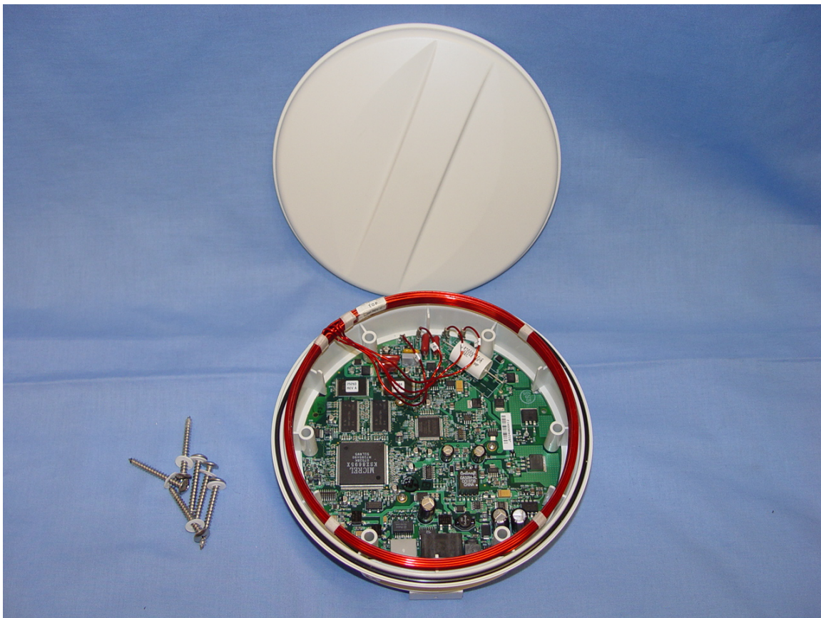
Internal Assembly complete with coil antenna
