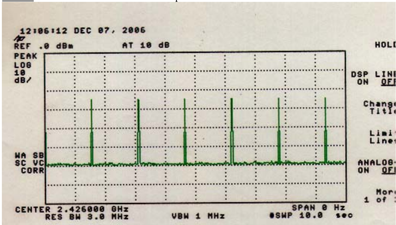
Plot #5: 802.11b Transmission at fastest repetition rate of 1.5 seconds between “blinks”.
