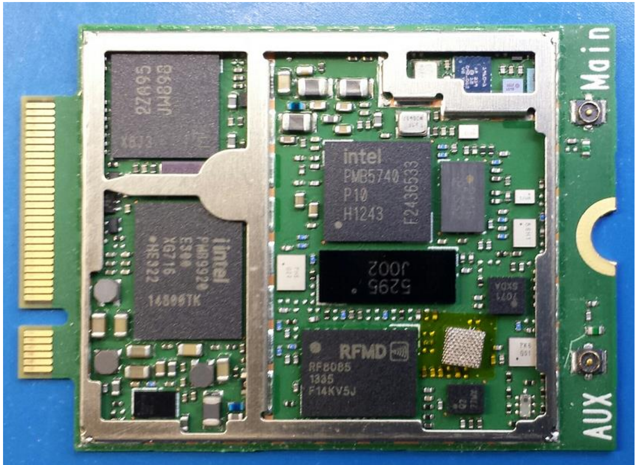
Internal LN930 Shield Removed Card Top
