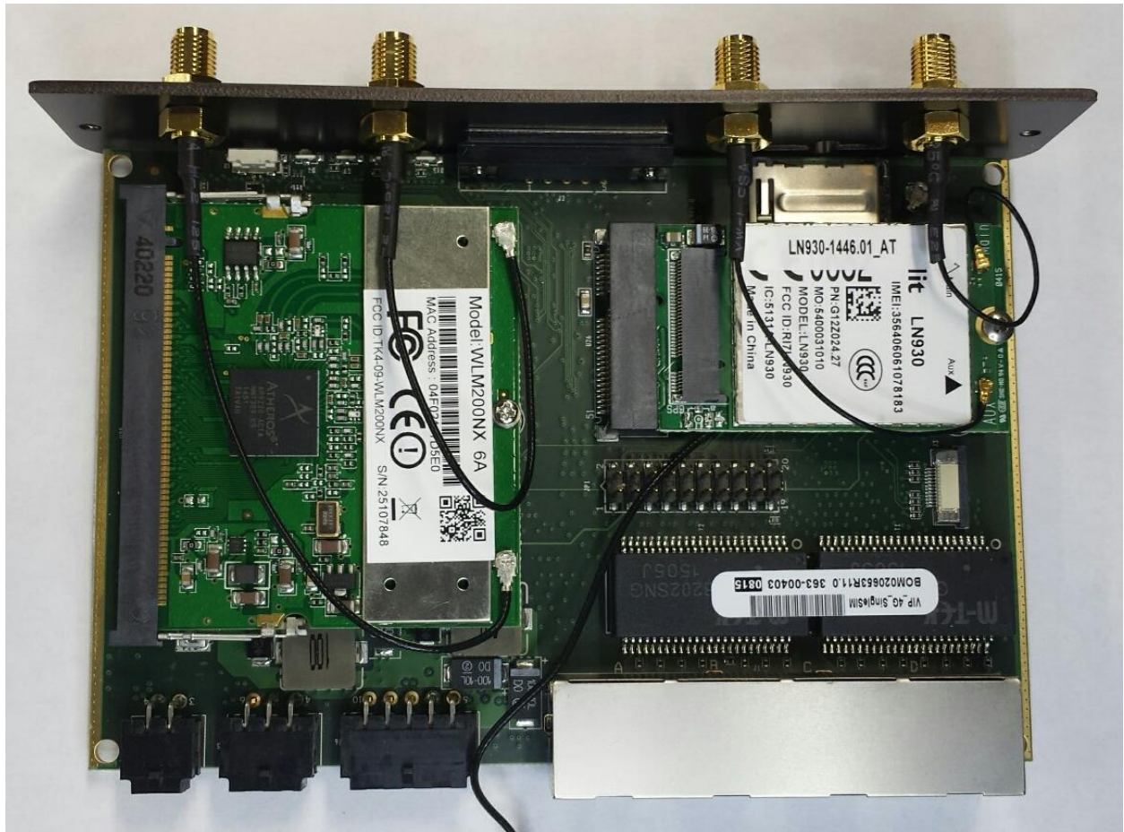
Internal Photo Assembled
