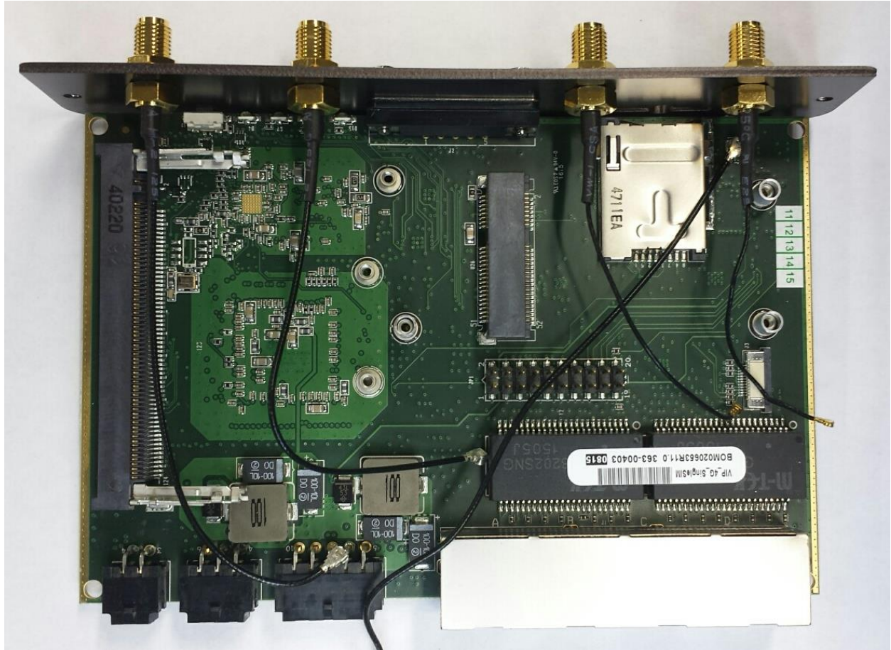
Internal Photo Cards Removed
