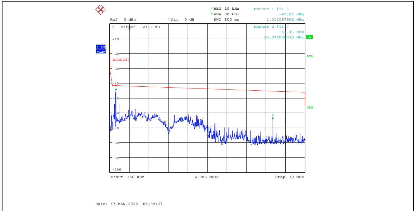
Plot C.2.74. Conducted Spurious Emissions in Restricted Frequency Bands, Chain 2 20 MHz Channel Bandwidth, Data Rate 7, Raw Power Setting 23, 2437 MHz, 150 kHz – 30 MHz, Peak Detector
