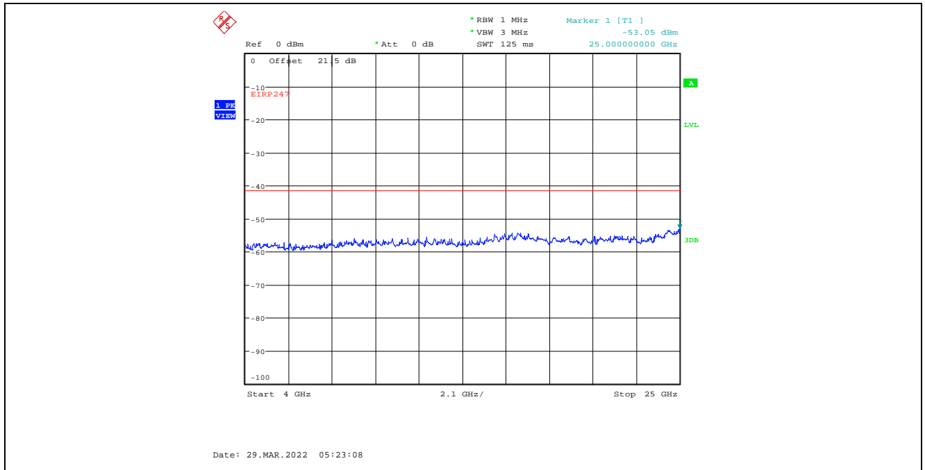
Plot C.4.90. Conducted Spurious Emissions in Restricted Frequency Bands, Chain 2 20 MHz Channel Bandwidth, Data Rate 7, Raw Power Setting 0, 2462 MHz, 4 GHz - 25 GHz, Peak Detector
