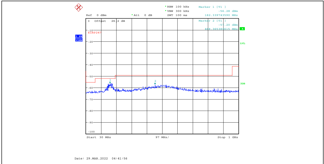
Plot C.3.86. Conducted Spurious Emissions in Restricted Frequency Bands, Chain 2 20 MHz Channel Bandwidth, Data Rate 3, Raw Power Setting 7, 2462 MHz, 30 MHz - 1 GHz, Peak Detector
