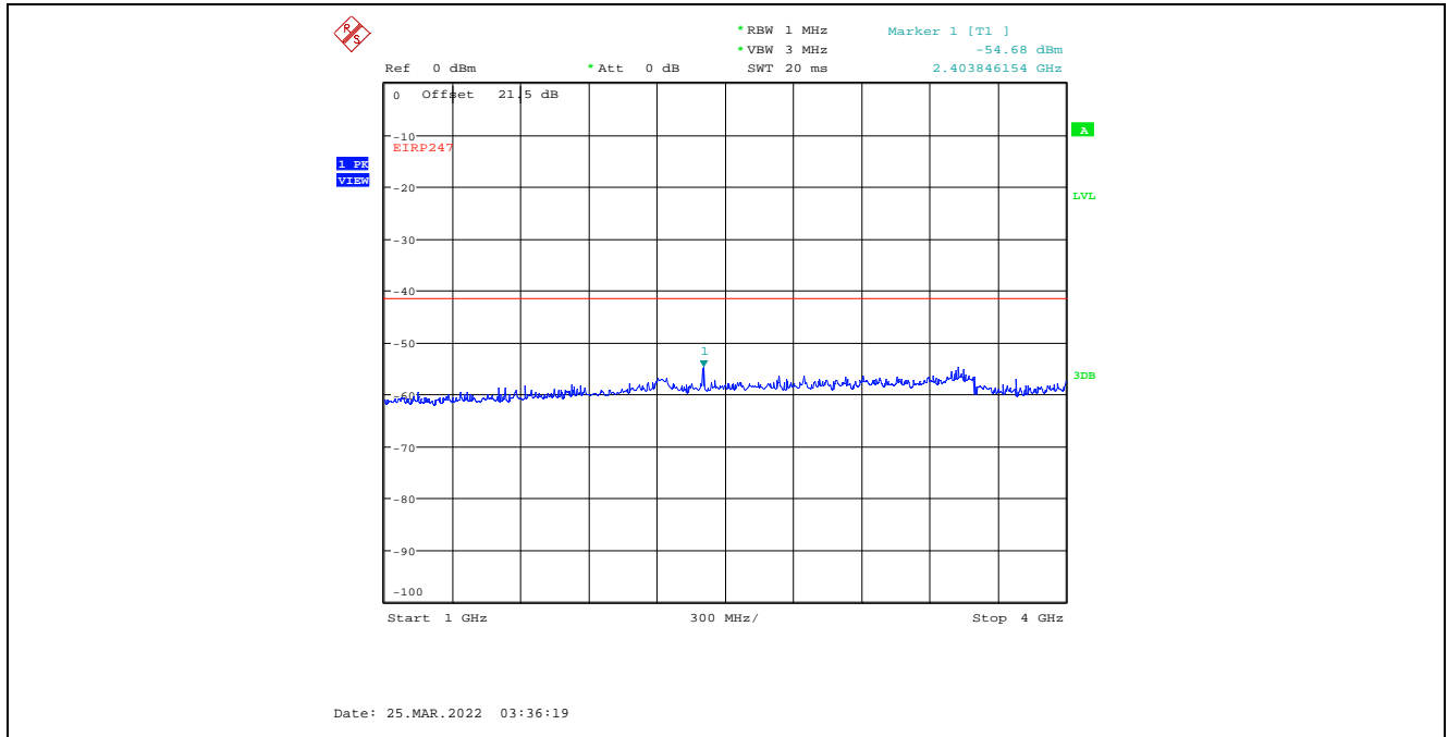
Plot C.3.8. Conducted Spurious Emissions in Restricted Frequency Bands, Chain 1 4 MHz Channel Bandwidth, Data Rate 3, Raw Power Setting 8, 2402 MHz, 1 GHz - 4 GHz, Peak Detector
