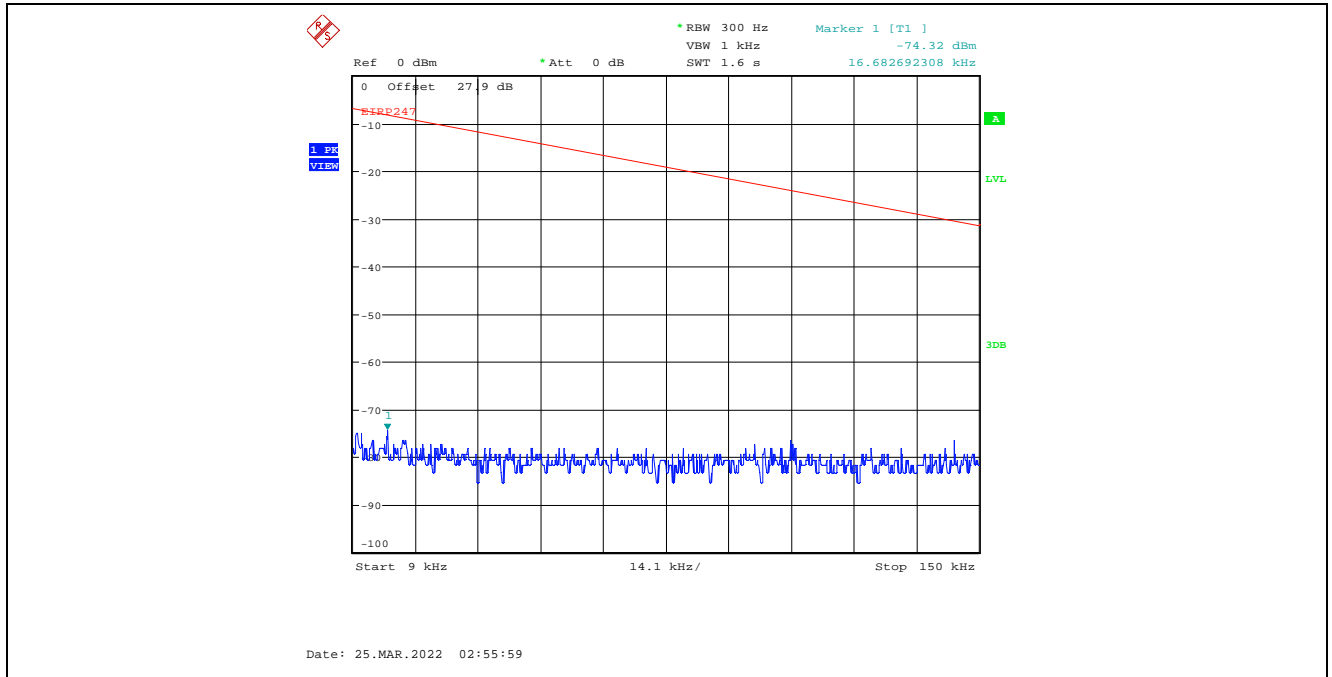
Plot C.3.22. Conducted Spurious Emissions in Restricted Frequency Bands, Chain 2 4 MHz Channel Bandwidth, Data Rate 3, Raw Power Setting 0, 2477 MHz, 9 kHz - 150 kHz, Peak Detector
