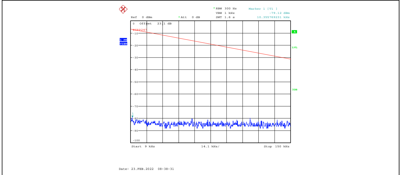
Plot C.1.1. Conducted Spurious Emissions in Restricted Frequency Bands, Chain 1 4 MHz Channel Bandwidth, Data Rate 3, Raw Power Setting 16, 2402 MHz, 9 kHz - 150 kHz, Peak Detector
