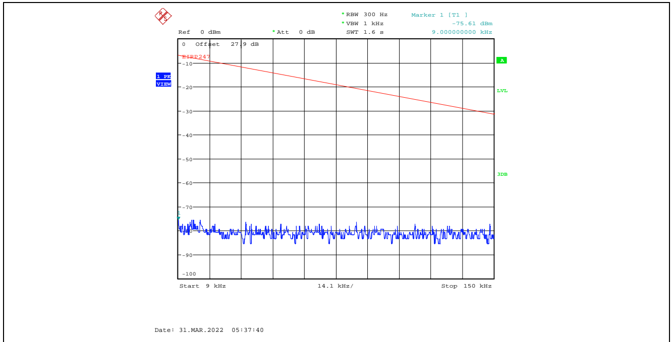
Plot C.4.92. Conducted Spurious Emissions in Restricted Frequency Bands, Chain 2 40 MHz Channel Bandwidth, Data Rate 7, Raw Power Setting 0, 2422 MHz, 9 kHz - 150 kHz, Peak Detector
