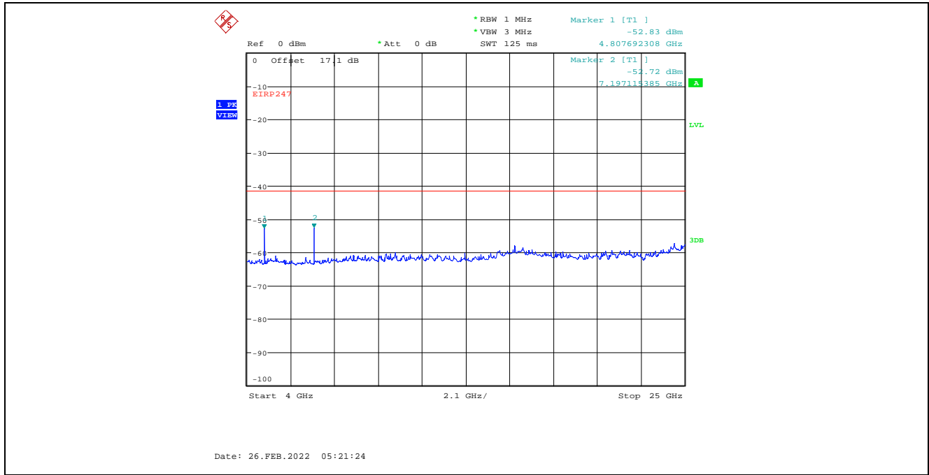
Plot C.2.9. Conducted Spurious Emissions in Restricted Frequency Bands, Chain 1 4 MHz Channel Bandwidth, Data Rate 7, Raw Power Setting 22, 2405 MHz, 4 GHz - 25 GHz, Peak Detector
