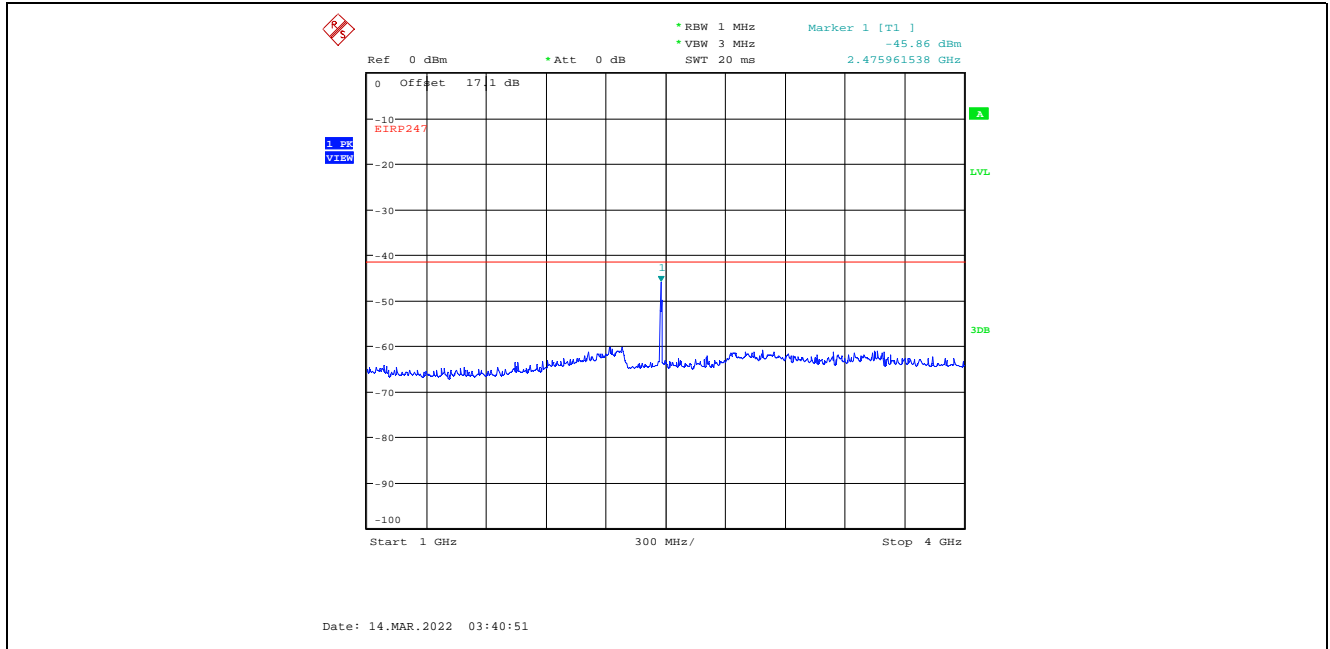
Plot C.1.57. Conducted Spurious Emissions in Restricted Frequency Bands, Chain 1 8 MHz Channel Bandwidth, Data Rate 3, Raw Power Setting 14, 2476 MHz, 1 GHz – 4 GHz, Peak Detector Marker 1 is Fundamental Signal
