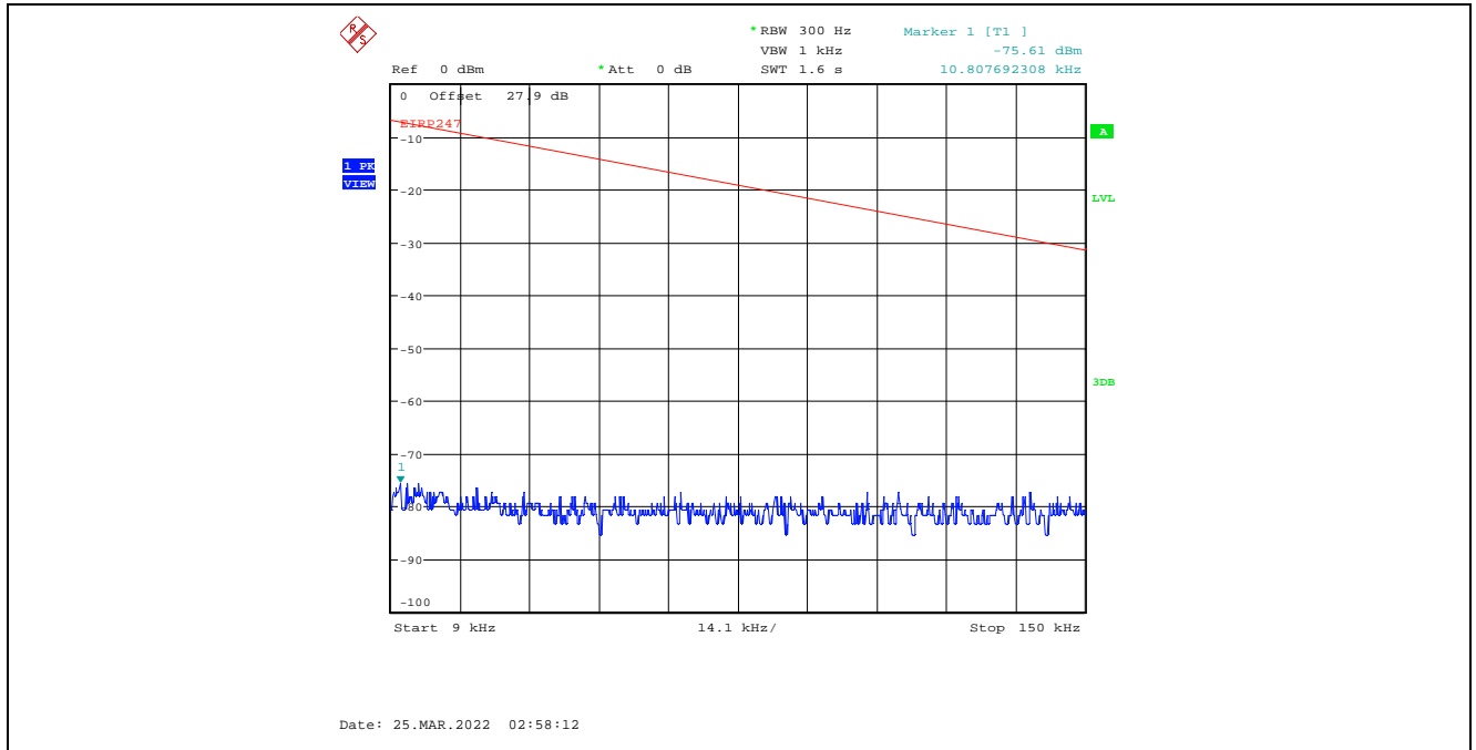
Plot C.3.12. Conducted Spurious Emissions in Restricted Frequency Bands, Chain 2 4 MHz Channel Bandwidth, Data Rate 3, Raw Power Setting 8, 2437 MHz, 9 kHz - 150 kHz, Peak Detector
