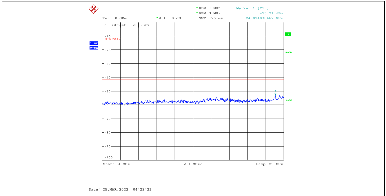
Plot C.4.20. Conducted Spurious Emissions in Restricted Frequency Bands, Chain 2 4 MHz Channel Bandwidth, Data Rate 7, Raw Power Setting 0, 2437 MHz, 4 GHz - 25 GHz, Peak Detector
