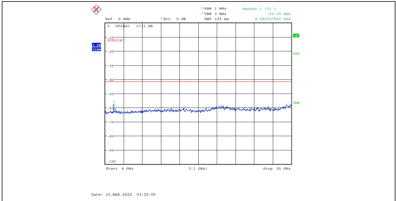
Plot C.2.30. Conducted Spurious Emissions in Restricted Frequency Bands, Chain 2 4 MHz Channel Bandwidth, Data Rate 7, Raw Power Setting 20, 2477 MHz, 4 GHz - 25 GHz, Peak Detector
