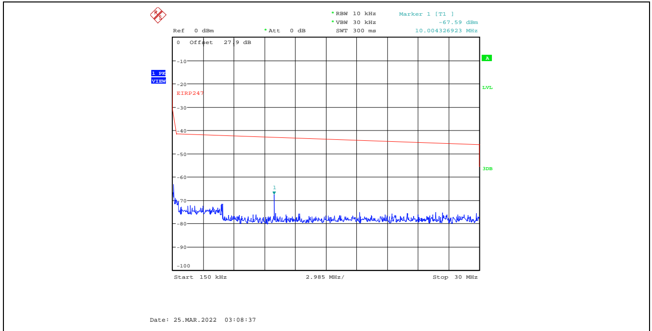
Plot C.3.24. Conducted Spurious Emissions in Restricted Frequency Bands, Chain 2 4 MHz Channel Bandwidth, Data Rate 3, Raw Power Setting 0, 2477 MHz, 150 kHz – 30 MHz, Peak Detector
