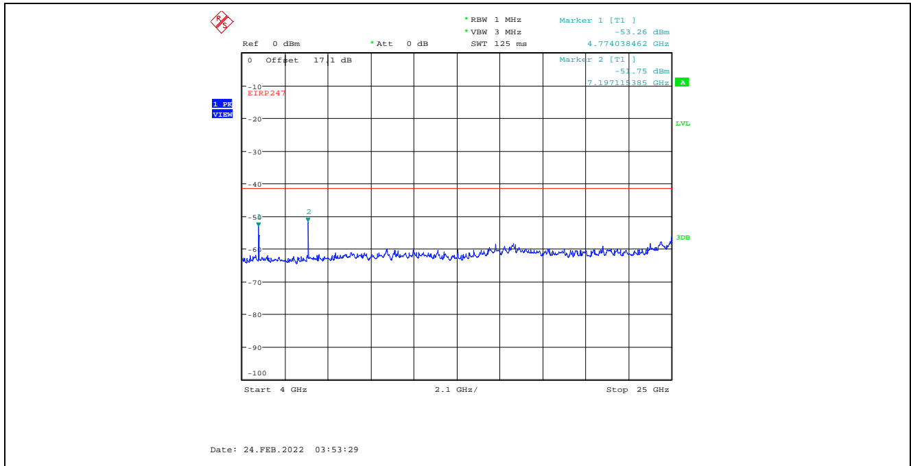
Plot C.1.10. Conducted Spurious Emissions in Restricted Frequency Bands, Chain 2 4 MHz Channel Bandwidth, Data Rate 3, Raw Power Setting 16, 2402 MHz, 4 GHz - 25 GHz, Peak Detector
