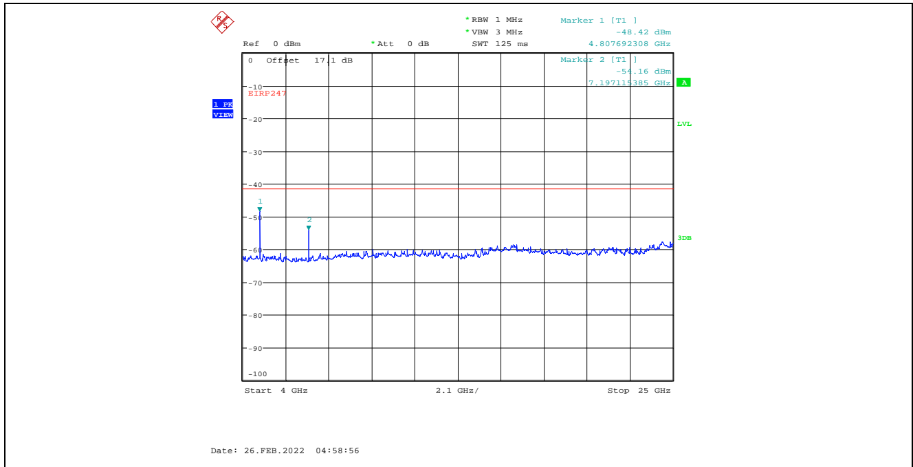
Plot C.2.10. Conducted Spurious Emissions in Restricted Frequency Bands, Chain 2 4 MHz Channel Bandwidth, Data Rate 7, Raw Power Setting 22, 2405 MHz, 4 GHz - 25 GHz, Peak Detector
