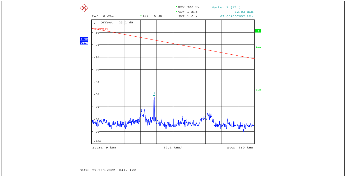
Plot C.2.42. Conducted Spurious Emissions in Restricted Frequency Bands, Chain 2 8 MHz Channel Bandwidth, Data Rate 7, Raw Power Setting 23, 2437 MHz, 9 kHz - 150 kHz, Peak Detector
