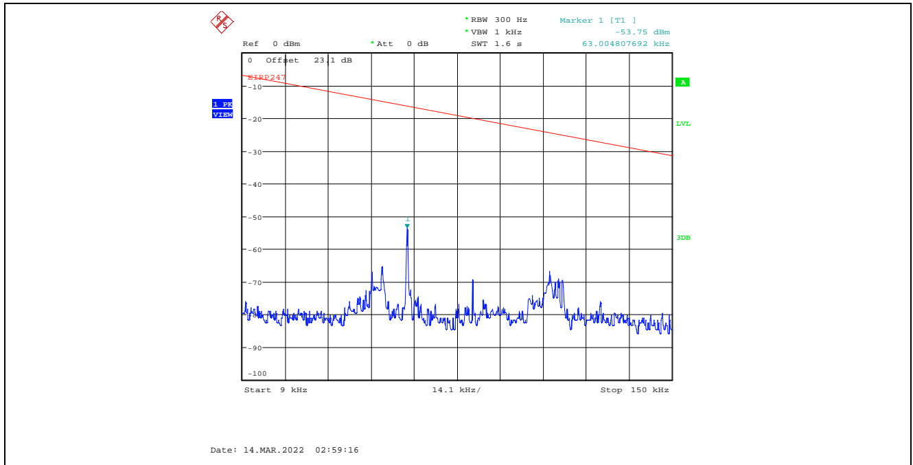
Plot C.1.52. Conducted Spurious Emissions in Restricted Frequency Bands, Chain 2 8 MHz Channel Bandwidth, Data Rate 3, Raw Power Setting 14, 2476 MHz, 9 kHz - 150 kHz, Peak Detector
