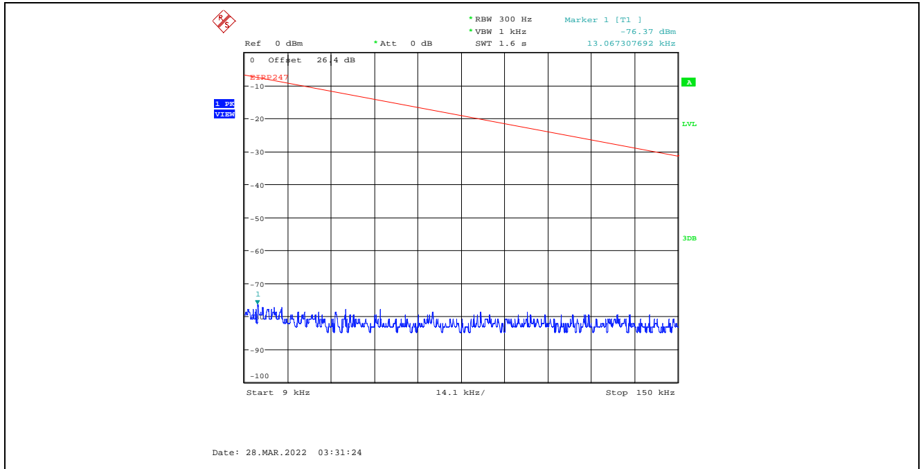
Plot C.4.41. Conducted Spurious Emissions in Restricted Frequency Bands, Chain 1 8 MHz Channel Bandwidth, Data Rate 7, Raw Power Setting 0, 2437 MHz, 9 kHz - 150 kHz, Peak Detector
