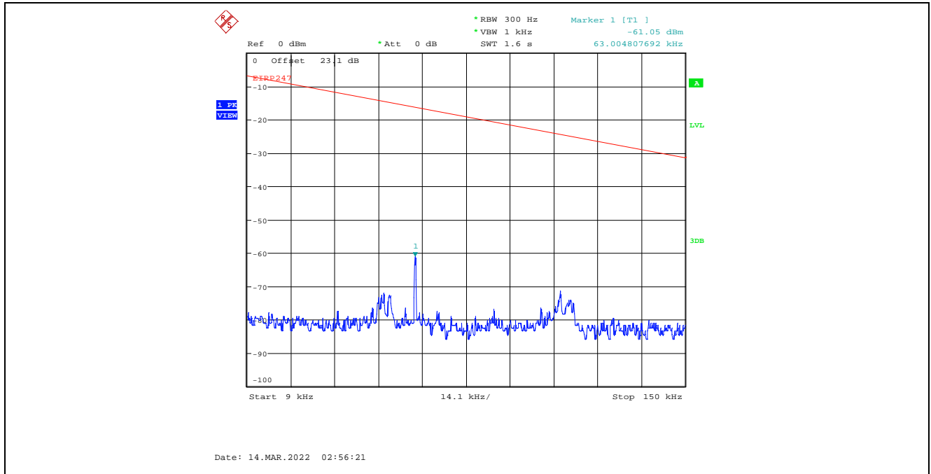
Plot C.1.51. Conducted Spurious Emissions in Restricted Frequency Bands, Chain 1 8 MHz Channel Bandwidth, Data Rate 3, Raw Power Setting 14, 2476 MHz, 9 kHz - 150 kHz, Peak Detector
