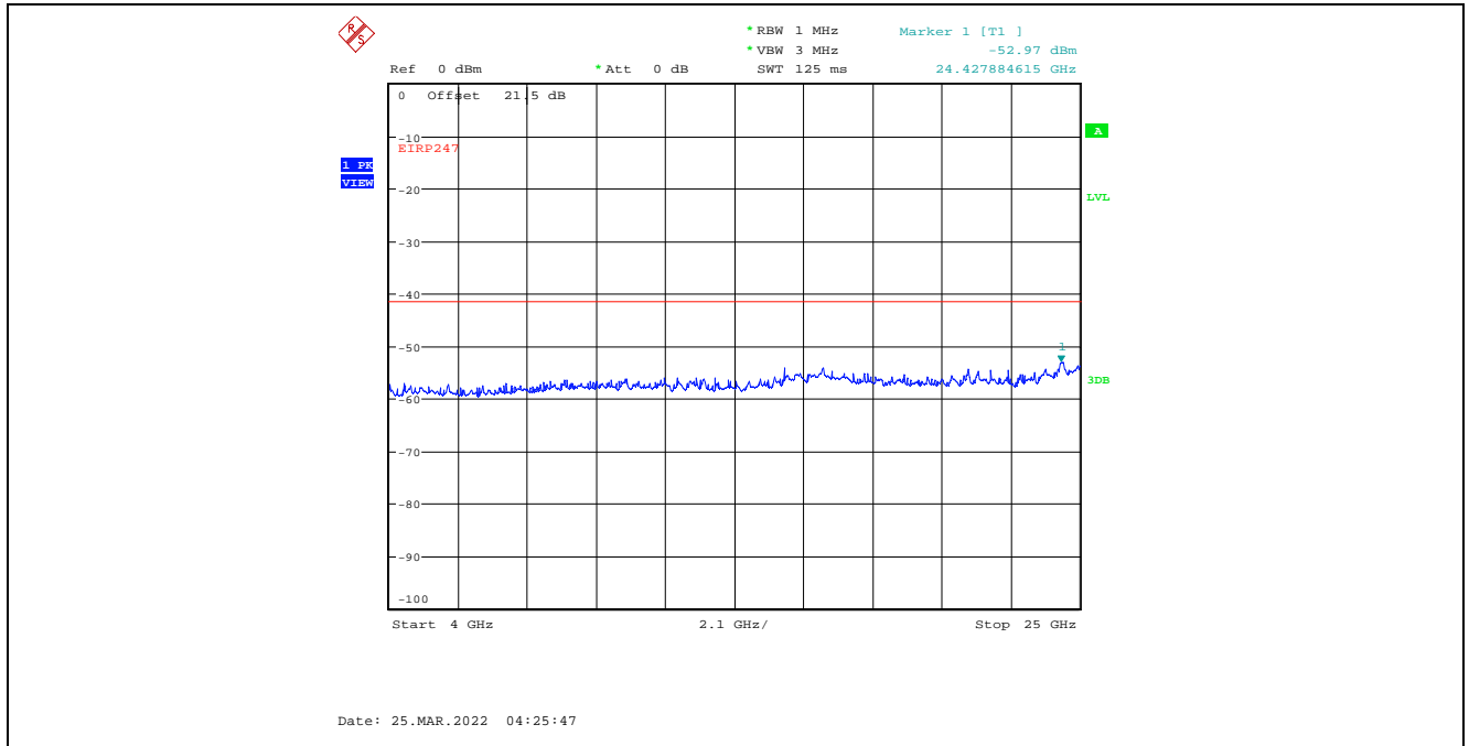
Plot C.4.30. Conducted Spurious Emissions in Restricted Frequency Bands, Chain 2 4 MHz Channel Bandwidth, Data Rate 7, Raw Power Setting 0, 2477 MHz, 4 GHz - 25 GHz, Peak Detector
