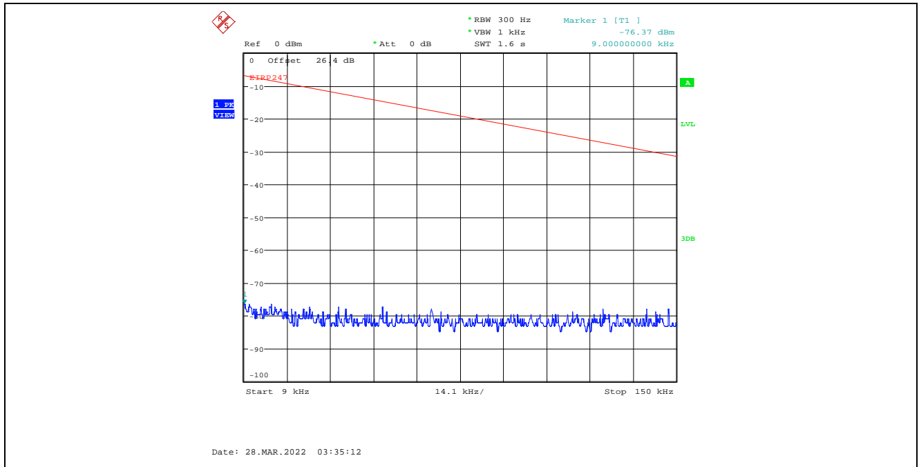
Plot C.4.42. Conducted Spurious Emissions in Restricted Frequency Bands, Chain 2 8 MHz Channel Bandwidth, Data Rate 7, Raw Power Setting 0, 2437 MHz, 9 kHz - 150 kHz, Peak Detector
