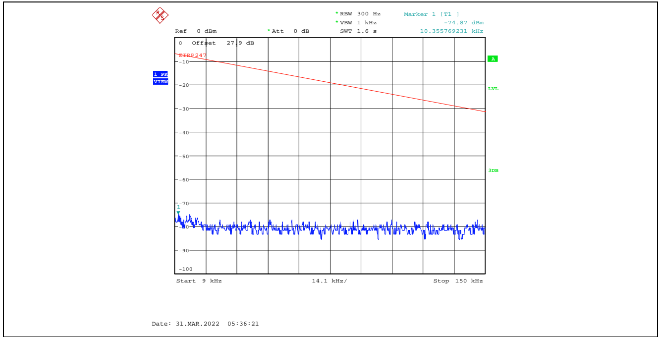
Plot C.4.91. Conducted Spurious Emissions in Restricted Frequency Bands, Chain 1 40 MHz Channel Bandwidth, Data Rate 7, Raw Power Setting 0, 2422 MHz, 9 kHz - 150 kHz, Peak Detector
