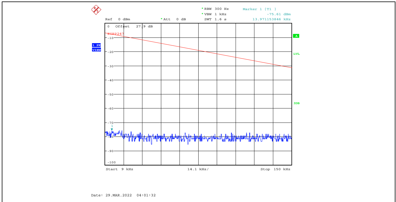
Plot C.3.72. Conducted Spurious Emissions in Restricted Frequency Bands, Chain 2 20 MHz Channel Bandwidth, Data Rate 3, Raw Power Setting 7, 2437 MHz, 9 kHz - 150 kHz, Peak Detector
