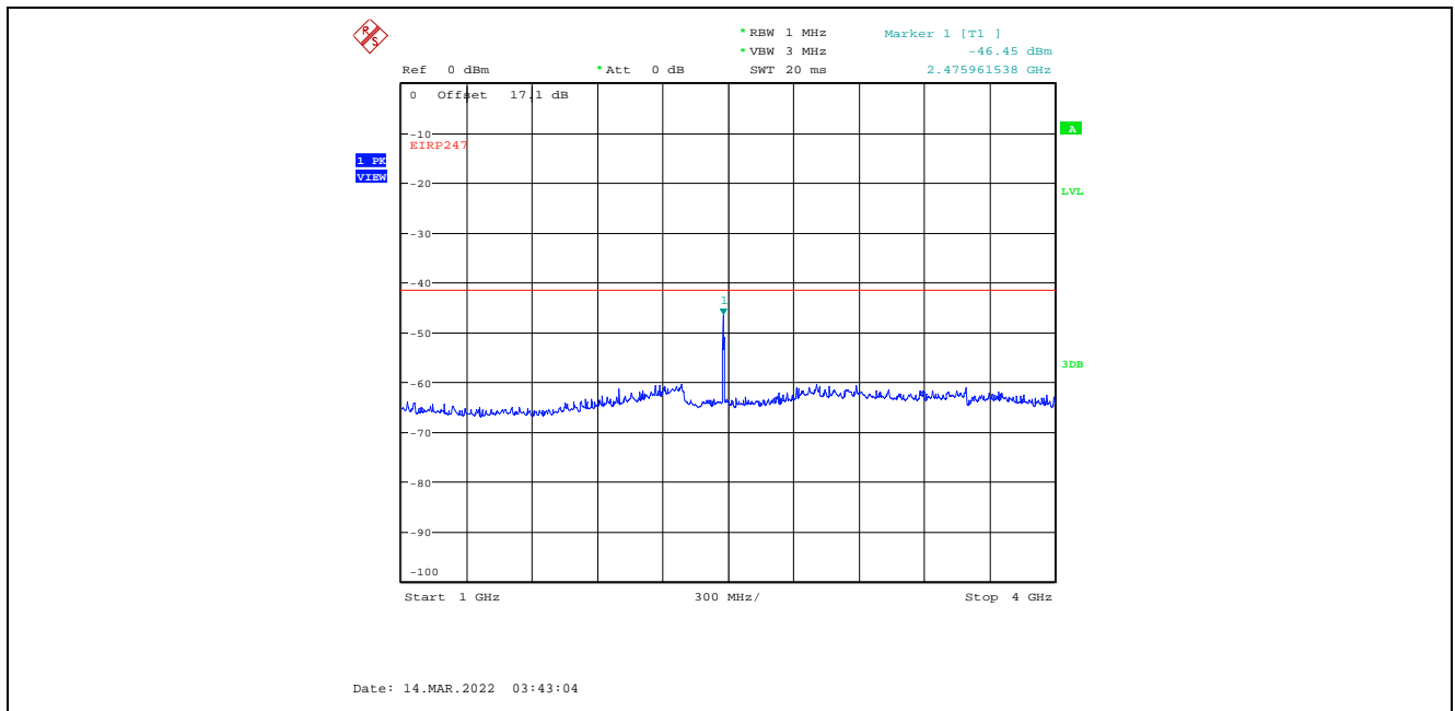
Plot C.1.58. Conducted Spurious Emissions in Restricted Frequency Bands, Chain 2 8 MHz Channel Bandwidth, Data Rate 3, Raw Power Setting 14, 2476 MHz, 1 GHz – 4 GHz, Peak Detector Marker 1 is Fundamental Signal
