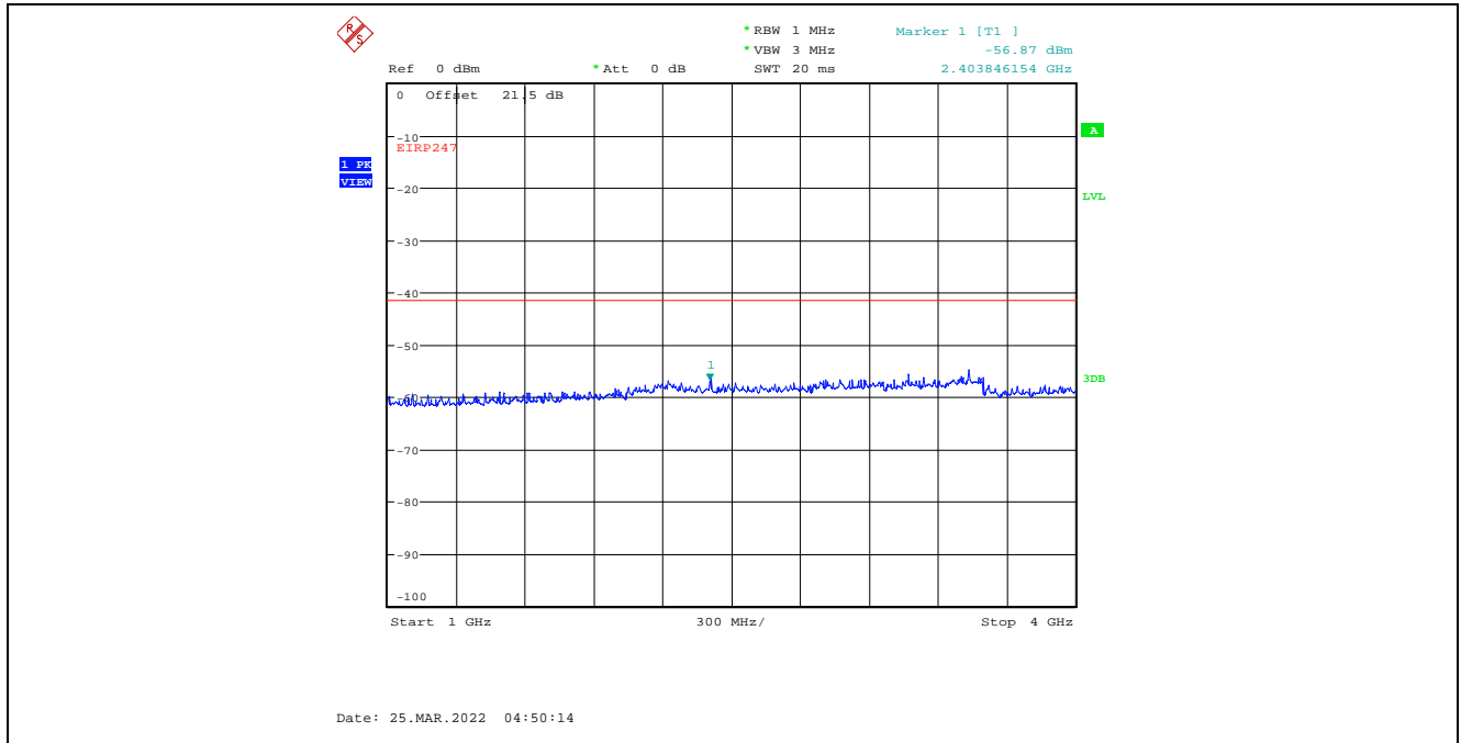
Plot C.4.8. Conducted Spurious Emissions in Restricted Frequency Bands, Chain 1 4 MHz Channel Bandwidth, Data Rate 7, Raw Power Setting 0, 2405 MHz, 1 GHz - 4 GHz, Peak Detector
