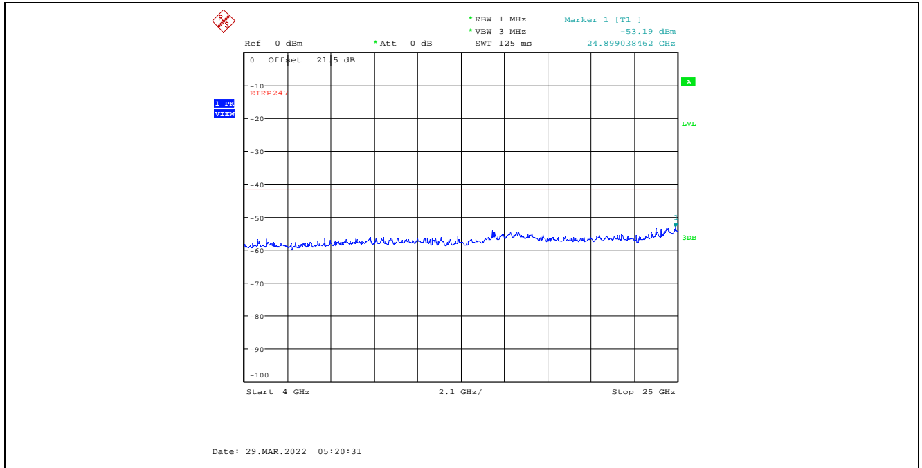
Plot C.4.89. Conducted Spurious Emissions in Restricted Frequency Bands, Chain 1 20 MHz Channel Bandwidth, Data Rate 7, Raw Power Setting 0, 2462 MHz, 4 GHz - 25 GHz, Peak Detector
