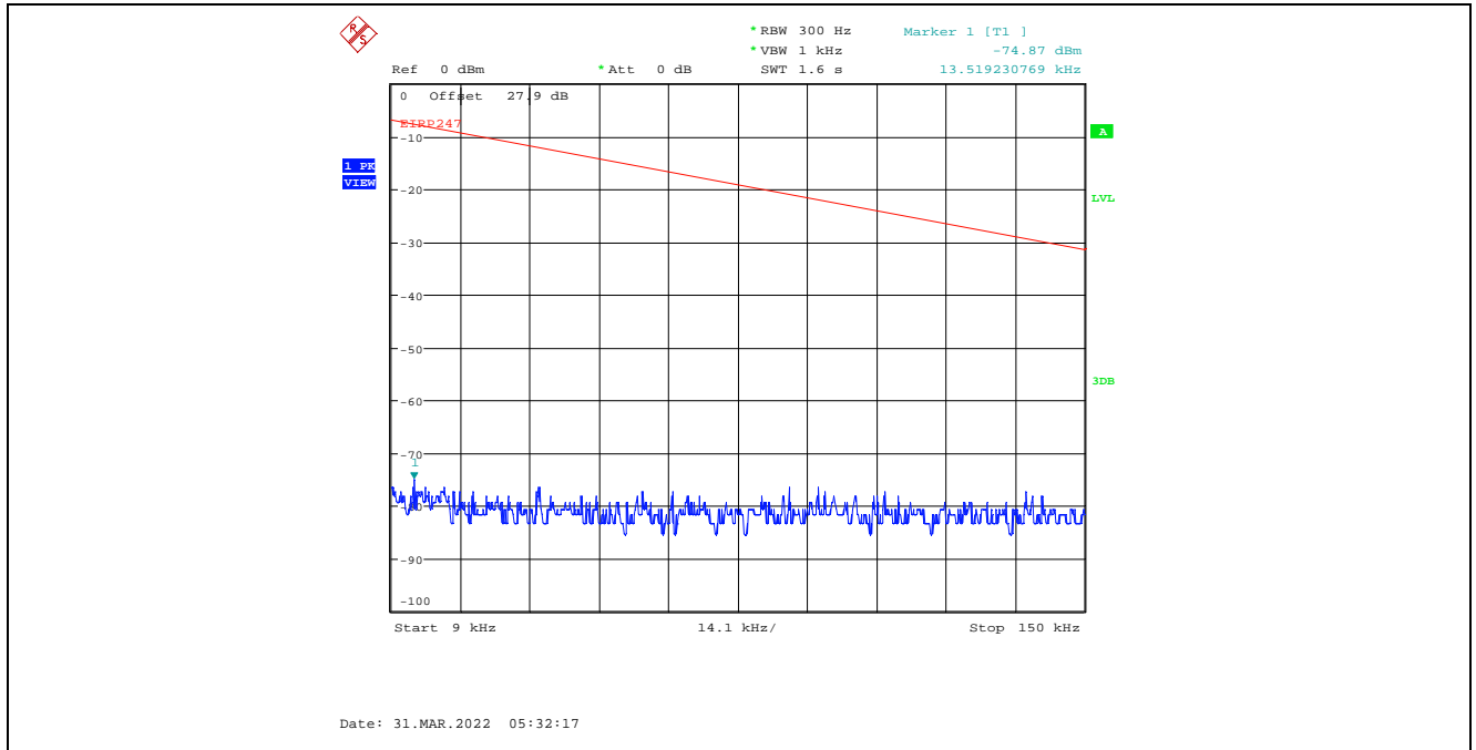
Plot C.4.111. Conducted Spurious Emissions in Restricted Frequency Bands, Chain 1 40 MHz Channel Bandwidth, Data Rate 7, Raw Power Setting 0, 2452 MHz, 9 kHz - 150 kHz, Peak Detector
