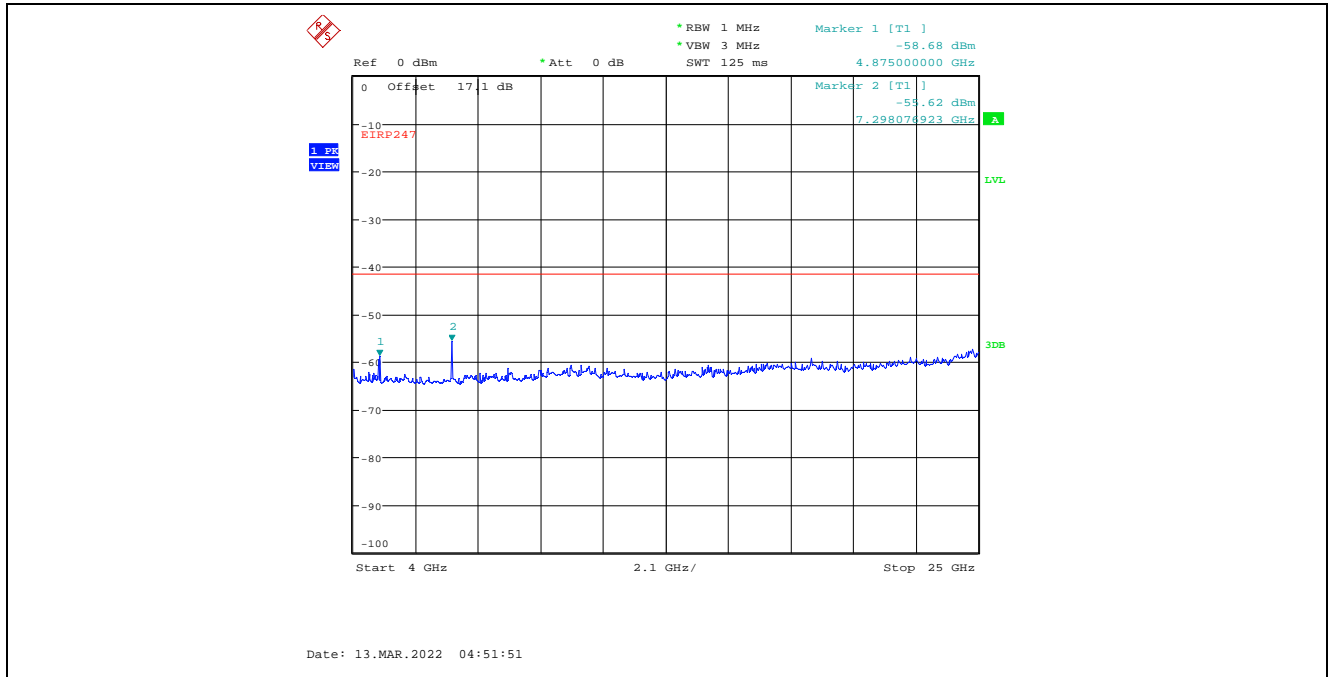
Plot C.2.80. Conducted Spurious Emissions in Restricted Frequency Bands, Chain 2 20 MHz Channel Bandwidth, Data Rate 7, Raw Power Setting 23, 2437 MHz, 4 GHz - 25 GHz, Peak Detector
