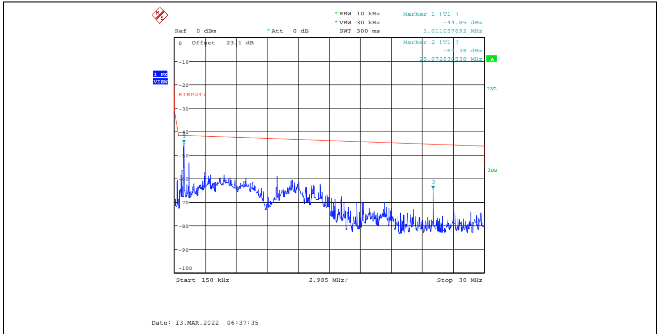
Plot C.2.84. Conducted Spurious Emissions in Restricted Frequency Bands, Chain 2 20 MHz Channel Bandwidth, Data Rate 7, Raw Power Setting 23, 2462 MHz, 150 kHz – 30 MHz, Peak Detector
