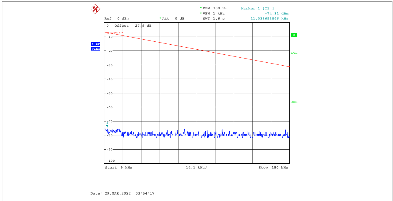
Plot C.3.71. Conducted Spurious Emissions in Restricted Frequency Bands, Chain 1 20 MHz Channel Bandwidth, Data Rate 3, Raw Power Setting 7, 2437 MHz, 9 kHz - 150 kHz, Peak Detector
