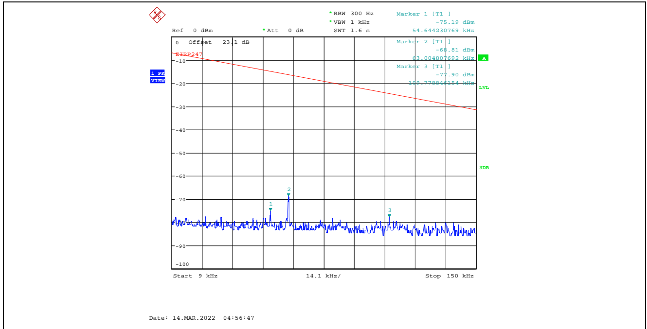
Plot C.2.52. Conducted Spurious Emissions in Restricted Frequency Bands, Chain 2 8 MHz Channel Bandwidth, Data Rate 7, Raw Power Setting 12, 2476 MHz, 9 kHz - 150 kHz, Peak Detector
