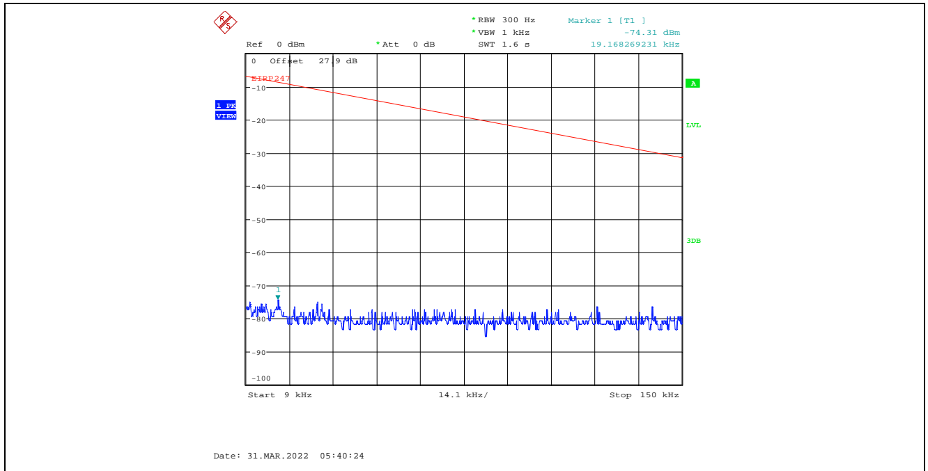
Plot C.4.112. Conducted Spurious Emissions in Restricted Frequency Bands, Chain 2 40 MHz Channel Bandwidth, Data Rate 7, Raw Power Setting 0, 2452 MHz, 9 kHz - 150 kHz, Peak Detector
