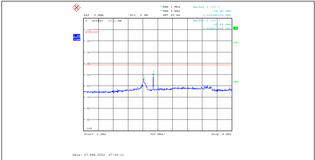
Plot C.1.38. Conducted Spurious Emissions in Restricted Frequency Bands, Chain 2 8 MHz Channel Bandwidth, Data Rate 3, Raw Power Setting 21, 2407 MHz, 1 GHz – 4 GHz, Peak Detector
