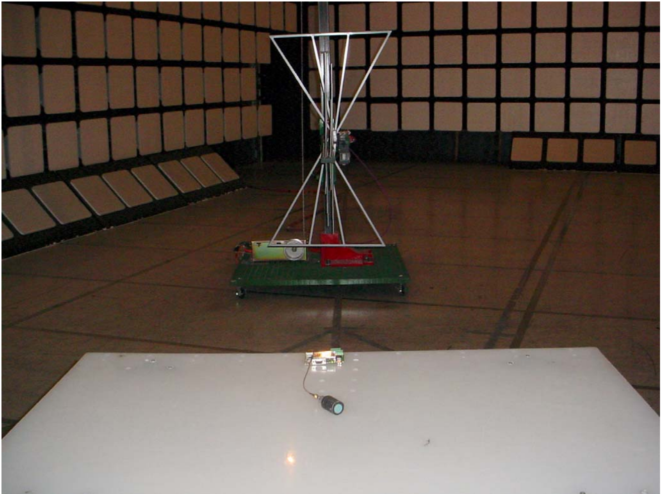
Radiated Emissions @ 3 m
