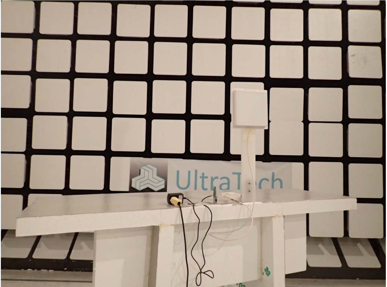
Radiated Emissions @ 3 m EUT with 8 dBi Patch Antenna, Orthogonal Position 3
