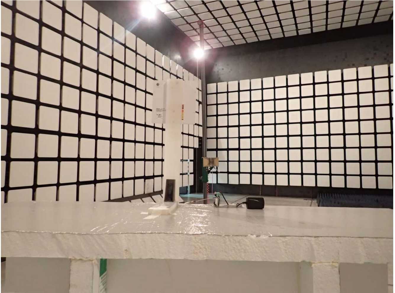
Radiated Emissions @ 3 m EUT with 8 dBi Patch Antenna, Orthogonal Position 2
