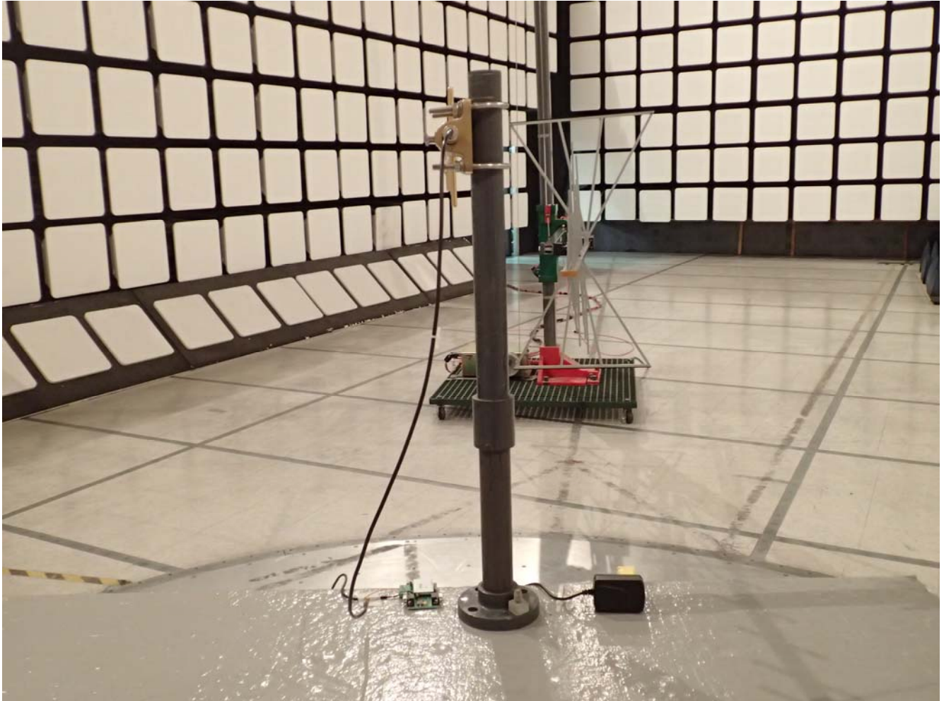
Radiated Emissions @ 3 m EUT with 13.15 dBi Yagi Antenna, Orthogonal Position 1
