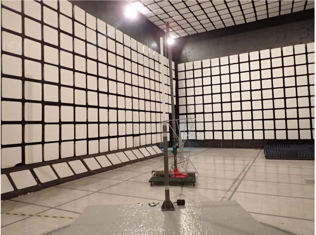
Radiated Emissions @ 3 m EUT with 8.15 dBi Omni Directional Antenna, Orthogonal Position 1
