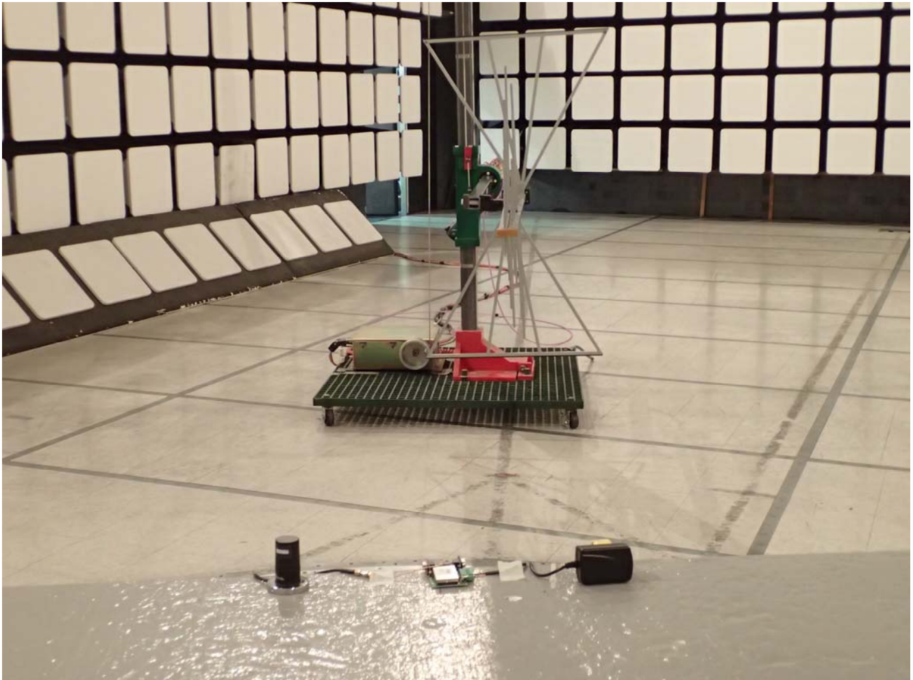
Radiated Emissions @ 3 m EUT with 4 dBi Puck Antenna, Orthogonal Position 1
