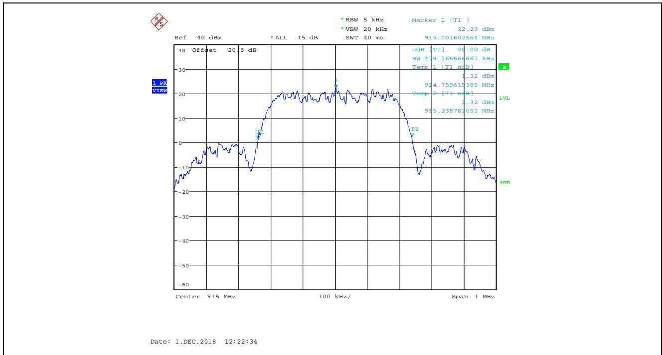
Plot 5.3.4.8. 20 dB Bandwidth, 915.0 MHz, High Data Rate, 500 kHz CS, High Power, Raw Power Setting at 10
