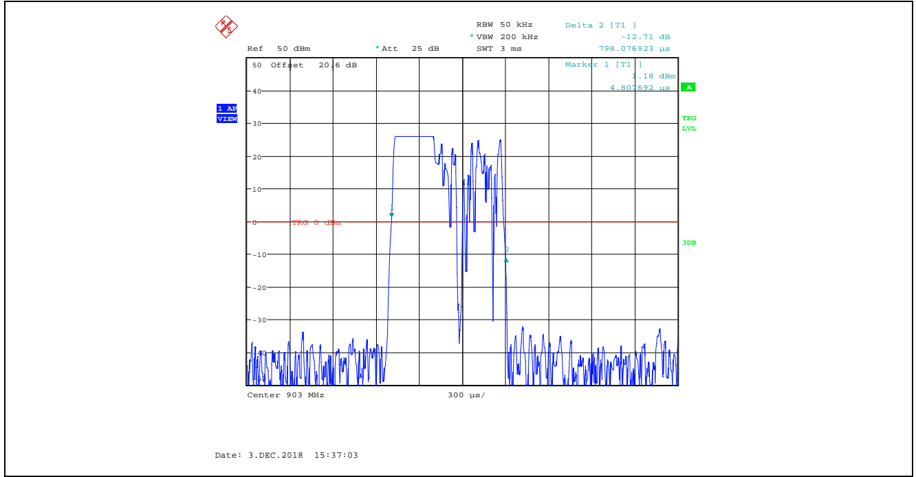
Plot 5.3.4.37. Time of Occupancy, 903.0 MHz, High Data Rate, 500 kHz CS Dwell Time at 903.0 MHz = 798.08 μs
