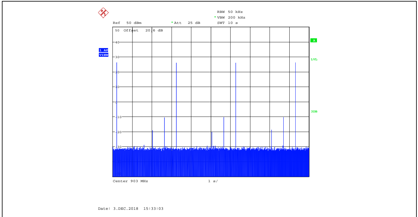
Plot 5.3.4.38. Time of Occupancy, 903.0 MHz, High Data Rate, 500 kHz CS Average time of occupancy = (Dwell Time) x (number of hops within a 10s period) = 798.08 μs x 4 = 3.19 ms
