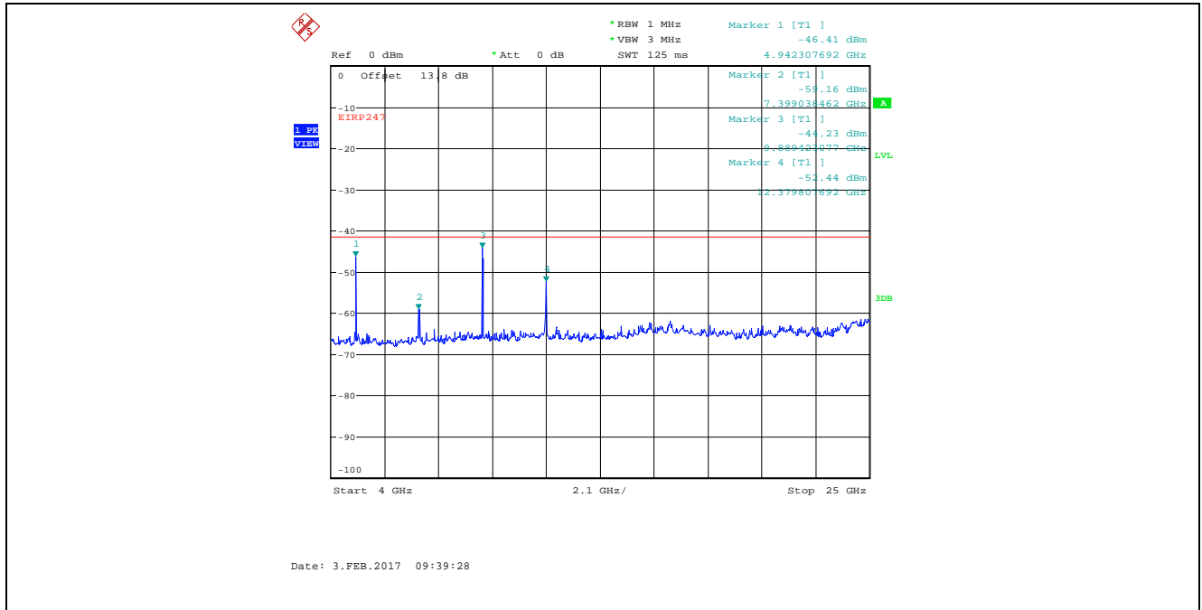
Plot 5.4.4.3.30. Conducted Spurious Emissions in Restricted Frequency Bands Bandwidth: 8 MHz, TX Gain Setting 55, Data Rate 4, 2477 MHz, 4 GHz - 25 GHz, Peak Detector
