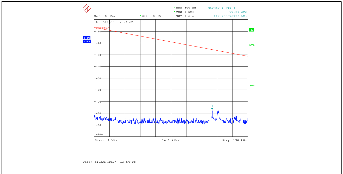
Plot 5.4.4.16. Conducted Spurious Emissions in Restricted Frequency Bands Bandwidth: 8 MHz, TX Gain Setting 25, Data Rate 4, 2407 MHz, 9 kHz - 150 kHz, Peak Detector
