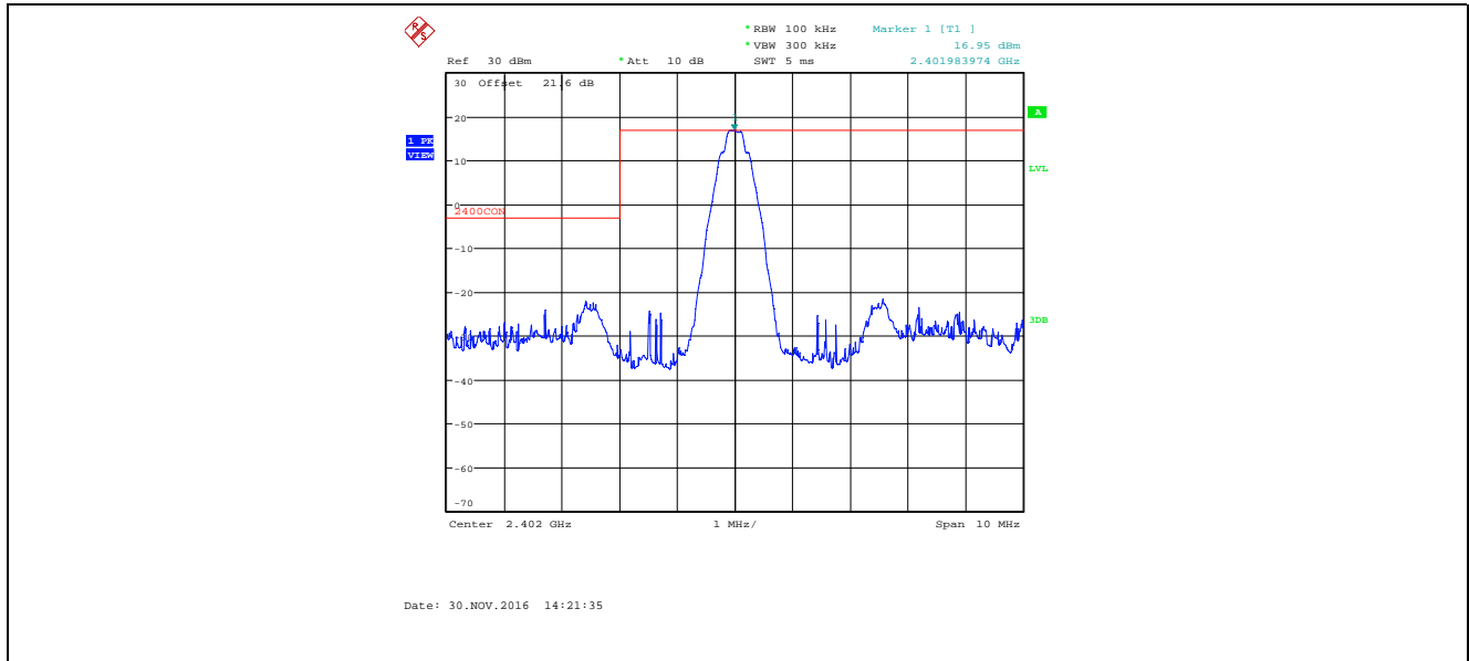
Plot 5.4.4.1.1. Band-Edge RF Conducted Emissions Bandwidth: 1 MHz, TX Gain Setting: 26, Data Rate 2, 2402 MHz, Lower Band-edge
