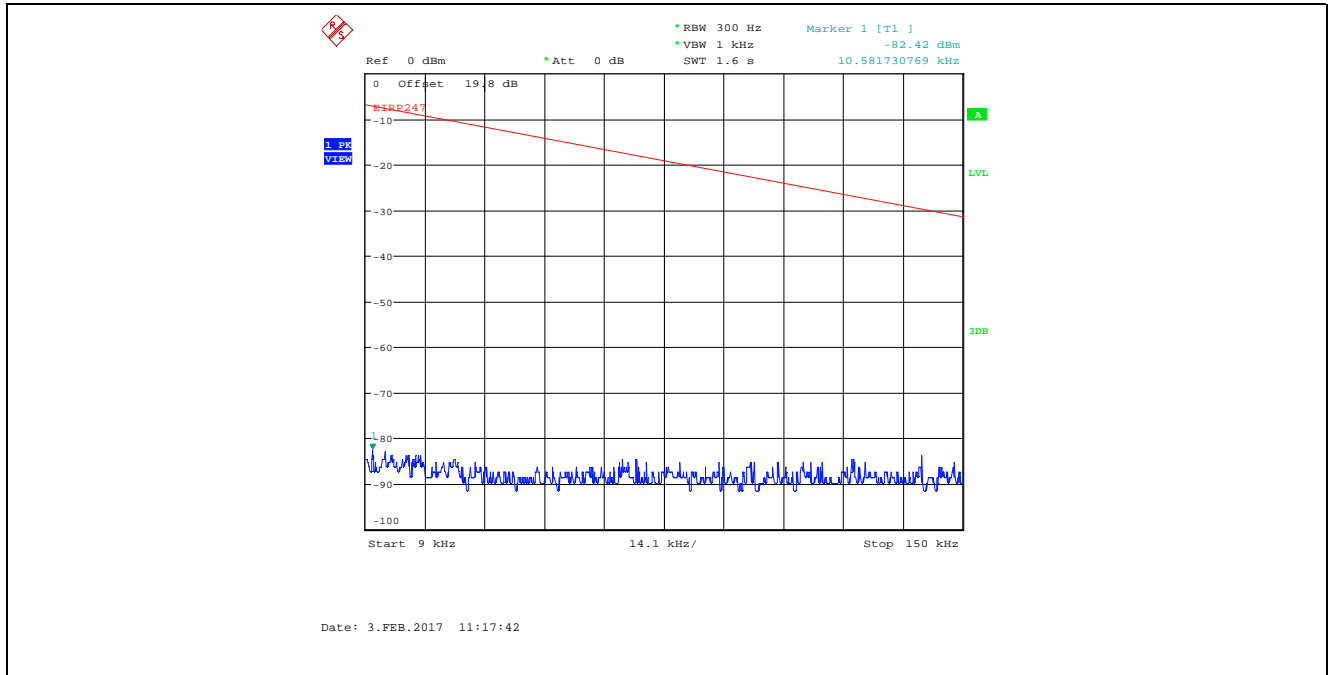
Plot 5.4.4.3.6. Conducted Spurious Emissions in Restricted Frequency Bands Bandwidth: 8 MHz, TX Gain Setting 50, Data Rate 1, 2442 MHz, 9 kHz - 150 kHz, Peak Detector
