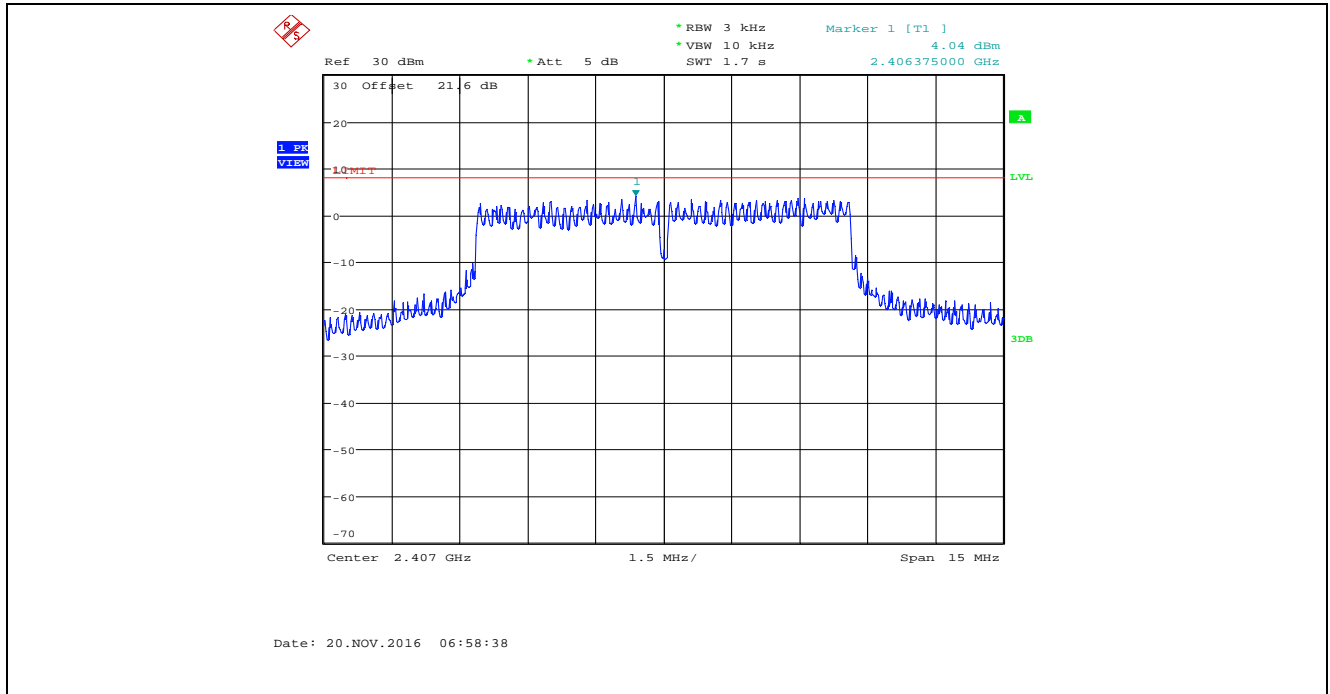
Plot 5.6.4.73. Power Spectral Density, Bandwidth: 8 MHz, TX Gain Setting: 55, Data Rate 5, 2407 MHz
