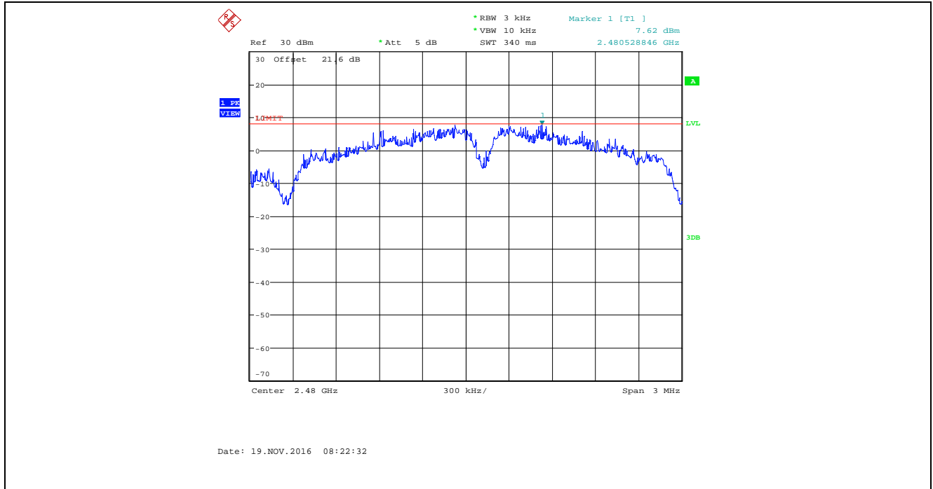
Plot 5.6.4.21. Power Spectral Density, Bandwidth: 4 MHz, TX Gain Setting: 43, Data Rate 2, 2480 MHz
