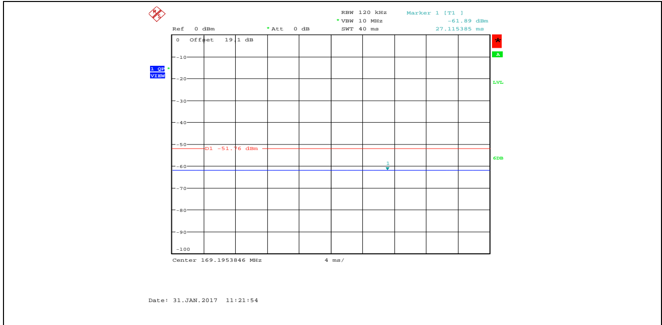
Plot 5.4.4.27. Conducted Spurious Emissions in Restricted Frequency Bands Bandwidth: 8 MHz, TX Gain Setting 25, Data Rate 4, 2442 MHz, RB 167.72-173.2 MHz, QP Detector QP at 169.19 MHz (RB 167.72-173.2 MHz) is -61.89dBm (limit -51.76dBm)
