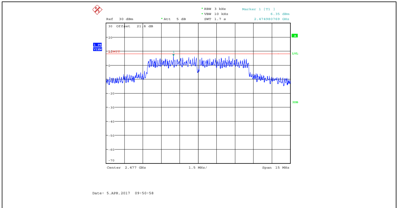
Plot 5.6.4.81. Power Spectral Density, Bandwidth: 8 MHz, TX Gain Setting: 55, Data Rate 7, 2477 MHz
