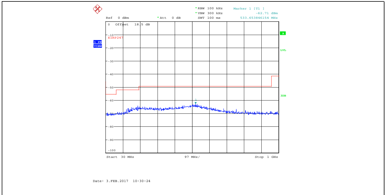
Plot 5.4.4.3.8. Conducted Spurious Emissions in Restricted Frequency Bands Bandwidth: 8 MHz, TX Gain Setting 50, Data Rate 1, 2442 MHz, 30 MHz - 1 GHz, Peak Detector
