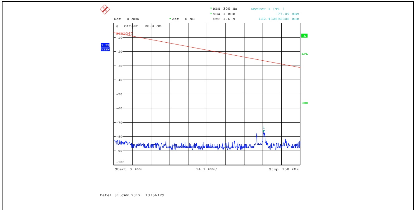
Plot 5.4.4.30. Conducted Spurious Emissions in Restricted Frequency Bands Bandwidth: 8 MHz, TX Gain Setting 25, Data Rate 4, 2477 MHz, 9 kHz - 150 kHz, Peak Detector
