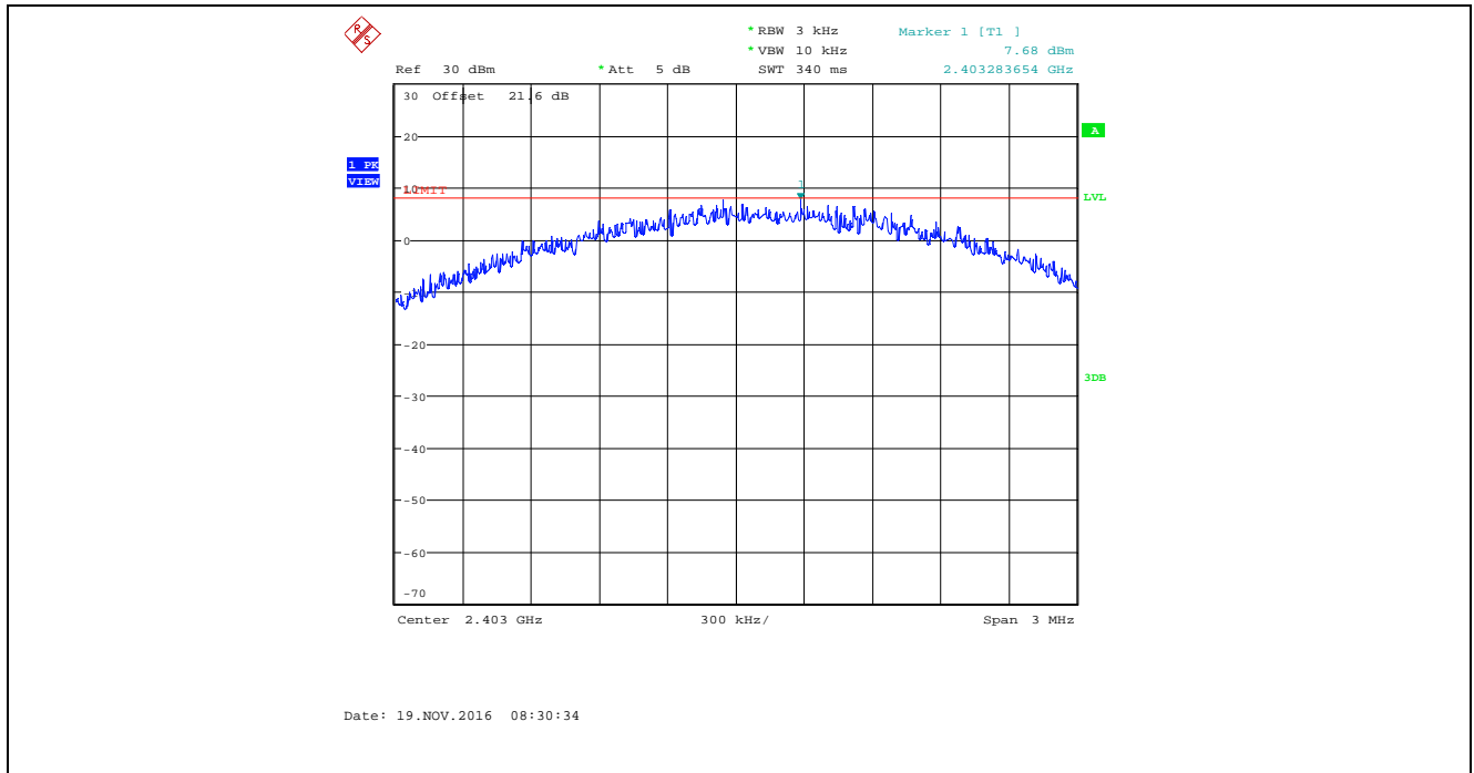
Plot 5.6.4.22. Power Spectral Density, Bandwidth: 4 MHz, TX Gain Setting: 43, Data Rate 3, 2403 MHz
