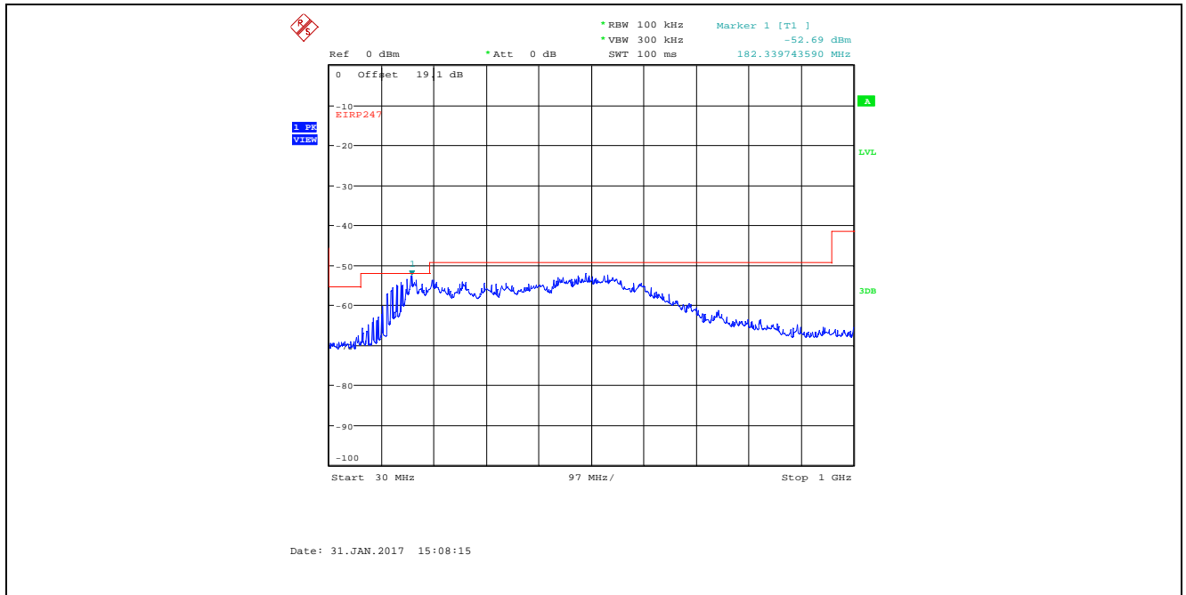
Plot 5.4.4.13. Conducted Spurious Emissions in Restricted Frequency Bands Bandwidth: 8 MHz, TX Gain Setting 25, Data Rate 1, 2477 MHz, 30 MHz - 1 GHz, Peak Detector
