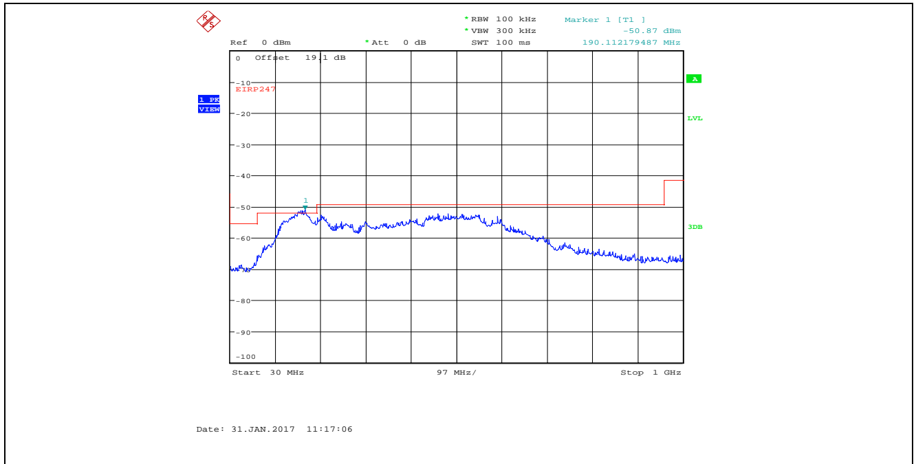
Plot 5.4.4.25. Conducted Spurious Emissions in Restricted Frequency Bands Bandwidth: 8 MHz, TX Gain Setting 25, Data Rate 4, 2442 MHz, 30 MHz - 1 GHz, Peak Detector
