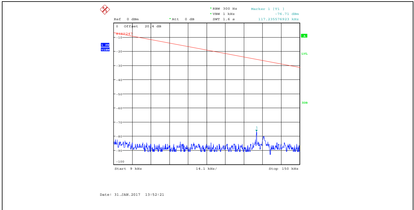
Plot 5.4.4.23. Conducted Spurious Emissions in Restricted Frequency Bands Bandwidth: 8 MHz, TX Gain Setting 25, Data Rate 4, 2442 MHz, 9 kHz - 150 kHz, Peak Detector
