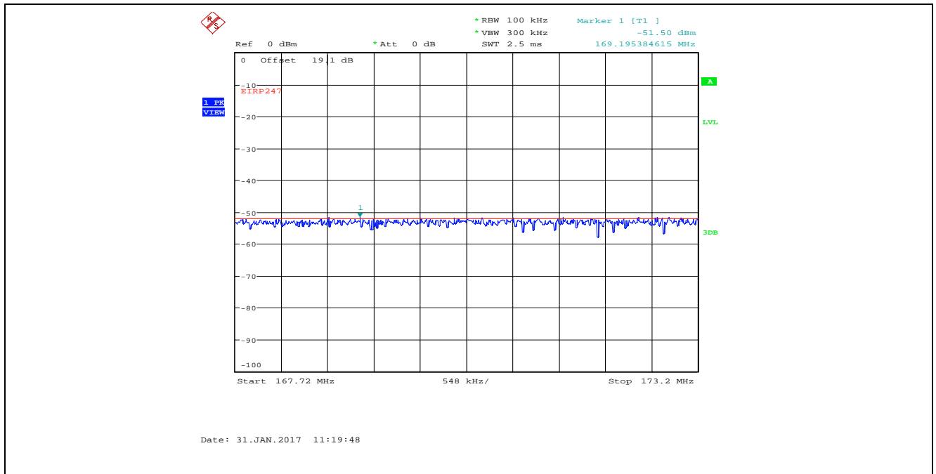
Plot 5.4.4.26. Conducted Spurious Emissions in Restricted Frequency Bands Bandwidth: 8 MHz, TX Gain Setting 25, Data Rate 4, 2442 MHz, RB 167.72-173.2 MHz, QP Detector
