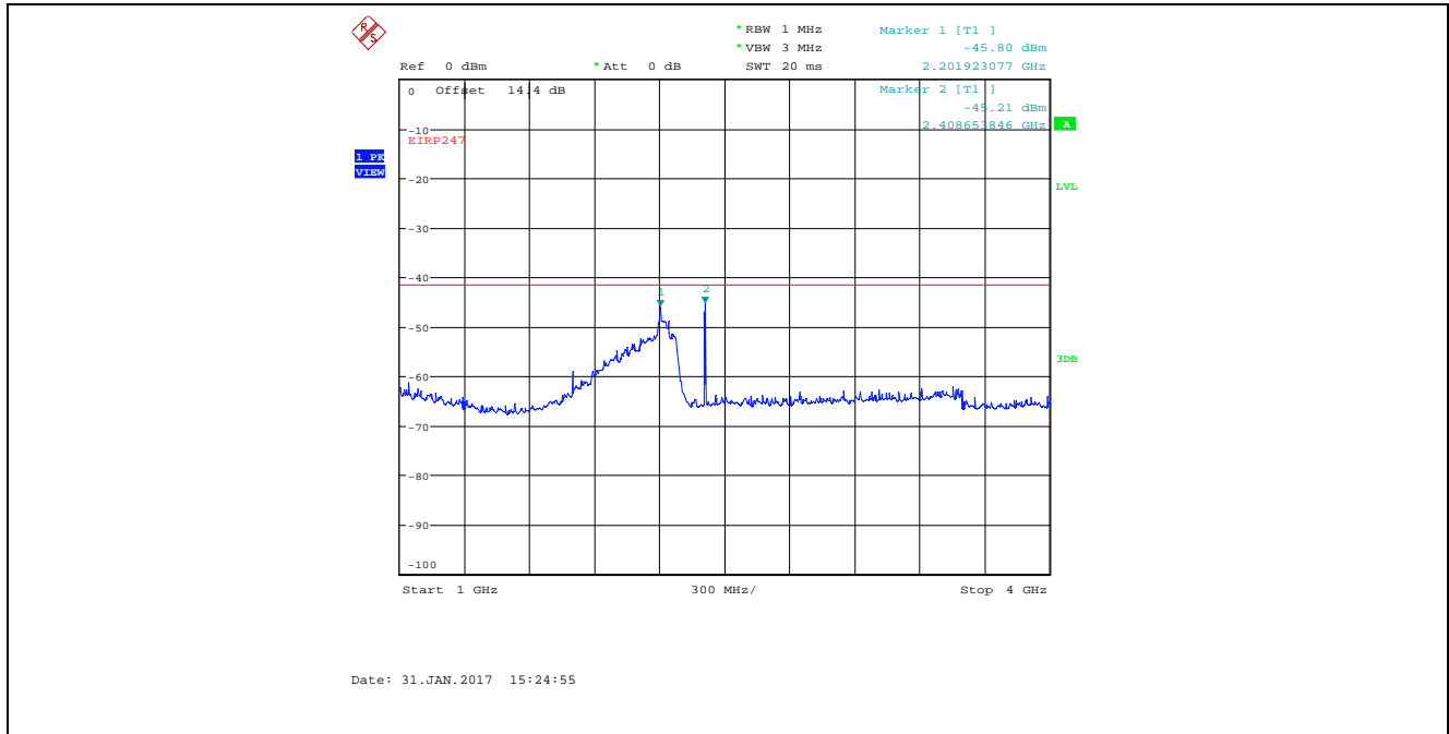
Plot 5.4.4.4. Conducted Spurious Emissions in Restricted Frequency Bands Bandwidth: 8 MHz, TX Gain Setting 25, Data Rate 1, 2407 MHz, 1 GHz - 4 GHz, Peak Detector
