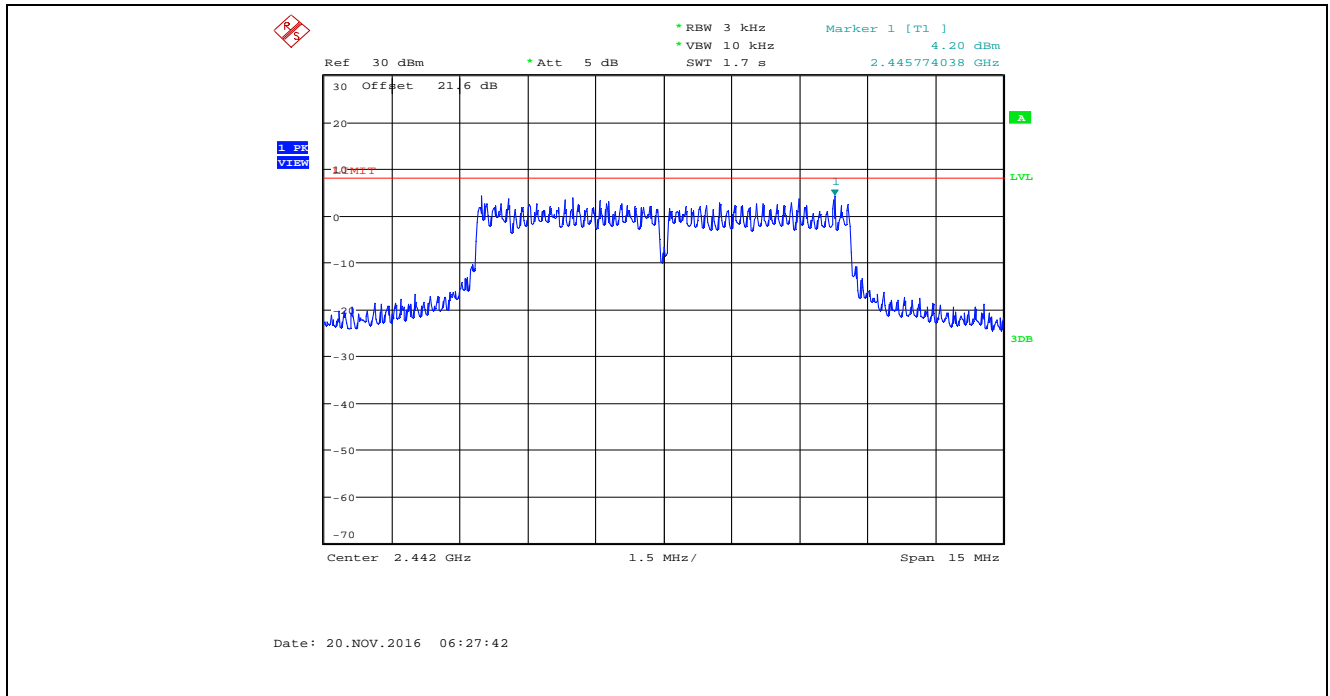
Plot 5.6.4.80. Power Spectral Density, Bandwidth: 8 MHz, TX Gain Setting: 55, Data Rate 7, 2442 MHz
