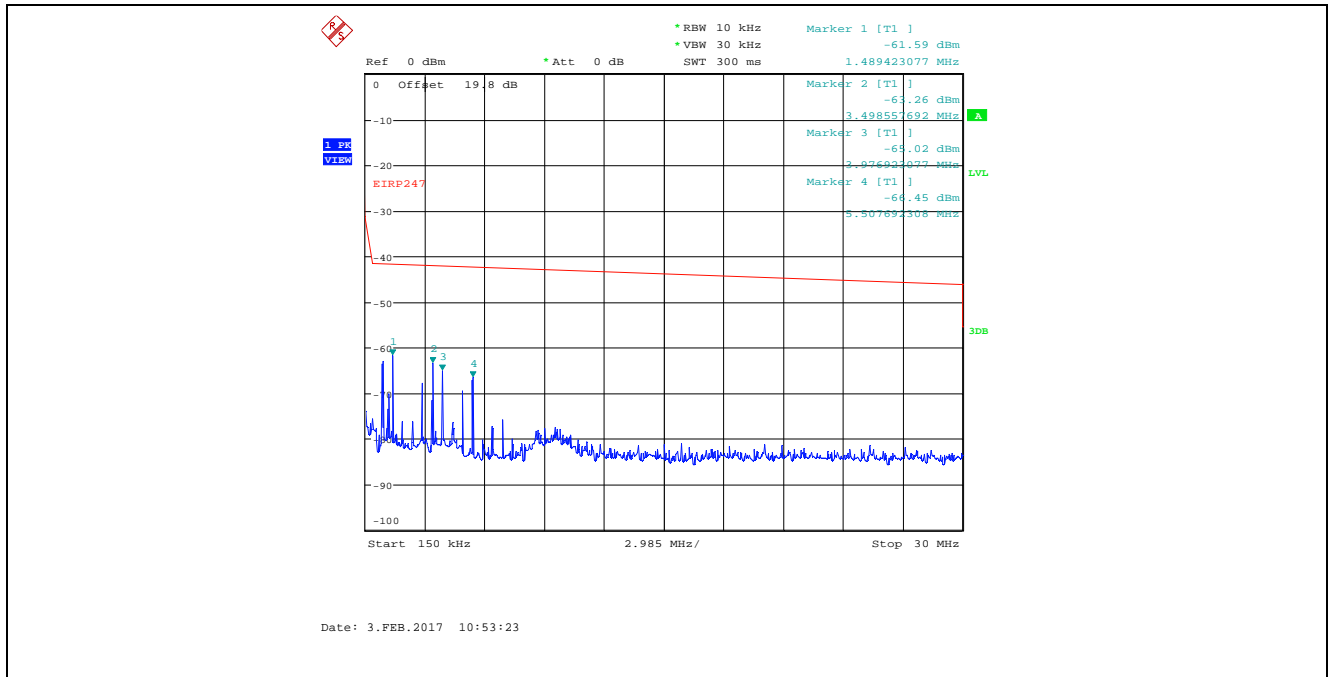
Plot 5.4.4.3.7. Conducted Spurious Emissions in Restricted Frequency Bands Bandwidth: 8 MHz, TX Gain Setting 50, Data Rate 1, 2442 MHz, 150 kHz - 30 MHz, Peak Detector
