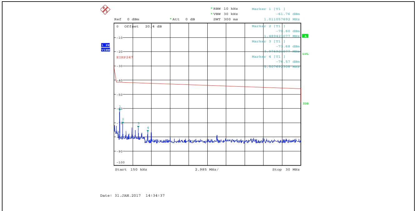
Plot 5.4.4.7. Conducted Spurious Emissions in Restricted Frequency Bands Bandwidth: 8 MHz, TX Gain Setting 25, Data Rate 1, 2442 MHz, 150 kHz - 30 MHz, Peak Detector
