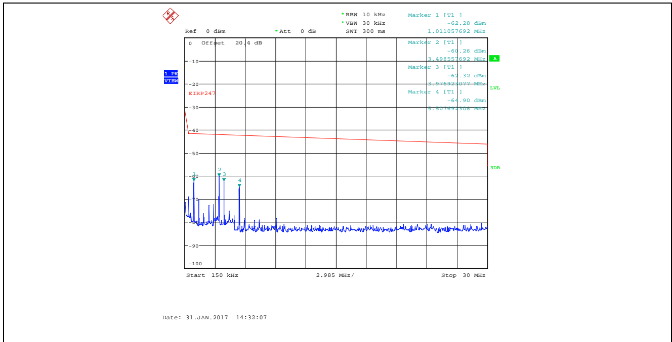
Plot 5.4.4.12. Conducted Spurious Emissions in Restricted Frequency Bands Bandwidth: 8 MHz, TX Gain Setting 25, Data Rate 1, 2477 MHz, 150 kHz - 30 MHz, Peak Detector
