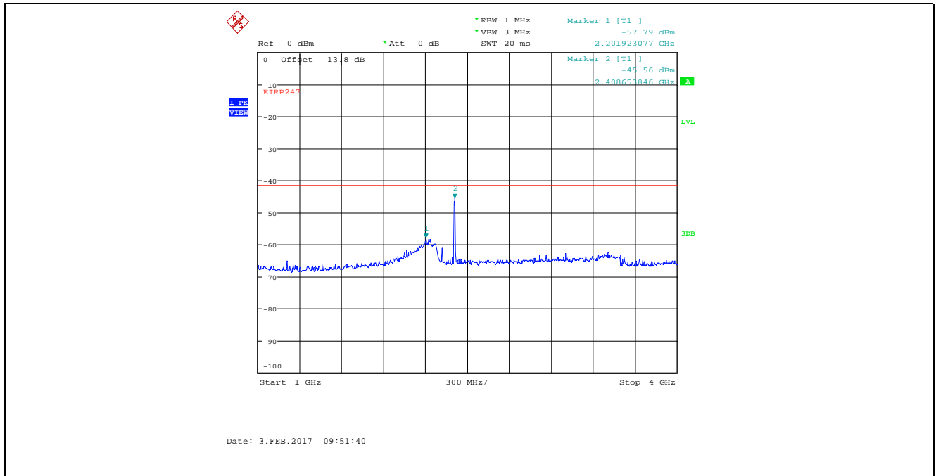
Plot 5.4.4.3.19. Conducted Spurious Emissions in Restricted Frequency Bands Bandwidth: 8 MHz, TX Gain Setting 55, Data Rate 4, 2407 MHz, 1 GHz - 4 GHz, Peak Detector
