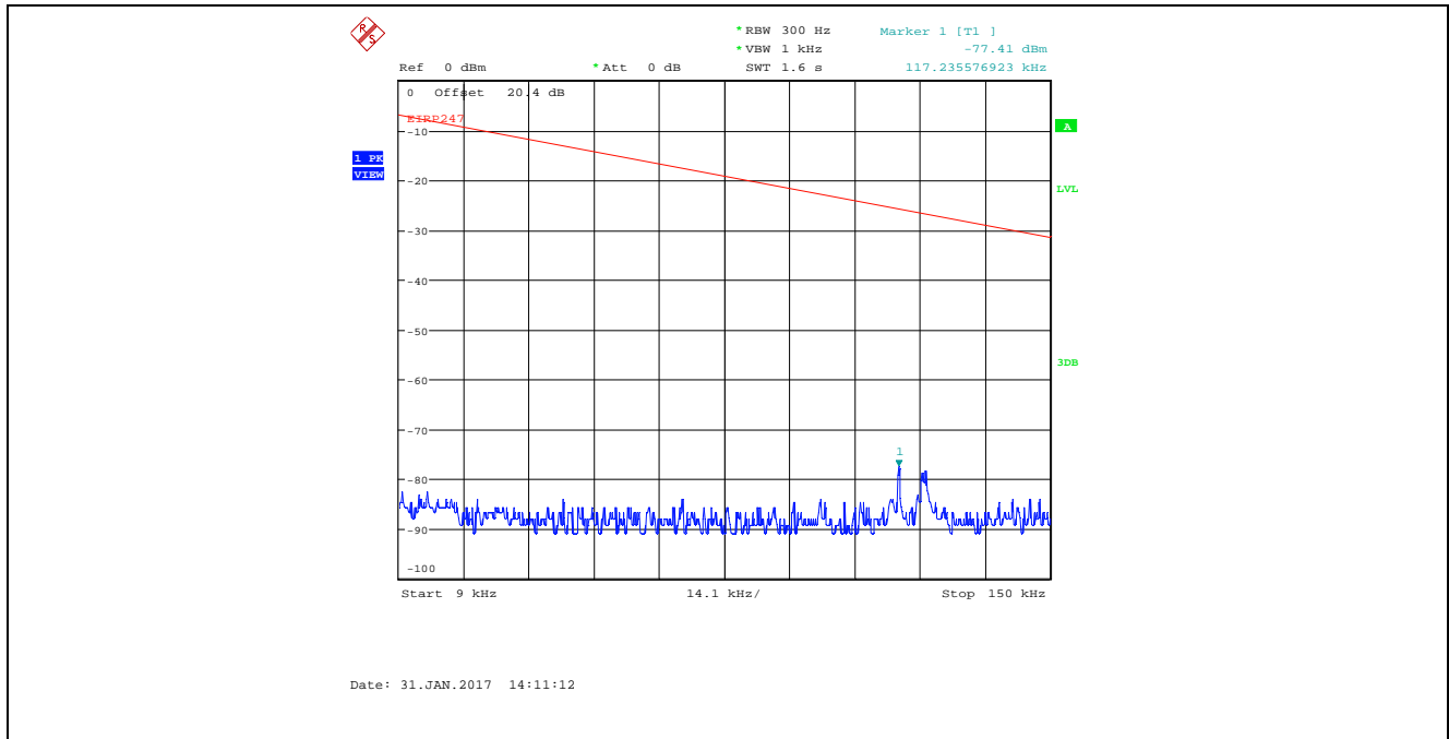
Plot 5.4.4.11. Conducted Spurious Emissions in Restricted Frequency Bands Bandwidth: 8 MHz, TX Gain Setting 25, Data Rate 1, 2477 MHz, 9 kHz - 150 kHz, Peak Detector
