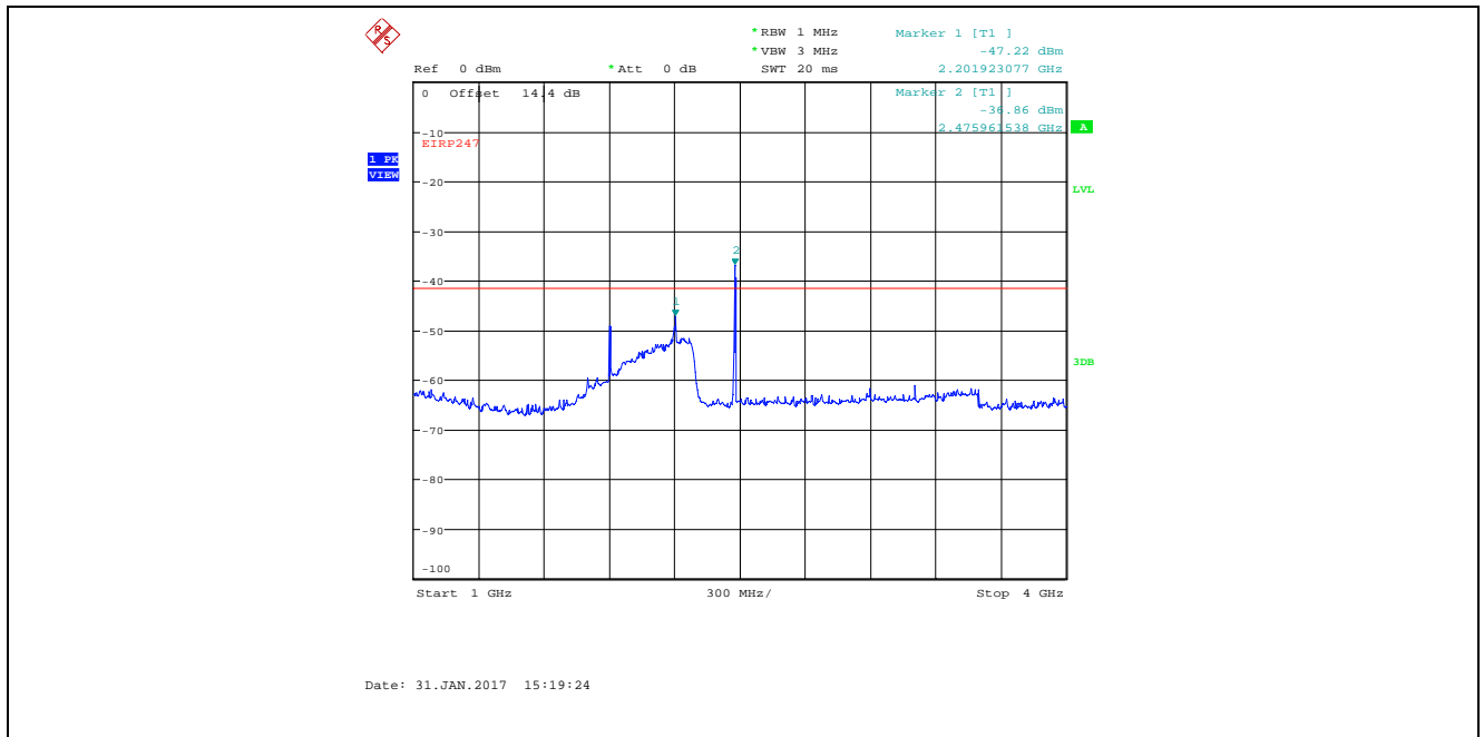
Plot 5.4.4.14. Conducted Spurious Emissions in Restricted Frequency Bands Bandwidth: 8 MHz, TX Gain Setting 25, Data Rate 1, 2477 MHz, 1 GHz - 4 GHz, Peak Detector Marker 2 is the Fundamental
