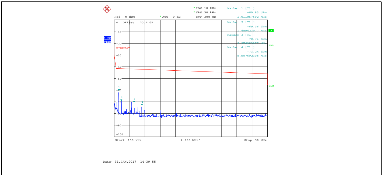
Plot 5.4.4.4.2. Conducted Spurious Emissions in Restricted Frequency Bands Bandwidth: 8 MHz, TX Gain Setting 25, Data Rate 1, 2407 MHz, 150 kHz - 30 MHz, Peak Detector
