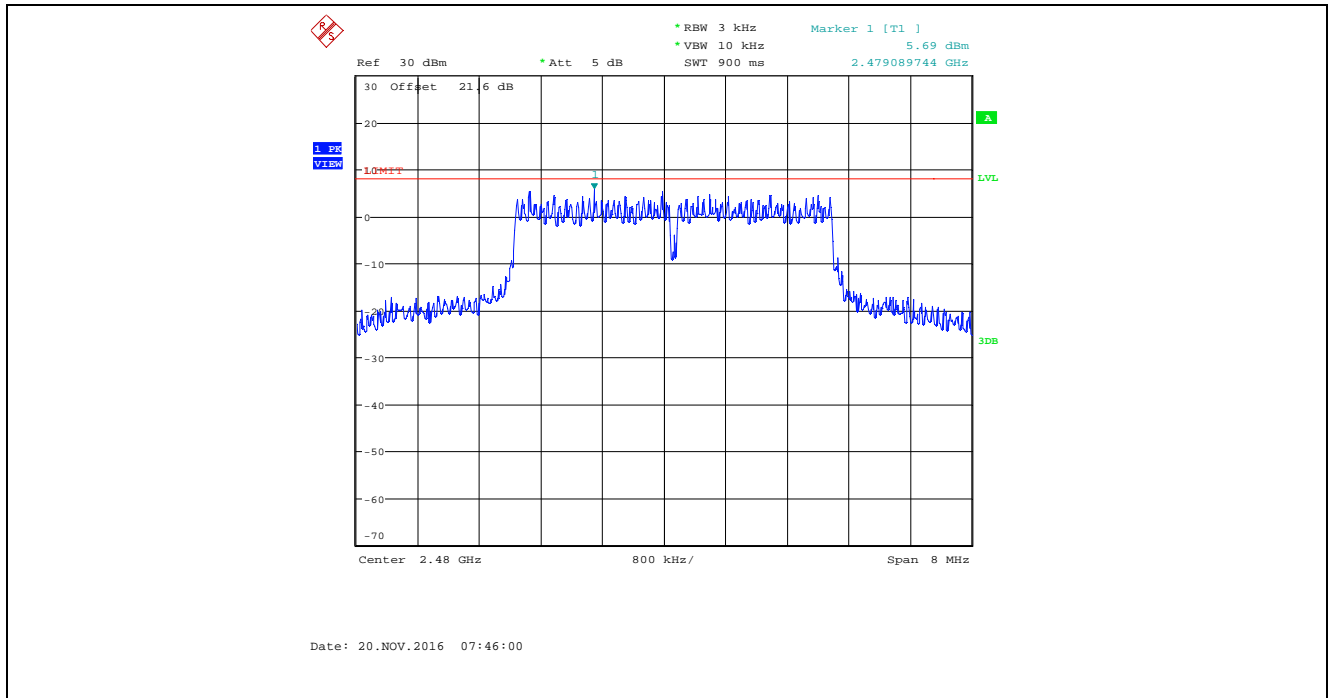
Plot 5.6.4.60. Power Spectral Density, Bandwidth: 4 MHz, TX Gain Setting: 50, Data Rate 4, 2480 MHz
