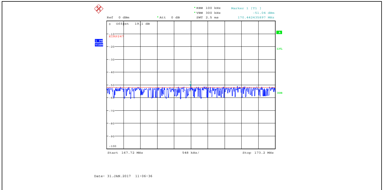
Plot 5.4.4.19. Conducted Spurious Emissions in Restricted Frequency Bands Bandwidth: 8 MHz, TX Gain Setting 25, Data Rate 4, 2407 MHz, RB 167.72-173.2 MHz, QP Detector
