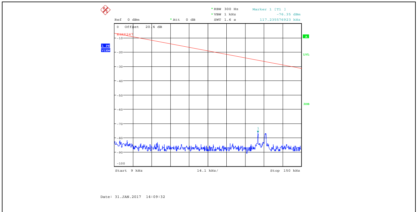
Plot 5.4.4.4.6. Conducted Spurious Emissions in Restricted Frequency Bands Bandwidth: 8 MHz, TX Gain Setting 25, Data Rate 1, 2442 MHz, 9 kHz - 150 kHz, Peak Detector
