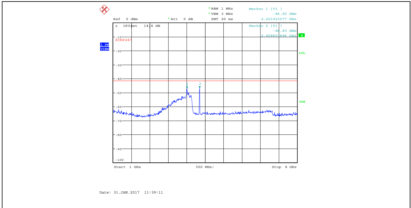
Plot 5.4.4.21. Conducted Spurious Emissions in Restricted Frequency Bands Bandwidth: 8 MHz, TX Gain Setting 25, Data Rate 4, 2407 MHz, 1 GHz - 4 GHz, Peak Detector
