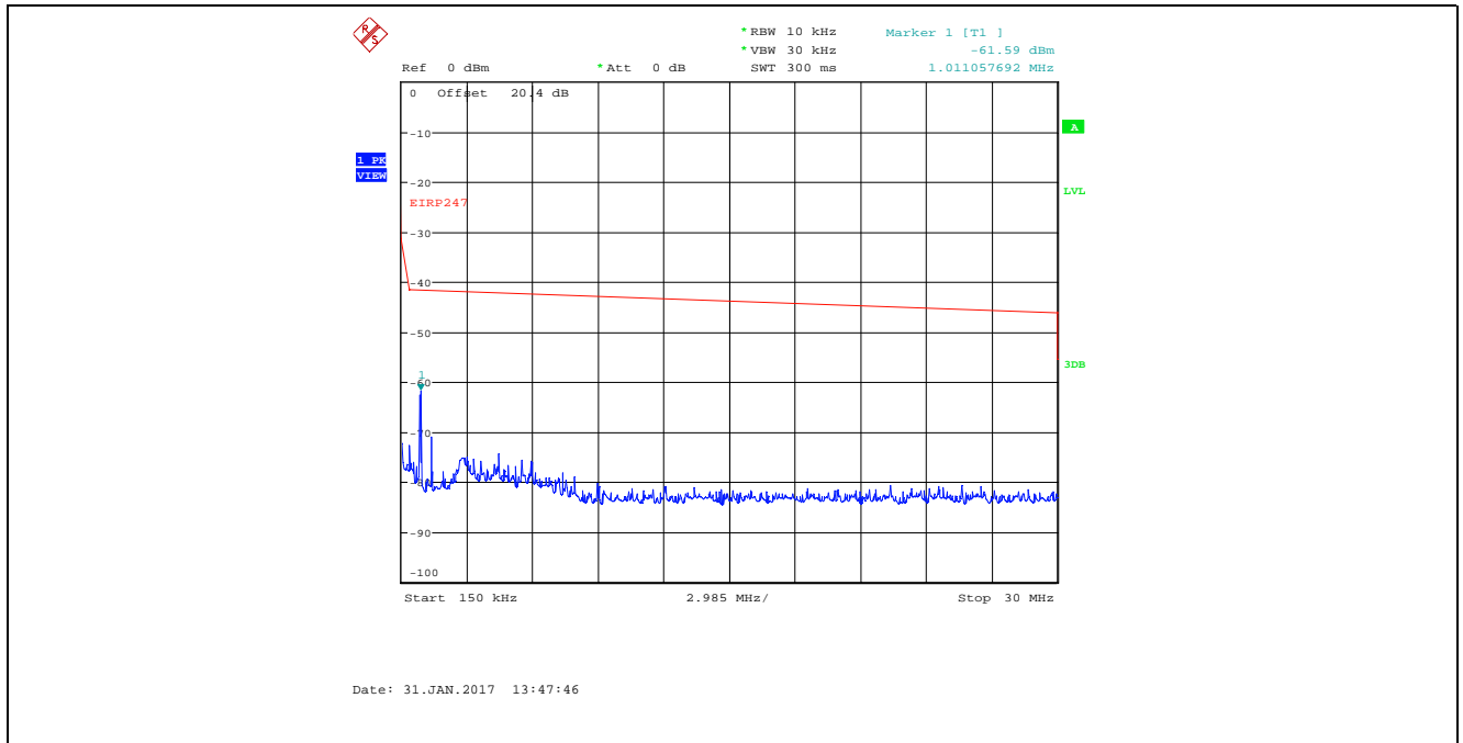
Plot 5.4.4.31. Conducted Spurious Emissions in Restricted Frequency Bands Bandwidth: 8 MHz, TX Gain Setting 25, Data Rate 4, 2477 MHz, 150 kHz - 30 MHz, Peak Detector
