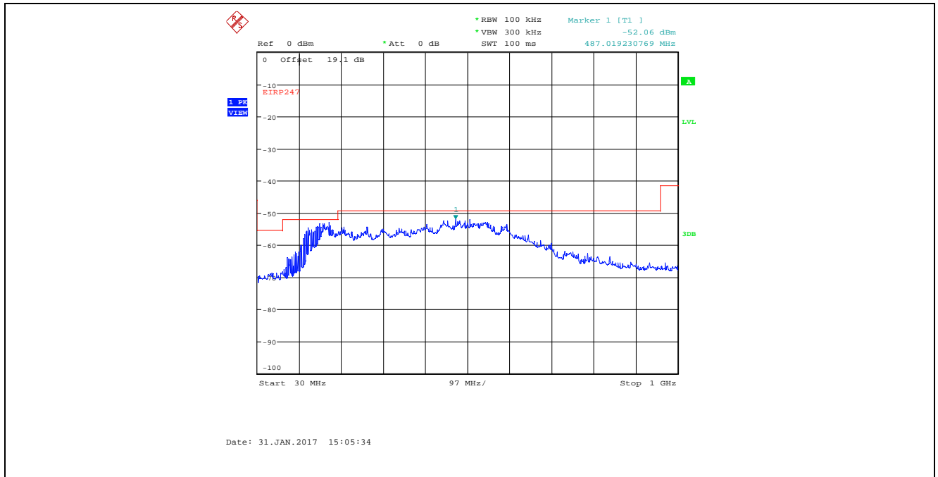
Plot 5.4.4.8. Conducted Spurious Emissions in Restricted Frequency Bands Bandwidth: 8 MHz, TX Gain Setting 25, Data Rate 1, 2442 MHz, 30 MHz - 1 GHz, Peak Detector
