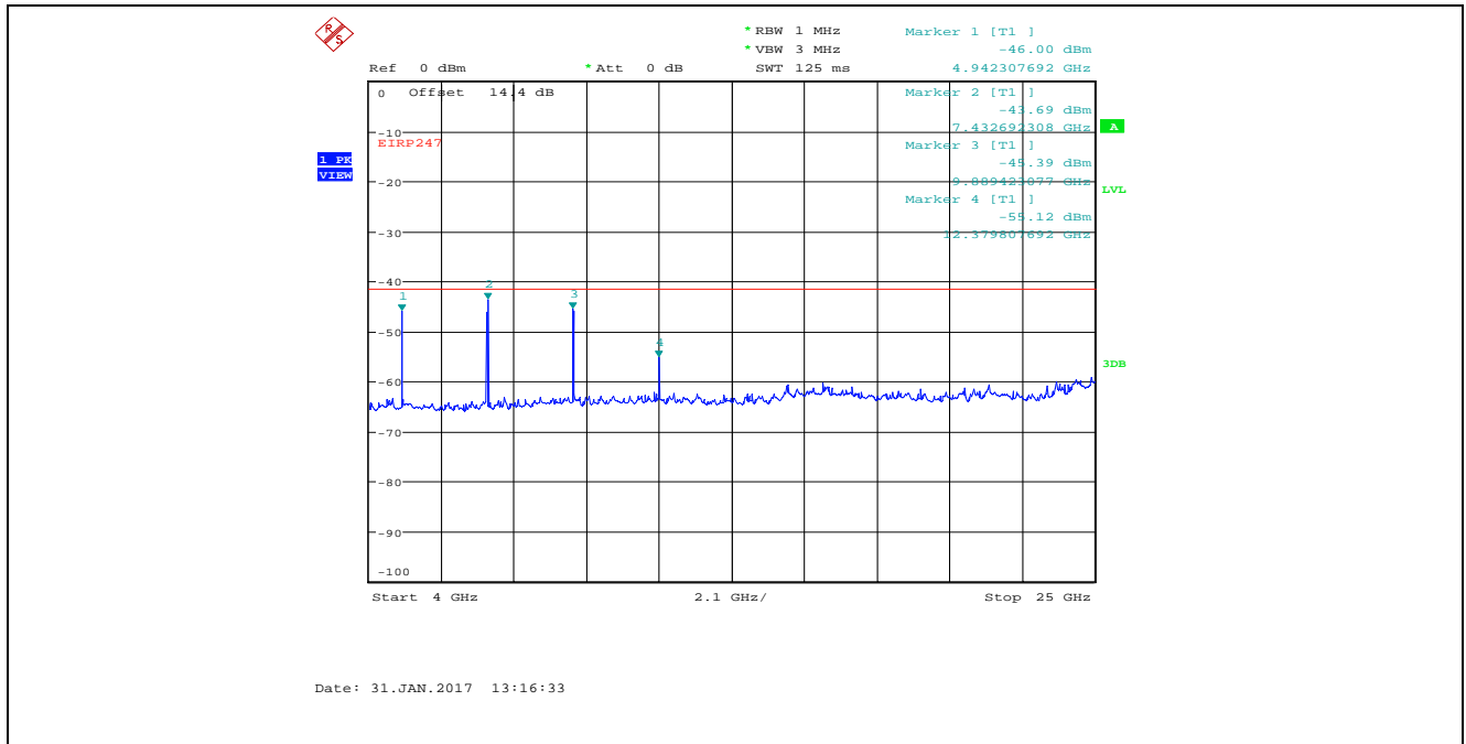
Plot 5.4.4.35. Conducted Spurious Emissions in Restricted Frequency Bands Bandwidth: 8 MHz, TX Gain Setting 25, Data Rate 4, 2477 MHz, 4 GHz - 25 GHz, Peak Detector
