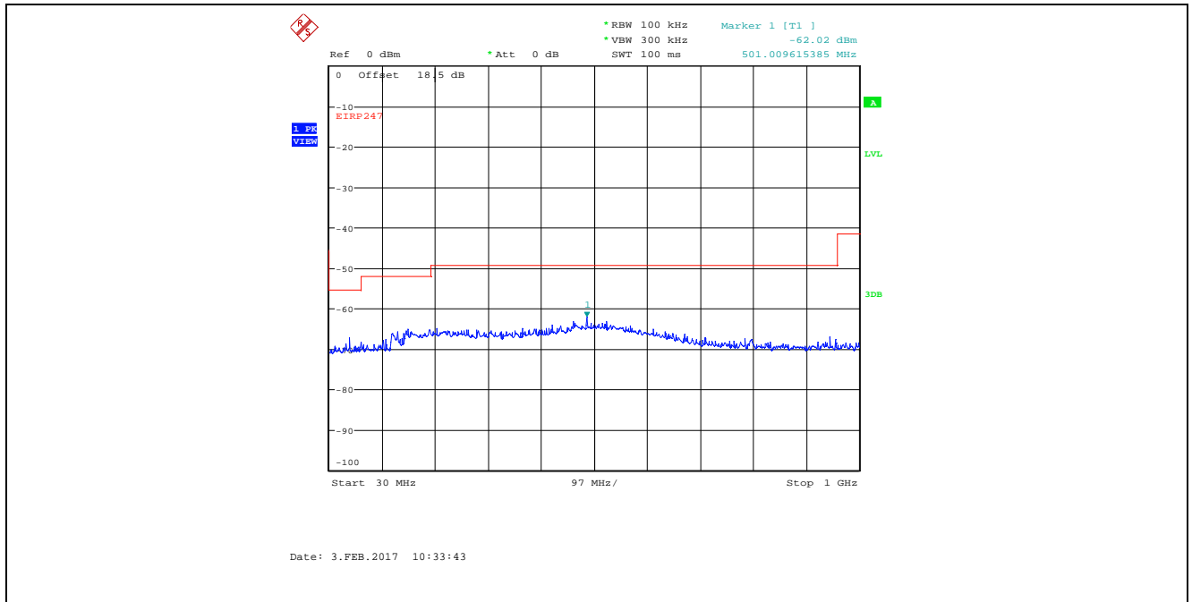
Plot 5.4.4.3.3. Conducted Spurious Emissions in Restricted Frequency Bands Bandwidth: 8 MHz, TX Gain Setting 50, Data Rate 1, 2407 MHz, 30 MHz - 1 GHz, Peak Detector
