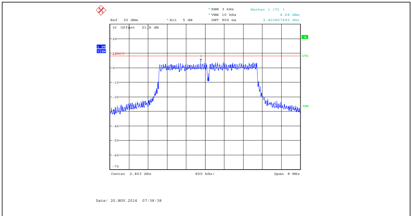
Plot 5.6.4.61. Power Spectral Density, Bandwidth: 4 MHz, TX Gain Setting: 50, Data Rate 5, 2403 MHz
