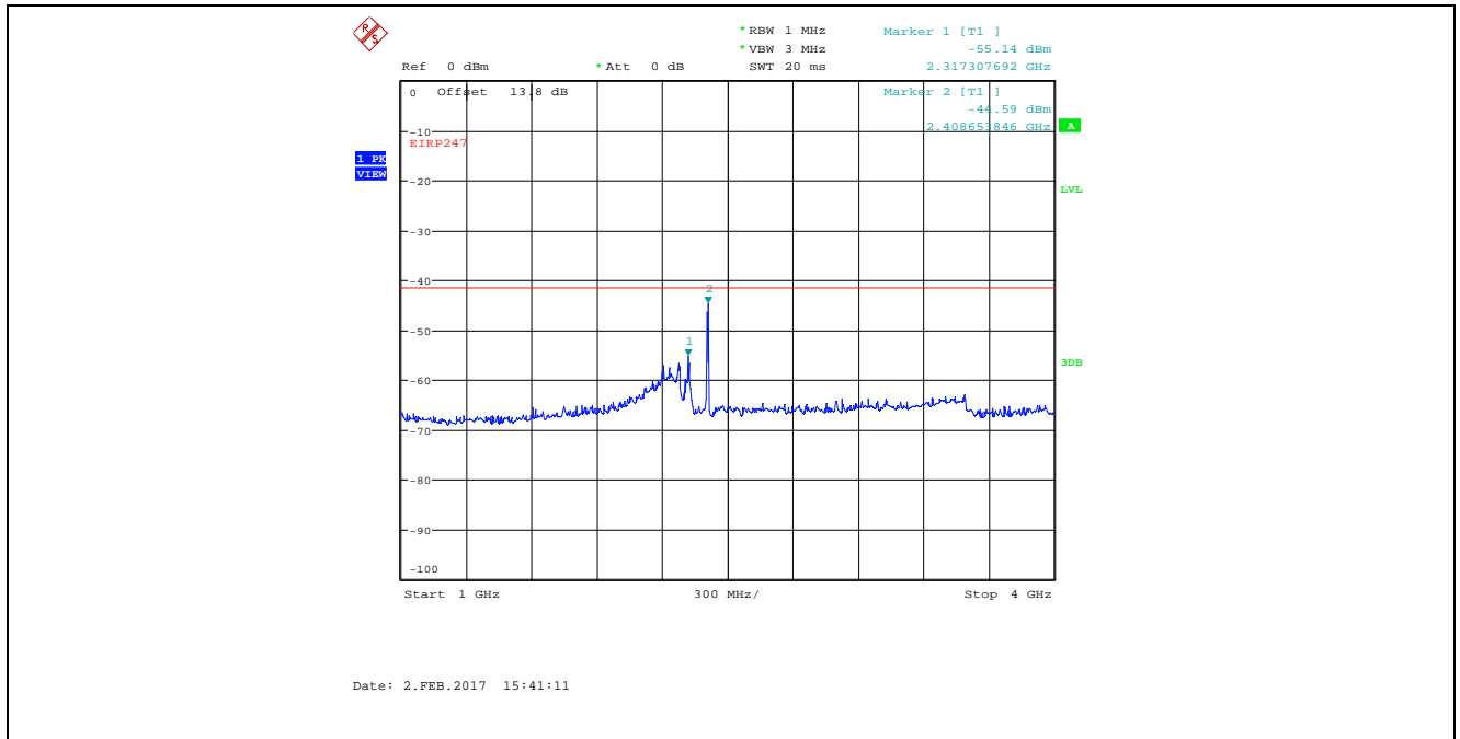
Plot 5.4.4.3.4. Conducted Spurious Emissions in Restricted Frequency Bands Bandwidth: 8 MHz, TX Gain Setting 50, Data Rate 1, 2407 MHz, 1 GHz - 4 GHz, Peak Detector
