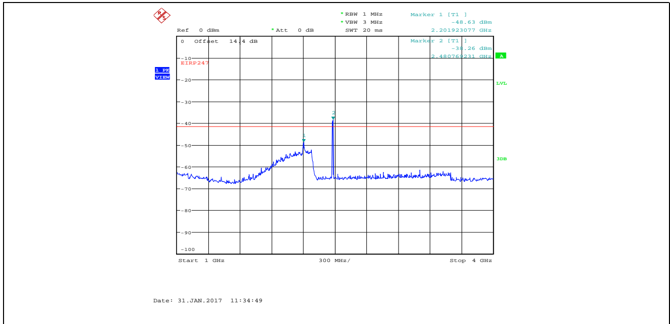
Plot 5.4.4.34. Conducted Spurious Emissions in Restricted Frequency Bands Bandwidth: 8 MHz, TX Gain Setting 25, Data Rate 4, 2477 MHz, 1 GHz - 4 GHz, Peak Detector Marker 2 is the Fundamental
