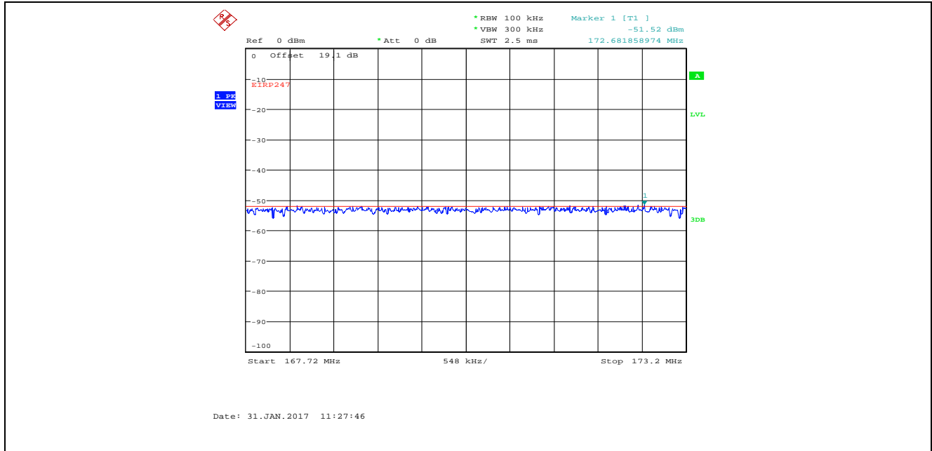
Plot 5.4.4.33. Conducted Spurious Emissions in Restricted Frequency Bands Bandwidth: 8 MHz, TX Gain Setting 25, Data Rate 4, 2477 MHz, RB 167.72-173.2 MHz, QP Detector QP at 172.68 MHz is -61.67dBm (limit -51.76 dBm)
