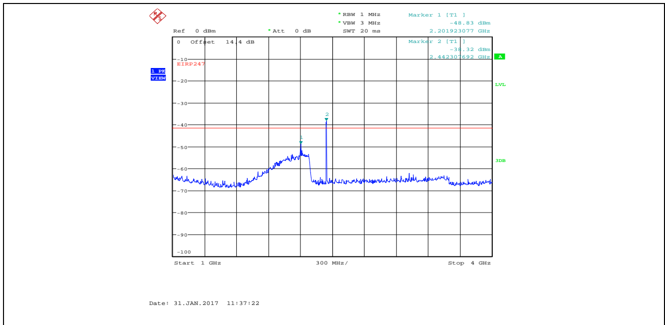
Plot 5.4.4.28. Conducted Spurious Emissions in Restricted Frequency Bands Bandwidth: 8 MHz, TX Gain Setting 25, Data Rate 4, 2442 MHz, 1 GHz - 4 GHz, Peak Detector Marker 2 is the Fundamental
