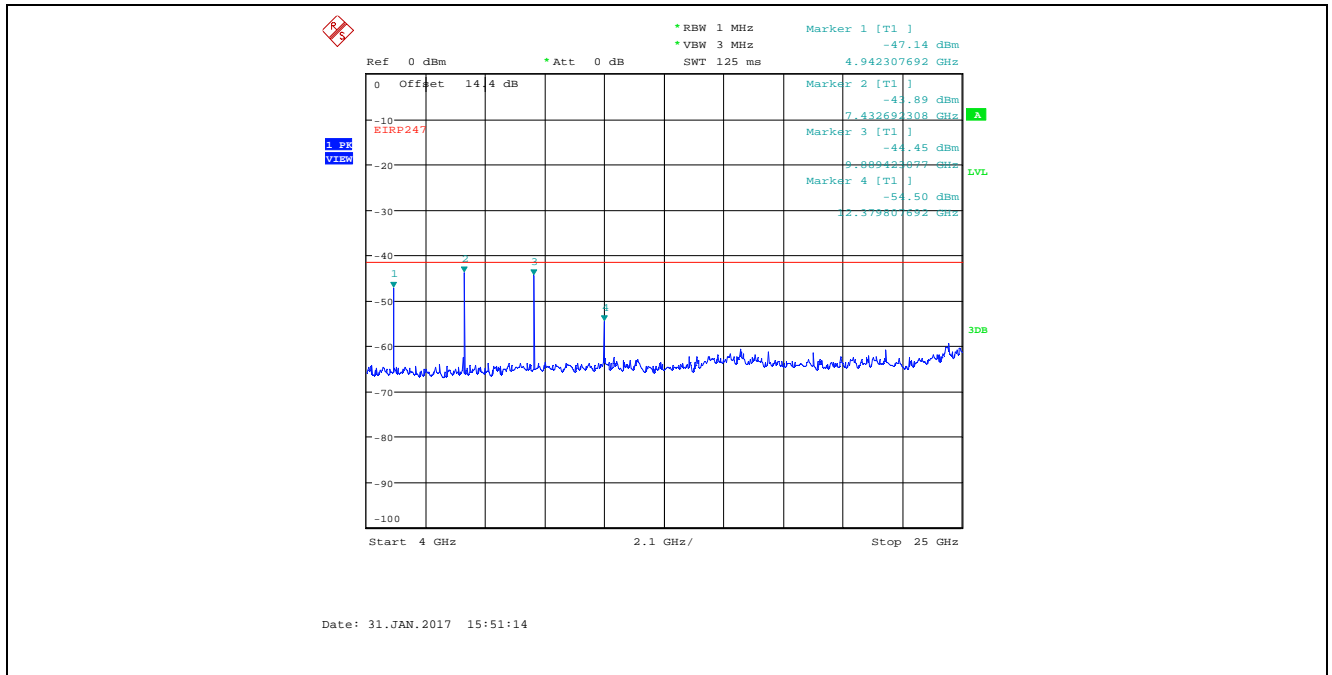
Plot 5.4.4.15. Conducted Spurious Emissions in Restricted Frequency Bands Bandwidth: 8 MHz, TX Gain Setting 25, Data Rate 1, 2477 MHz, 4 GHz - 25 GHz, Peak Detector
