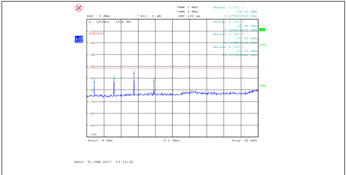
Plot 5.4.4.29. Conducted Spurious Emissions in Restricted Frequency Bands Bandwidth: 8 MHz, TX Gain Setting 25, Data Rate 4, 2442 MHz, 4 GHz - 25 GHz, Peak Detector
