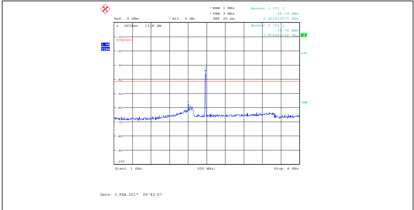
Plot 5.4.4.3.29. Conducted Spurious Emissions in Restricted Frequency Bands Bandwidth: 8 MHz, TX Gain Setting 55, Data Rate 4, 2477 MHz, 1 GHz - 4 GHz, Peak Detector Marker 2 is the Fundamental
