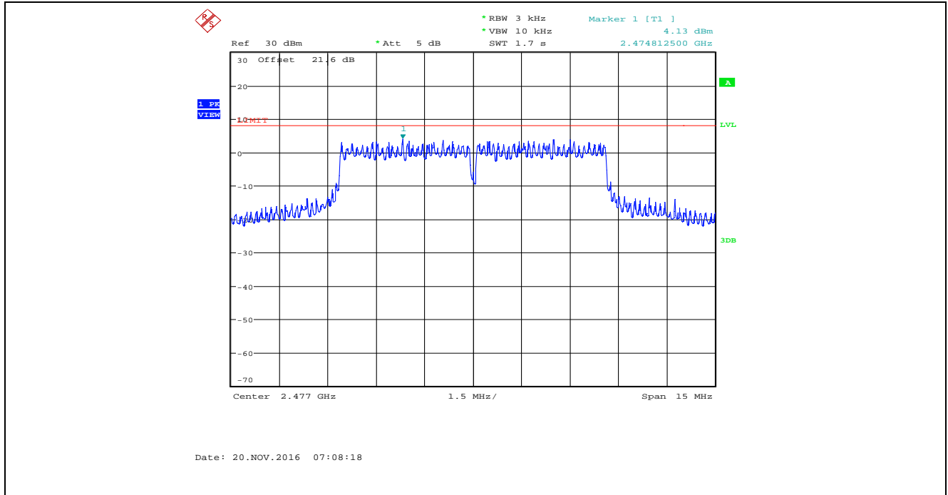
Plot 5.6.4.72. Power Spectral Density, Bandwidth: 8 MHz, TX Gain Setting: 55, Data Rate 4, 2477 MHz
