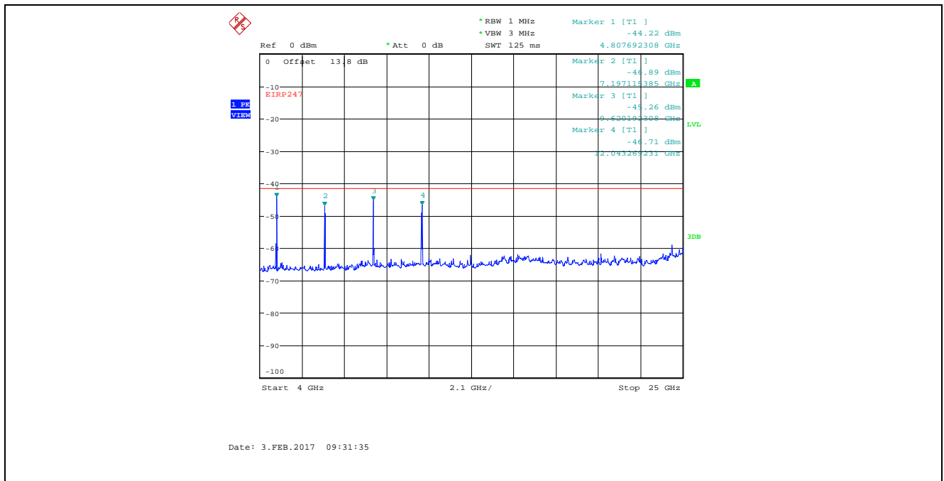
Plot 5.4.4.3.20. Conducted Spurious Emissions in Restricted Frequency Bands Bandwidth: 8 MHz, TX Gain Setting 55, Data Rate 4, 2407 MHz, 4 GHz - 25 GHz, Peak Detector
