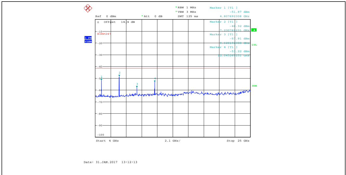
Plot 5.4.4.22. Conducted Spurious Emissions in Restricted Frequency Bands Bandwidth: 8 MHz, TX Gain Setting 25, Data Rate 4, 2407 MHz, 4 GHz - 25 GHz, Peak Detector
