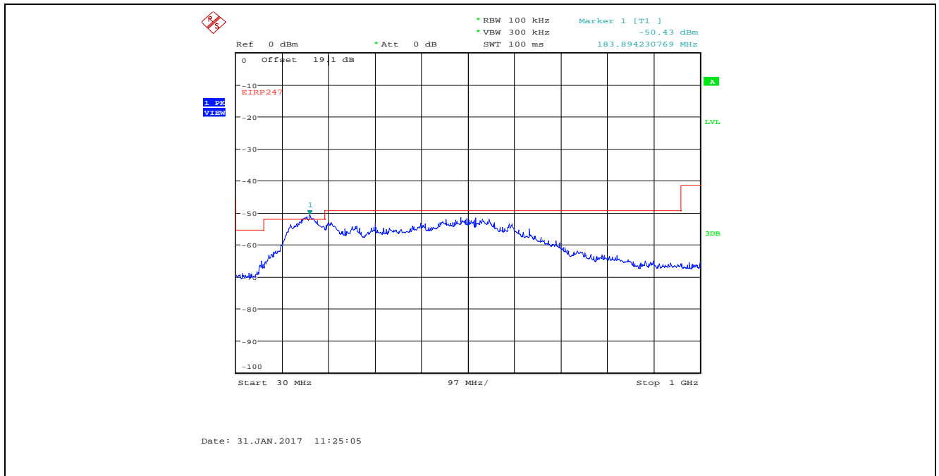
Plot 5.4.4.32. Conducted Spurious Emissions in Restricted Frequency Bands Bandwidth: 8 MHz, TX Gain Setting 25, Data Rate 4, 2477 MHz, 30 MHz - 1 GHz, Peak Detector
