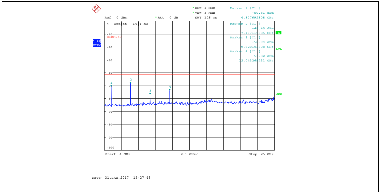
Plot 5.4.4.4.5. Conducted Spurious Emissions in Restricted Frequency Bands Bandwidth: 8 MHz, TX Gain Setting 25, Data Rate 1, 2407 MHz, 4 GHz - 25 GHz, Peak Detector
