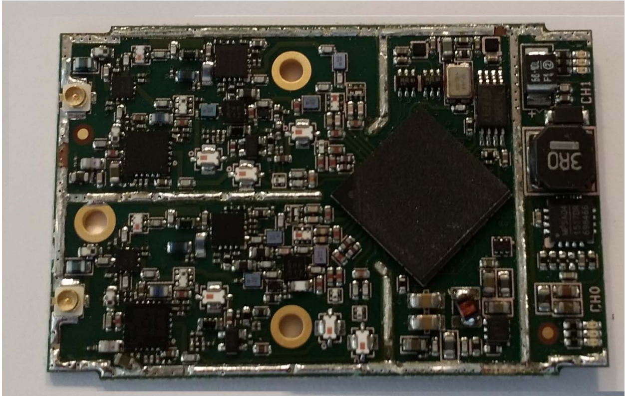
Top No Shield
