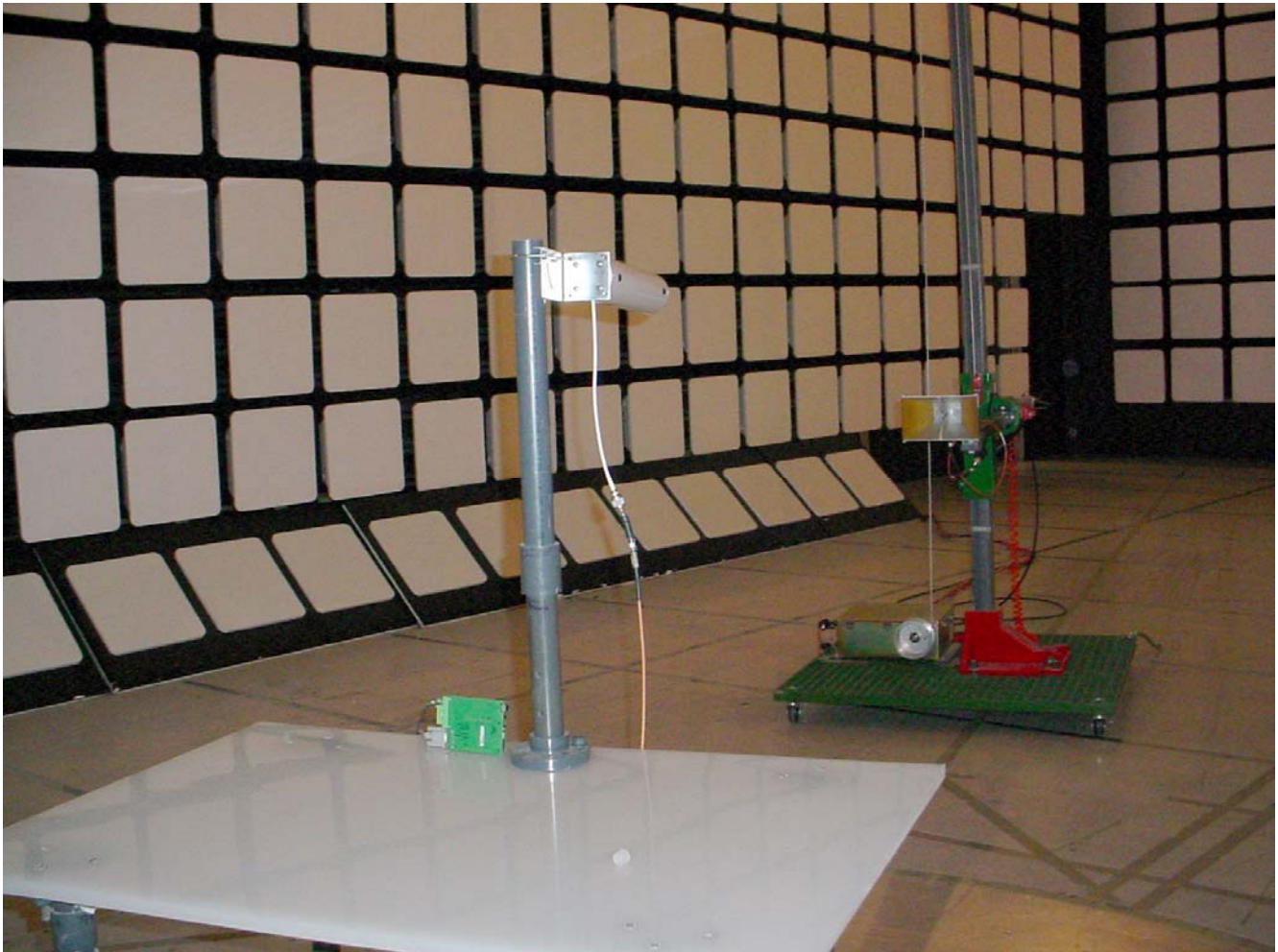
Radiated Emissions @ 3 Meters EUT with 14.5 dBi Yagi Antenna
