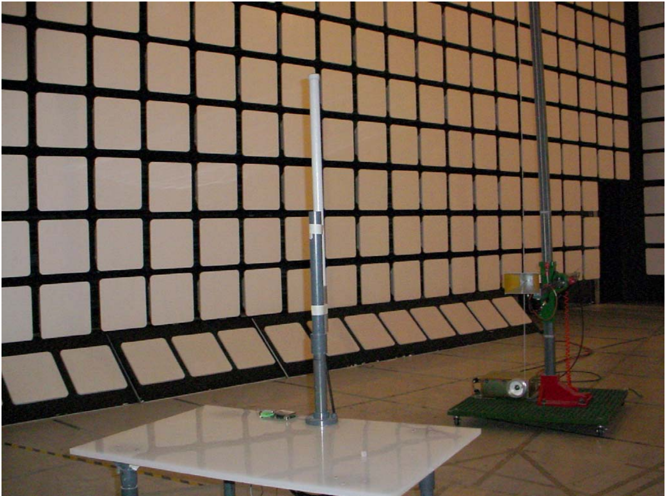
Radiated Emissions @ 3 Meters EUT with 15 dBi Omni Directional Antenna
