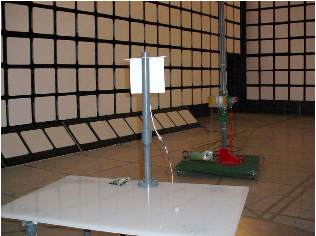
Radiated Emissions @ 3 Meters EUT with 14 dBi Patch Antenna
