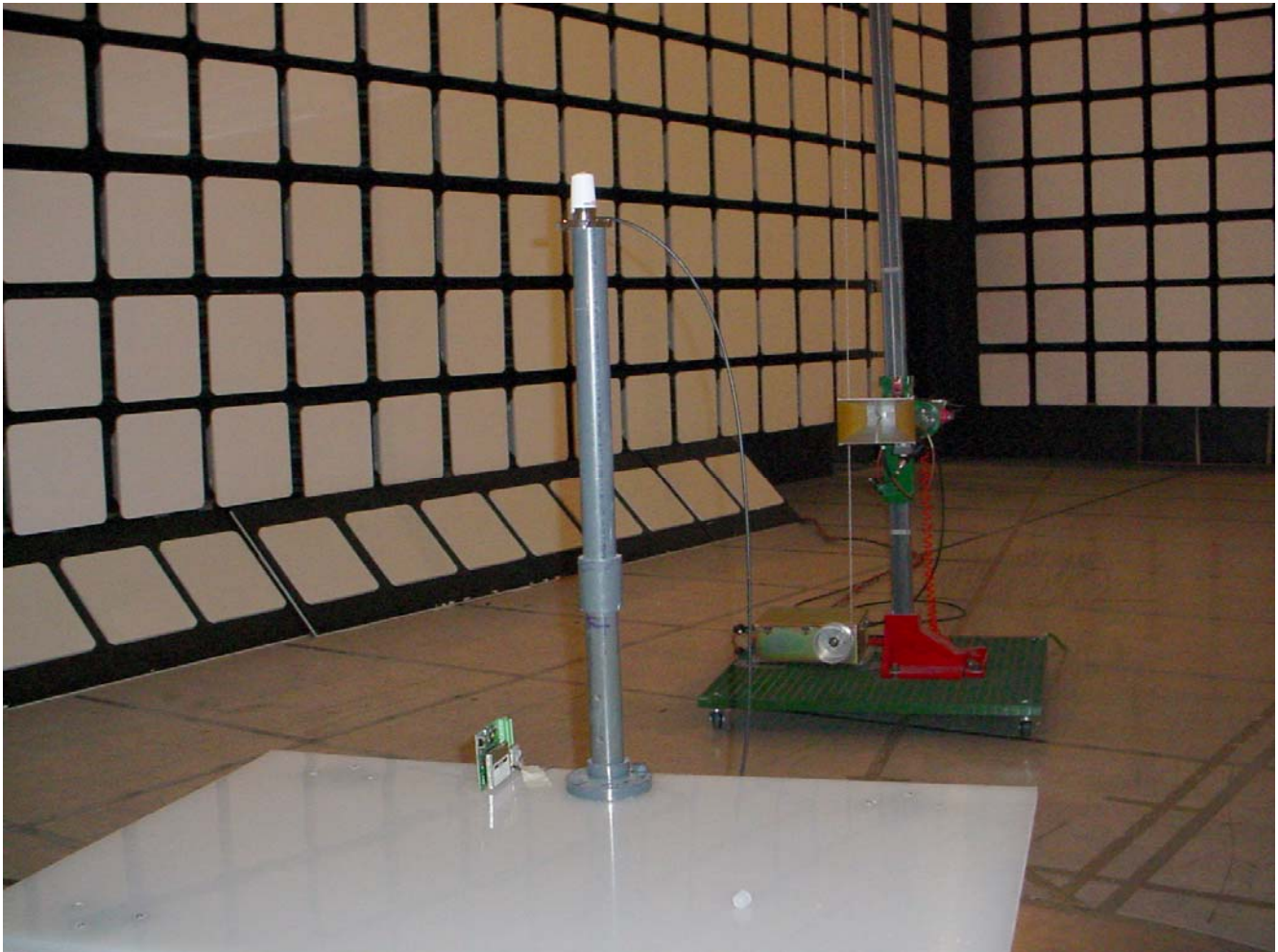
Radiated Emissions @ 3 Meters EUT with 3 dBi Transit Antenna
